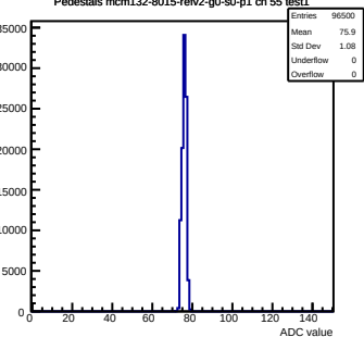
Pedestals mcm132-8015-refv2-g0-s0-p1 ch 55 test1
