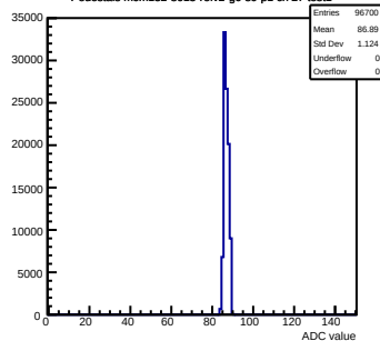
Pedestals mcm132-8015-refv2-g0-s0-p1 ch 27 test1
