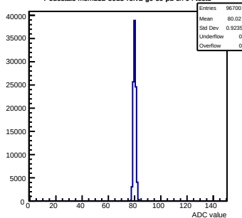
Pedestals mcm132-8015-refv2-g0-s0-p1 ch 94 test1
