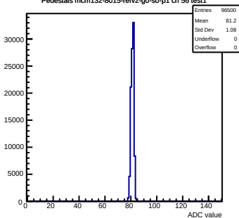
Pedestals mcm132-8015-refv2-g0-s0-p1 ch 56 test1
