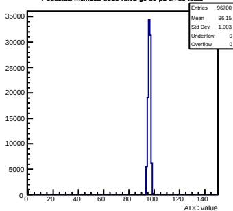
Pedestals mcm132-8015-refv2-g0-s0-p1 ch 89 test1
