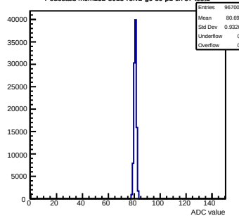
Pedestals mcm132-8015-refv2-g0-s0-p1 ch 87 test1
