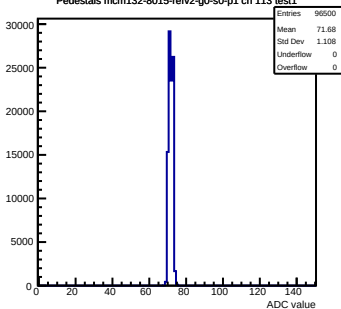
Pedestals mcm132-8015-refv2-g0-s0-p1 ch 113 test1
