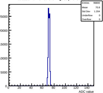
Pedestals mcm132-8015-refv2-g0-s0-p1 ch 5 test1
