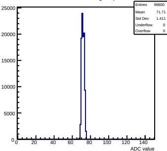
Pedestals mcm132-8015-refv2-g0-s0-p1 ch 8 test1
