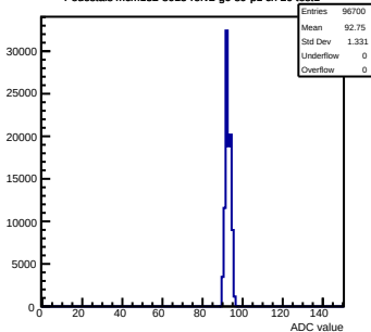
Pedestals mcm132-8015-refv2-g0-s0-p1 ch 20 test1
