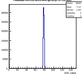
Pedestals mcm132-8015-refv2-g0-s0-p1 ch 114 test1
