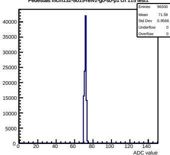
Pedestals mcm132-8015-refv2-g0-s0-p1 ch 115 test1
