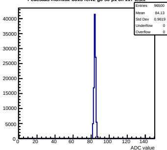
Pedestals mcm132-8015-refv2-g0-s0-p1 ch 117 test1
