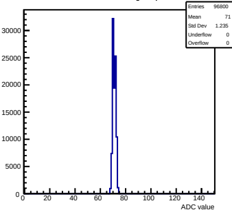
Pedestals mcm132-8015-refv2-g0-s0-p1 ch 11 test1
