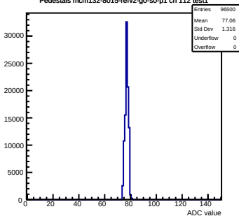
Pedestals mcm132-8015-refv2-g0-s0-p1 ch 112 test1
