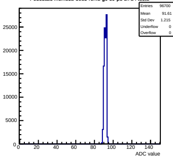
Pedestals mcm132-8015-refv2-g0-s0-p1 ch 24 test1
