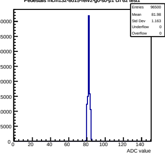
Pedestals mcm132-8015-refv2-g0-s0-p1 ch 62 test1
