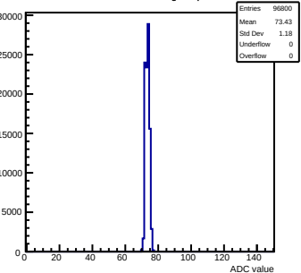
Pedestals mcm132-8015-refv2-g0-s0-p1 ch 13 test1
