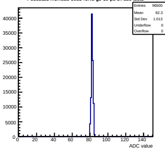
Pedestals mcm132-8015-refv2-g0-s0-p1 ch 120 test1
