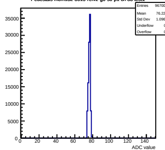
Pedestals mcm132-8015-refv2-g0-s0-p1 ch 83 test1
