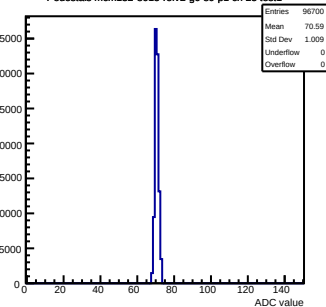
Pedestals mcm132-8015-refv2-g0-s0-p1 ch 25 test1
