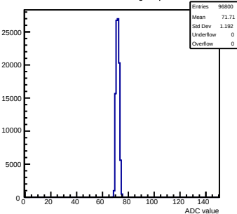
Pedestals mcm132-8015-refv2-g0-s0-p1 ch 15 test1
