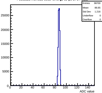
Pedestals mcm132-8015-refv2-g0-s0-p1 ch 84 test1
