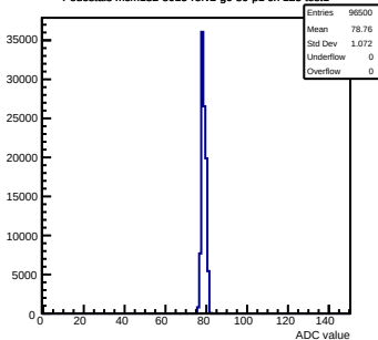
Pedestals mcm132-8015-refv2-g0-s0-p1 ch 125 test1
