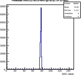
Pedestals mcm132-8015-refv2-g0-s0-p1 ch 53 test1
