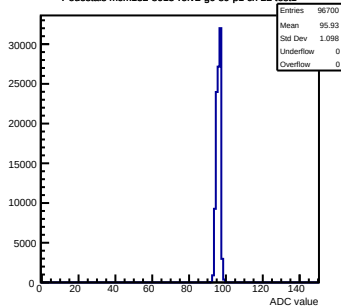
Pedestals mcm132-8015-refv2-g0-s0-p1 ch 22 test1
