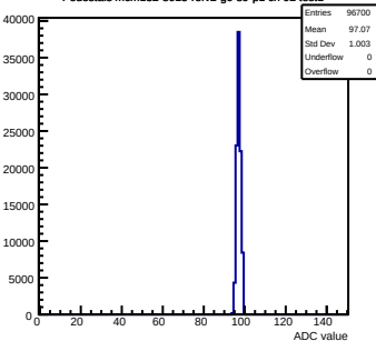
Pedestals mcm132-8015-refv2-g0-s0-p1 ch 92 test1
