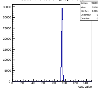
Pedestals mcm132-8015-refv2-g0-s0-p1 ch 23 test1
