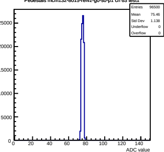
Pedestals mcm132-8015-refv2-g0-s0-p1 ch 63 test1
