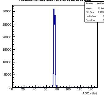
Pedestals mcm132-8015-refv2-g0-s0-p1 ch 82 test1
