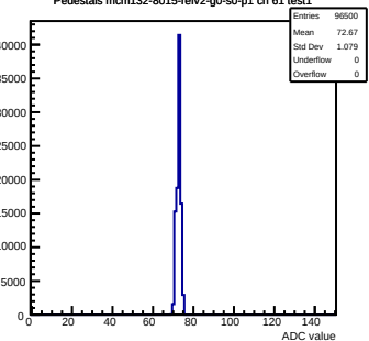
Pedestals mcm132-8015-refv2-g0-s0-p1 ch 61 test1
