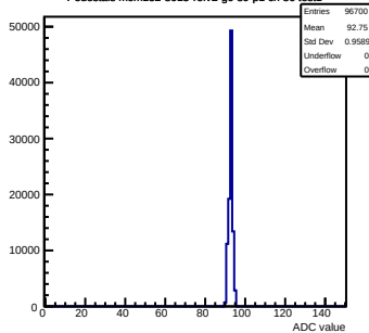
Pedestals mcm132-8015-refv2-g0-s0-p1 ch 86 test1
