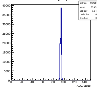
Pedestals mcm132-8015-refv2-g0-s0-p1 ch 30 test1
