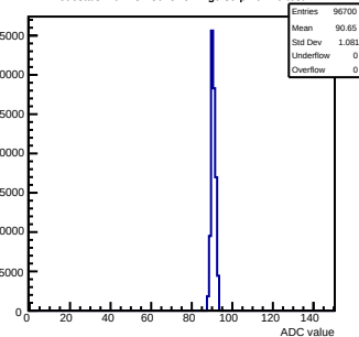
Pedestals mcm132-8015-refv2-g0-s0-p1 ch 29 test1
