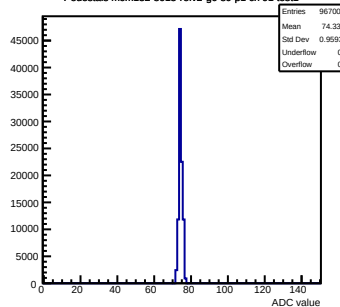
Pedestals mcm132-8015-refv2-g0-s0-p1 ch 91 test1
