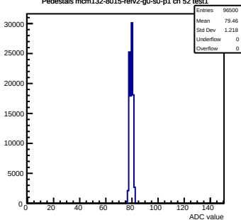
Pedestals mcm132-8015-refv2-g0-s0-p1 ch 52 test1
