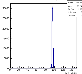
Pedestals mcm132-8015-refv2-g0-s0-p1 ch 31 test1
