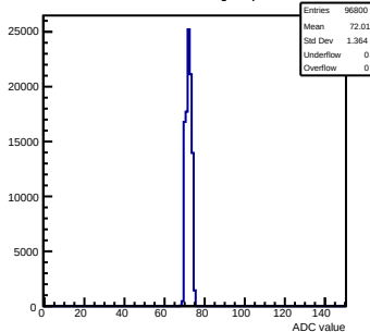
Pedestals mcm132-8015-refv2-g0-s0-p1 ch 10 test1
