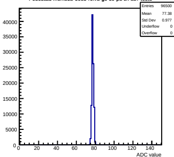
Pedestals mcm132-8015-refv2-g0-s0-p1 ch 127 test1
