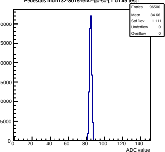
Pedestals mcm132-8015-refv2-g0-s0-p1 ch 49 test1
