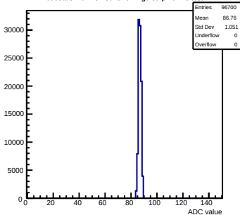
Pedestals mcm132-8015-refv2-g0-s0-p1 ch 28 test1
