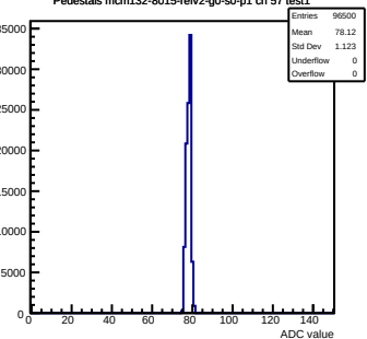
Pedestals mcm132-8015-refv2-g0-s0-p1 ch 57 test1
