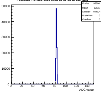
Pedestals mcm132-8015-refv2-g0-s0-p1 ch 119 test1
