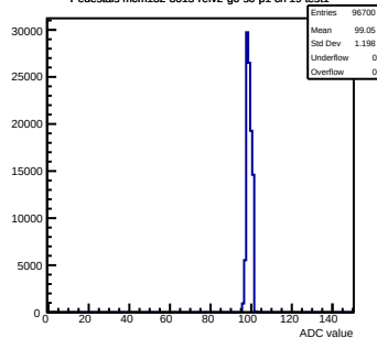
Pedestals mcm132-8015-refv2-g0-s0-p1 ch 19 test1
