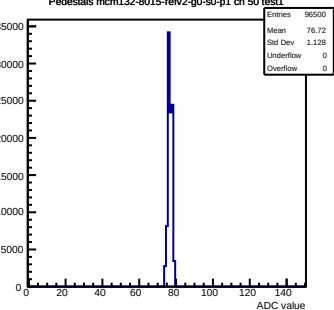
Pedestals mcm132-8015-refv2-g0-s0-p1 ch 50 test1
