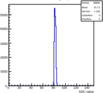
Pedestals mcm132-8015-refv2-g0-s0-p1 ch 9 test1
