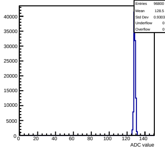
Pedestals mcm132-8015-rlv6-g0-s0-p1 ch 13 test1
