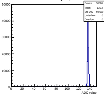
Pedestals mcm132-8015-refv6-g0-s0-p1 ch 109 test1
