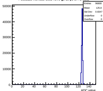
Pedestals mcm132-8015-relv6-g0-s0-p1 ch 75 test1
