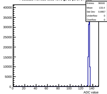
Pedestals mcm132-8015-relv6-g0-s0-p1 ch 54 test1
