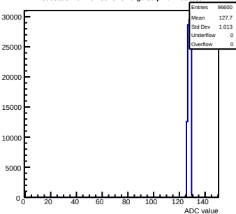
Pedestals mcm132-8015-refv6-g0-s0-p1 ch 108 test1
