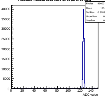
Pedestals mcm132-8015-relv6-g0-s0-p1 ch 39 test1
