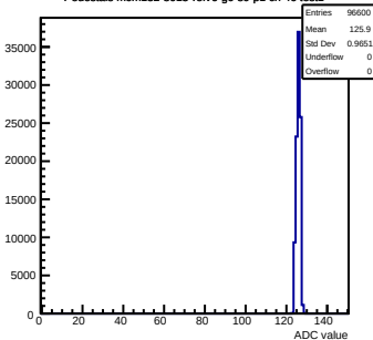
Pedestals mcm132-8015-relv6-g0-s0-p1 ch 46 test1
