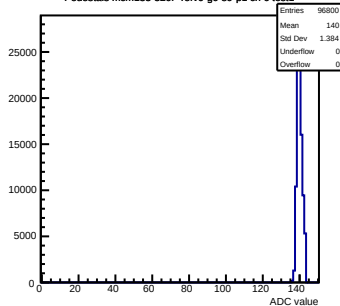
Pedestals mcm133-320F-refV0-g0-s0-p1 ch 6 test1
