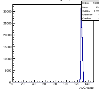
Pedestals mcm133-320F-refV0-g0-s0-p1 ch 15 test1
