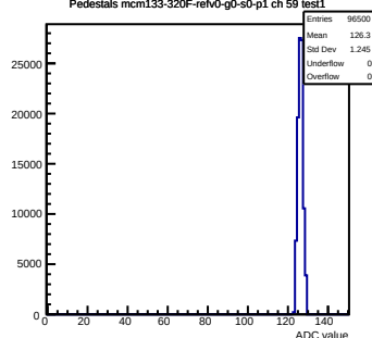
Pedestals mcm133-320F-refV0-g0-s0-p1 ch 59 test1
