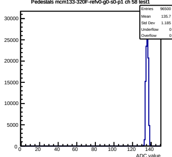
Pedestals mcm133-320F-refV0-g0-s0-p1 ch 58 test1
