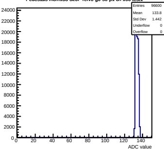
Pedestals mcm133-320F-refV0-g0-s0-p1 ch 100 test1
