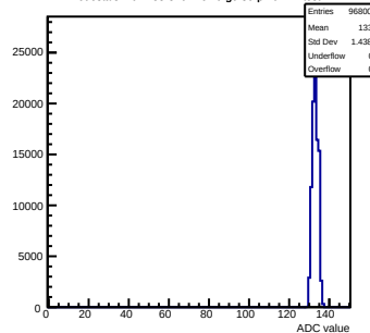
Pedestals mcm133-320F-refV0-g0-s0-p1 ch 11 test1
