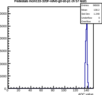
Pedestals mcm133-320F-refV0-g0-s0-p1 ch 57 test1
