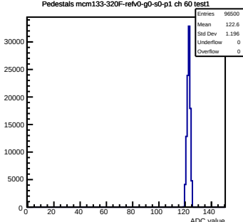
Pedestals mcm133-320F-refV0-g0-s0-p1 ch 60 test1
