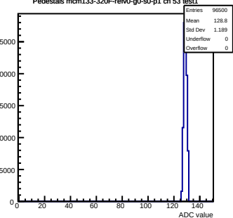
Pedestals mcm133-320F-refV0-g0-s0-p1 ch 53 test1
