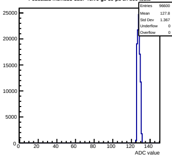
Pedestals mcm133-320F-refV0-g0-s0-p1 ch 109 test1
