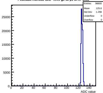
Pedestals mcm133-320F-refV0-g0-s0-p1 ch 97 test1
