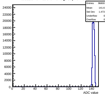
Pedestals mcm133-320F-refV0-g0-s0-p1 ch 10 test1
