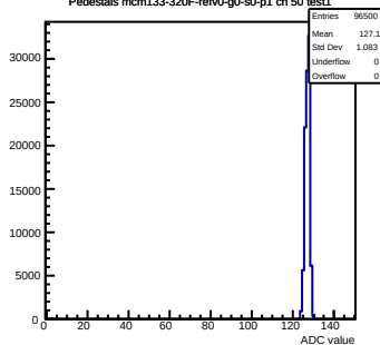
Pedestals mcm133-320F-refV0-g0-s0-p1 ch 50 test1
