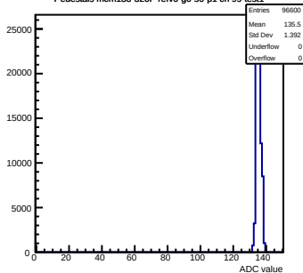
Pedestals mcm133-320F-refV0-g0-s0-p1 ch 99 test1
