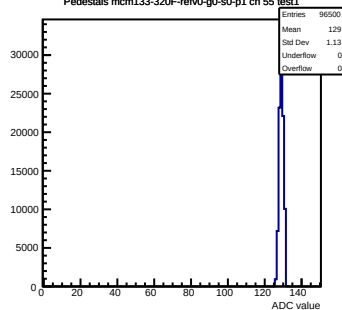
Pedestals mcm133-320F-refV0-g0-s0-p1 ch 55 test1
