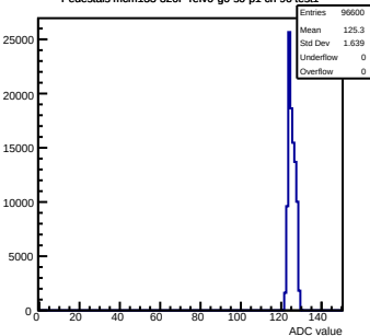
Pedestals mcm133-320F-refV0-g0-s0-p1 ch 96 test1
