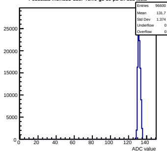
Pedestals mcm133-320F-refV0-g0-s0-p1 ch 111 test1
