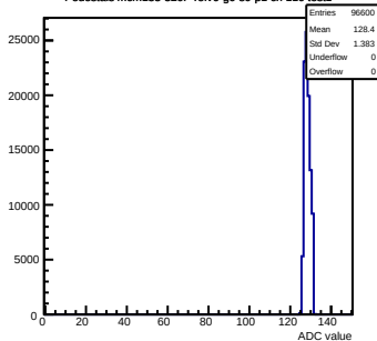
Pedestals mcm133-320F-refV0-g0-s0-p1 ch 110 test1
