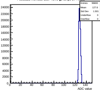
Pedestals mcm133-320F-refV0-g0-s0-p1 ch 4 test1
