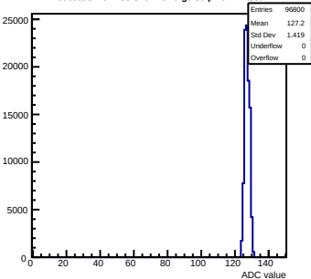
Pedestals mcm133-320F-refV0-g0-s0-p1 ch 12 test1
