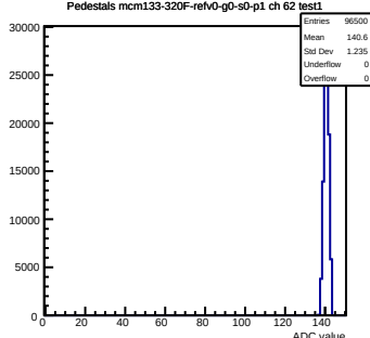
Pedestals mcm133-320F-refV0-g0-s0-p1 ch 62 test1
