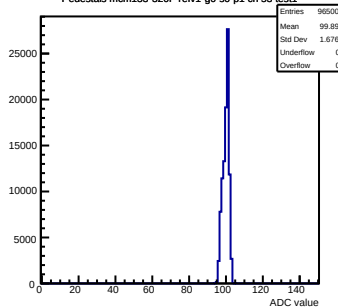
Pedestals mcm133-320F-refv1-g0-s0-p1 ch 53 test1
