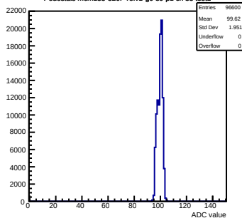
Pedestals mcm133-320F-refv1-g0-s0-p1 ch 33 test1
