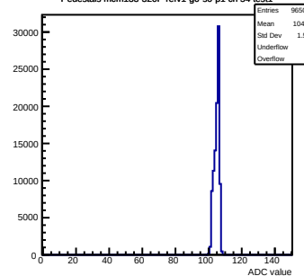
Pedestals mcm133-320F-refv1-g0-s0-p1 ch 54 test1
