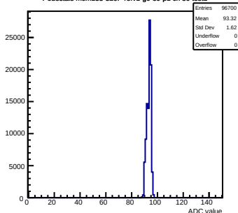
Pedestals mcm133-320F-refv1-g0-s0-p1 ch 30 test1
