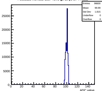
Pedestals mcm133-320F-refv1-g0-s0-p1 ch 44 test1
