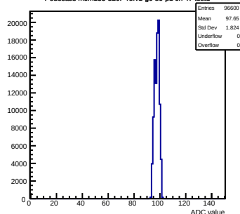
Pedestals mcm133-320F-refv1-g0-s0-p1 ch 47 test1
