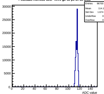
Pedestals mcm133-320F-refv1-g0-s0-p1 ch 18 test1
