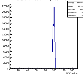
Pedestals mcm133-320F-refv1-g0-s0-p1 ch 46 test1
