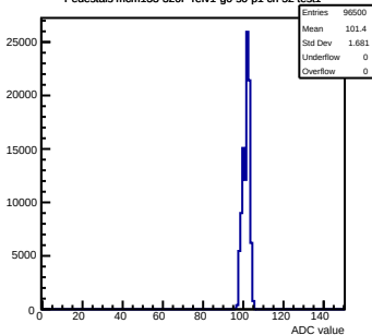
Pedestals mcm133-320F-refv1-g0-s0-p1 ch 52 test1
