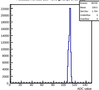
Pedestals mcm133-320F-refv1-g0-s0-p1 ch 20 test1
