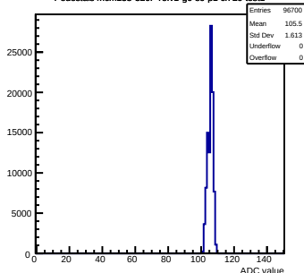
Pedestals mcm133-320F-refv1-g0-s0-p1 ch 29 test1
