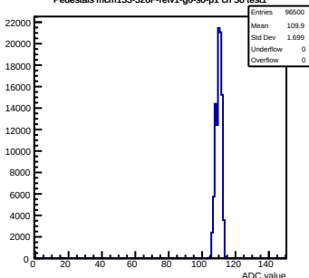
Pedestals mcm133-320F-refv1-g0-s0-p1 ch 56 test1
