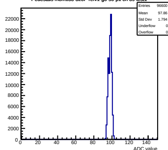
Pedestals mcm133-320F-refv1-g0-s0-p1 ch 39 test1
