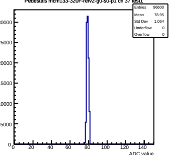
Pedestals mcm133-320F-refv2-g0-s0-p1 ch 37 test1
