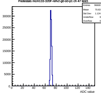
Pedestals mcm133-320F-refv2-g0-s0-p1 ch 47 test1
