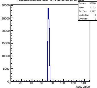
Pedestals mcm133-320F-refv2-g0-s0-p1 ch 68 test1
