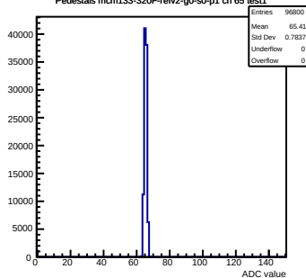
Pedestals mcm133-320F-refv2-g0-s0-p1 ch 65 test1
