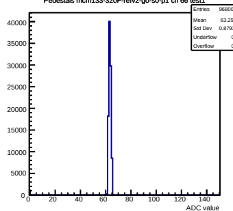
Pedestals mcm133-320F-refv2-g0-s0-p1 ch 66 test1
