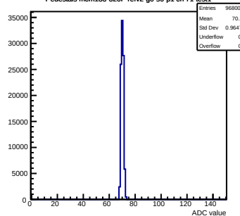
Pedestals mcm133-320F-refv2-g0-s0-p1 ch 71 test1
