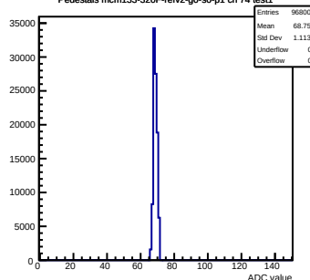
Pedestals mcm133-320F-refv2-g0-s0-p1 ch 74 test1
