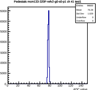
Pedestals mcm133-320F-refv2-g0-s0-p1 ch 41 test1
