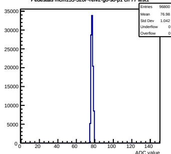
Pedestals mcm133-320F-refv2-g0-s0-p1 ch 77 test1
