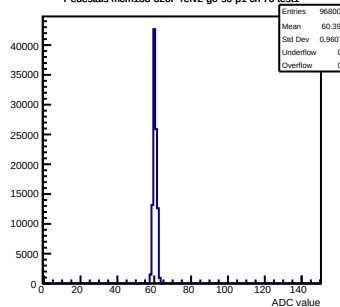
Pedestals mcm133-320F-refv2-g0-s0-p1 ch 70 test1
