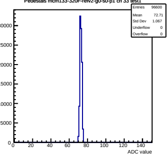
Pedestals mcm133-320F-refv2-g0-s0-p1 ch 33 test1
