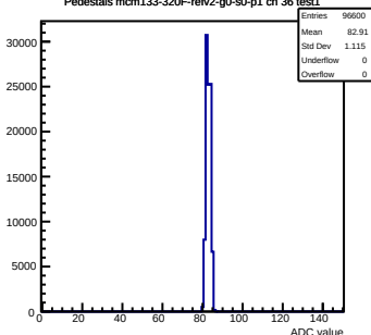
Pedestals mcm133-320F-refv2-g0-s0-p1 ch 36 test1
