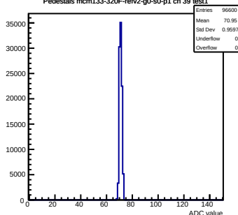
Pedestals mcm133-320F-refv2-g0-s0-p1 ch 39 test1
