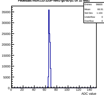
Pedestals mcm133-320F-refv2-g0-s0-p1 ch 32 test1
