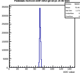
Pedestals mcm133-320F-refv2-g0-s0-p1 ch 46 test1
