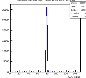
Pedestals mcm133-320F-refv2-g0-s0-p1 ch 69 test1
