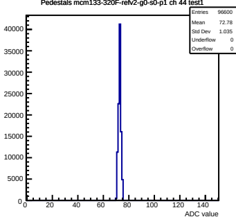
Pedestals mcm133-320F-refv2-g0-s0-p1 ch 44 test1
