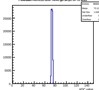
Pedestals mcm133-320F-refv2-g0-s0-p1 ch 78 test1
