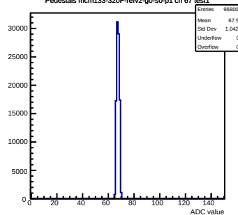
Pedestals mcm133-320F-refv2-g0-s0-p1 ch 67 test1
