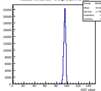
Pedestals mcm133-320F-refV5-g0-s0-p1 ch 63 test1
