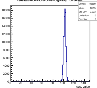
Pedestals mcm133-320F-refv5-g0-s0-p1 ch 36 test1
