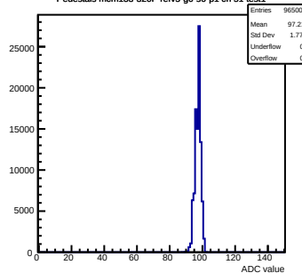
Pedestals mcm133-320F-refV5-g0-s0-p1 ch 51 test1
