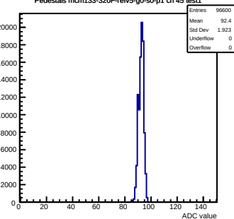
Pedestals mcm133-320F-refv5-g0-s0-p1 ch 45 test1
