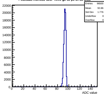
Pedestals mcm133-320F-refV5-g0-s0-p1 ch 53 test1
