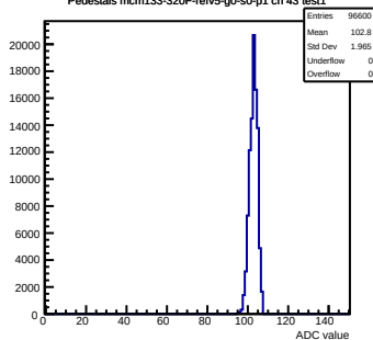
Pedestals mcm133-320F-refv5-g0-s0-p1 ch 43 test1
