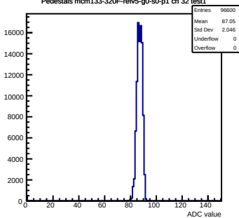
Pedestals mcm133-320F-refv5-g0-s0-p1 ch 32 test1
