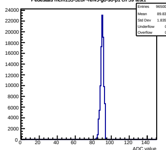
Pedestals mcm133-320F-refV5-g0-s0-p1 ch 59 test1
