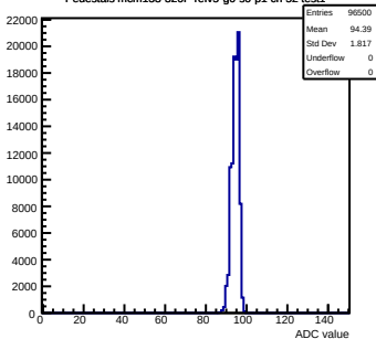
Pedestals mcm133-320F-refV5-g0-s0-p1 ch 52 test1
