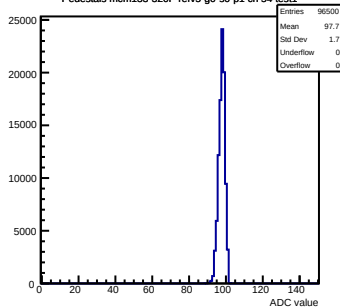
Pedestals mcm133-320F-refV5-g0-s0-p1 ch 54 test1
