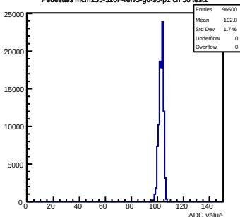
Pedestals mcm133-320F-refV5-g0-s0-p1 ch 56 test1
