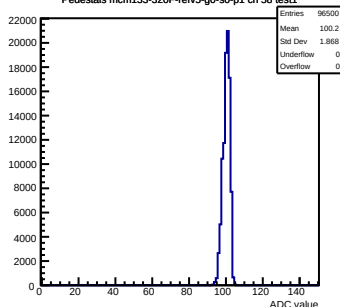
Pedestals mcm133-320F-refV5-g0-s0-p1 ch 58 test1
