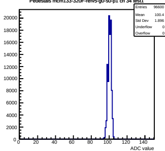
Pedestals mcm133-320F-refv5-g0-s0-p1 ch 34 test1
