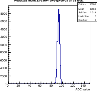
Pedestals mcm133-320F-refv5-g0-s0-p1 ch 33 test1
