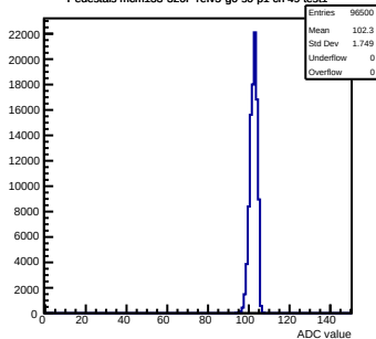
Pedestals mcm133-320F-refV5-g0-s0-p1 ch 49 test1
