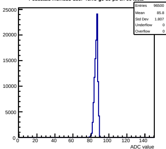
Pedestals mcm133-320F-refV5-g0-s0-p1 ch 60 test1
