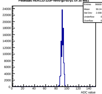
Pedestals mcm133-320F-refv5-g0-s0-p1 ch 35 test1
