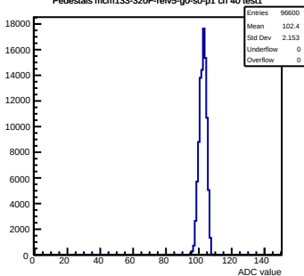
Pedestals mcm133-320F-refv5-g0-s0-p1 ch 40 test1
