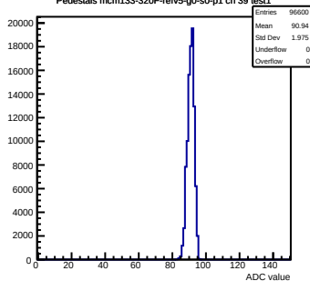
Pedestals mcm133-320F-refv5-g0-s0-p1 ch 39 test1
