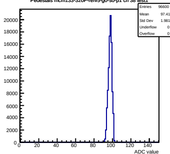
Pedestals mcm133-320F-refv5-g0-s0-p1 ch 38 test1
