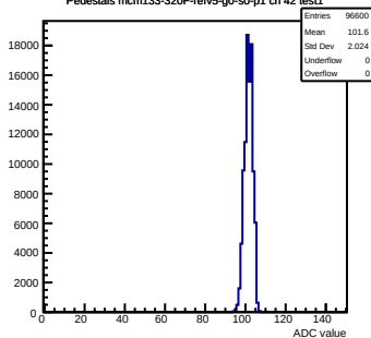
Pedestals mcm133-320F-refv5-g0-s0-p1 ch 42 test1
