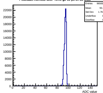
Pedestals mcm133-320F-refV5-g0-s0-p1 ch 55 test1
