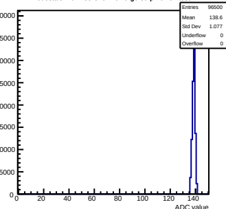
Pedestals mcm133-320F-refv6-g0-s0-p1 ch 57 test1
