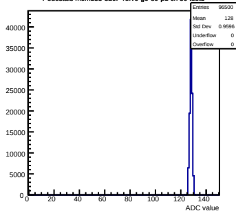
Pedestals mcm133-320F-refv6-g0-s0-p1 ch 50 test1
