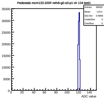
Pedestals mcm133-320F-refv6-g0-s0-p1 ch 124 test1
