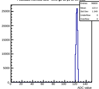
Pedestals mcm133-320F-refv6-g0-s0-p1 ch 64 test1
