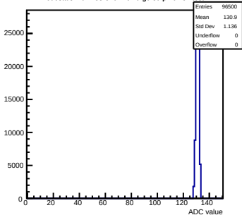
Pedestals mcm133-320F-refv6-g0-s0-p1 ch 52 test1
