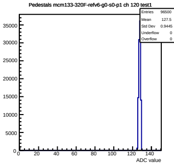
Pedestals mcm133-320F-refv6-g0-s0-p1 ch 120 test1
