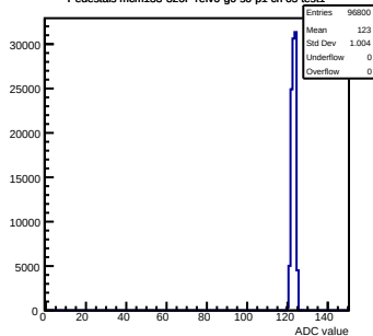
Pedestals mcm133-320F-refv6-g0-s0-p1 ch 65 test1
