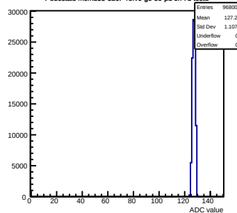
Pedestals mcm133-320F-refv6-g0-s0-p1 ch 71 test1
