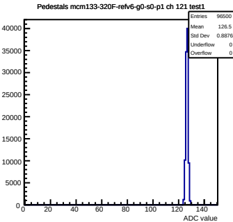
Pedestals mcm133-320F-refv6-g0-s0-p1 ch 121 test1
