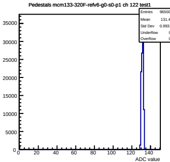
Pedestals mcm133-320F-refv6-g0-s0-p1 ch 122 test1
