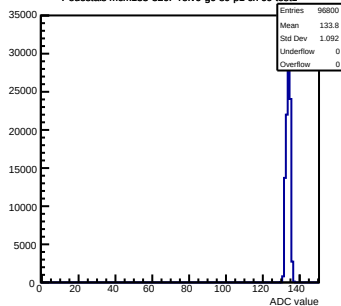
Pedestals mcm133-320F-refv6-g0-s0-p1 ch 69 test1
