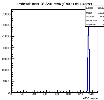
Pedestals mcm133-320F-refv6-g0-s0-p1 ch 114 test1
