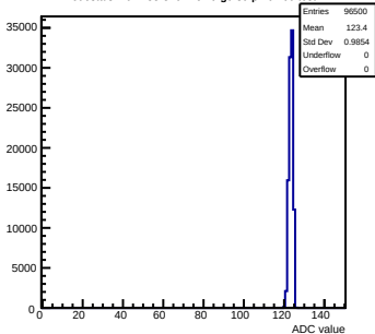
Pedestals mcm133-320F-refv6-g0-s0-p1 ch 60 test1
