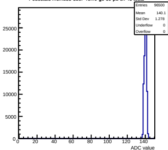
Pedestals mcm133-320F-refv6-g0-s0-p1 ch 48 test1
