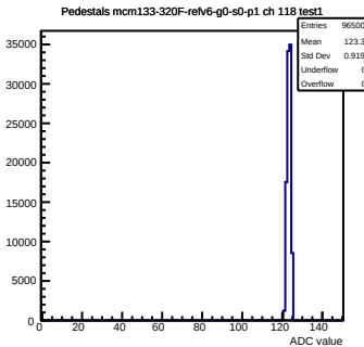
Pedestals mcm133-320F-refv6-g0-s0-p1 ch 118 test1
