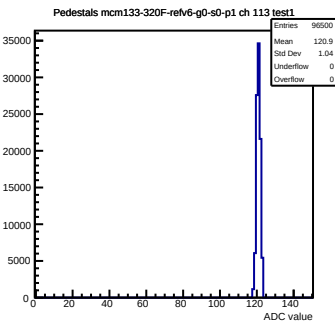
Pedestals mcm133-320F-refv6-g0-s0-p1 ch 113 test1
