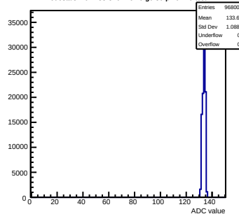
Pedestals mcm133-320F-refv6-g0-s0-p1 ch 79 test1
