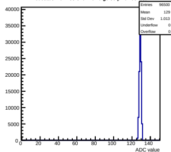
Pedestals mcm133-320F-refv6-g0-s0-p1 ch 55 test1
