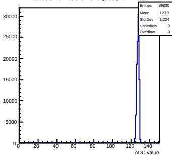
Pedestals mcm133-320F-refv6-g0-s0-p1 ch 72 test1
