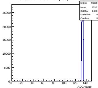
Pedestals mcm133-320F-refv6-g0-s0-p1 ch 77 test1
