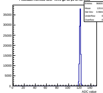
Pedestals mcm133-320F-refv6-g0-s0-p1 ch 66 test1
