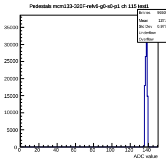
Pedestals mcm133-320F-refv6-g0-s0-p1 ch 115 test1
