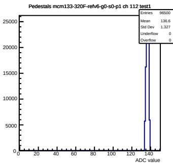
Pedestals mcm133-320F-refv6-g0-s0-p1 ch 112 test1
