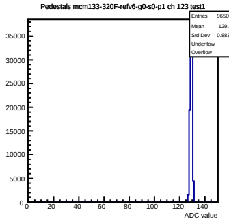
Pedestals mcm133-320F-refv6-g0-s0-p1 ch 123 test1
