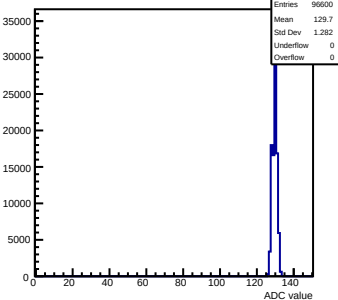
Pedestals mcm140-722E-refV0-g0-s0-p1 ch 40 test1
