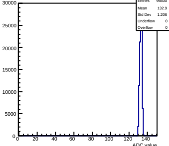
Pedestals mcm140-722E-refV0-g0-s0-p1 ch 37 test1
