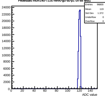
Pedestals mcm140-722E-refV0-g0-s0-p1 ch 68 test1
