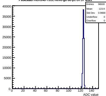
Pedestals mcm140-722E-refV0-g0-s0-p1 ch 57 test1
