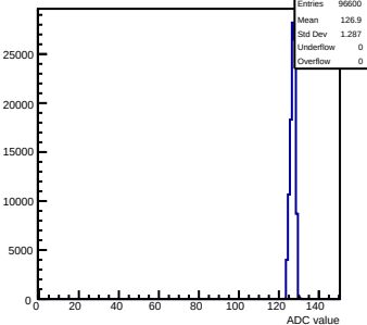
Pedestals mcm140-722E-refV0-g0-s0-p1 ch 44 test1
