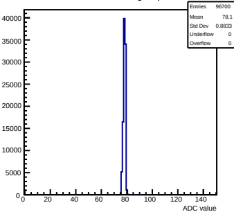
Pedestals mcm140-722E-refv2-g0-s0-p1 ch 92 test1
