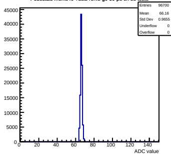
Pedestals mcm140-722E-refv2-g0-s0-p1 ch 81 test1
