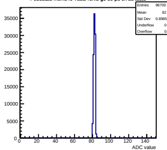
Pedestals mcm140-722E-ref2-g0-s0-p1 ch 22 test1
