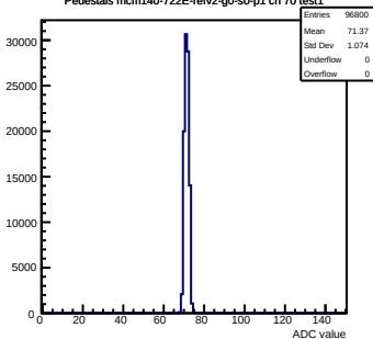
Pedestals mcm140-722E-refV2-g0-s0-p1 ch 70 test1
