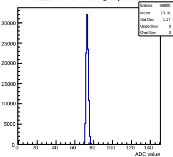
Pedestals mcm140-722E-refV2-g0-s0-p1 ch 8 test1
