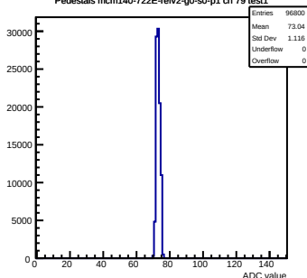
Pedestals mcm140-722E-refV2-g0-s0-p1 ch 79 test1
