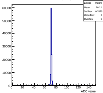
Pedestals mcm140-722E-refv2-g0-s0-p1 ch 93 test1
