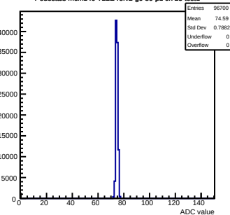
Pedestals mcm140-722E-ref2-g0-s0-p1 ch 25 test1
