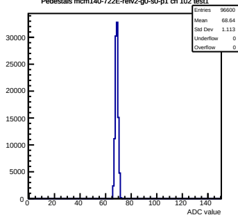
Pedestals mcm140-722E-refv2-g0-s0-p1 ch 102 test1
