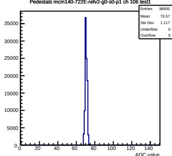
Pedestals mcm140-722E-refv2-g0-s0-p1 ch 106 test1
