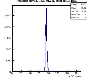
Pedestals mcm140-722E-refv2-g0-s0-p1 ch 104 test1
