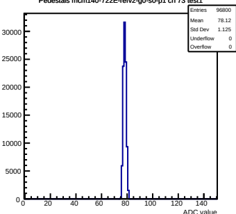
Pedestals mcm140-722E-refV2-g0-s0-p1 ch 73 test1
