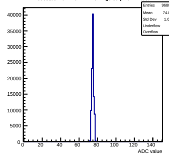
Pedestals mcm140-722E-refV2-g0-s0-p1 ch 11 test1
