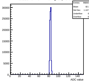
Pedestals mcm140-722E-refV2-g0-s0-p1 ch 9 test1
