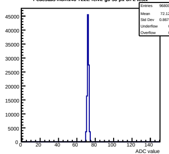
Pedestals mcm140-722E-refV2-g0-s0-p1 ch 2 test1
