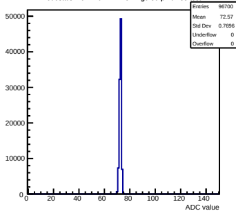
Pedestals mcm140-722E-refv2-g0-s0-p1 ch 85 test1
