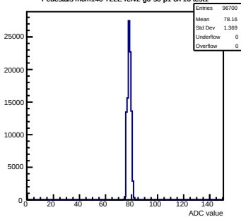
Pedestals mcm140-722E-ref2-g0-s0-p1 ch 16 test1
