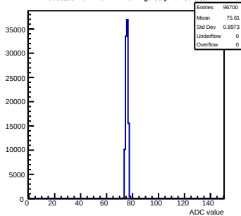
Pedestals mcm140-722E-refv2-g0-s0-p1 ch 89 test1
