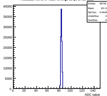
Pedestals mcm140-722E-ref2-g0-s0-p1 ch 31 test1
