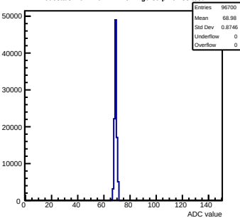
Pedestals mcm140-722E-refv2-g0-s0-p1 ch 88 test1
