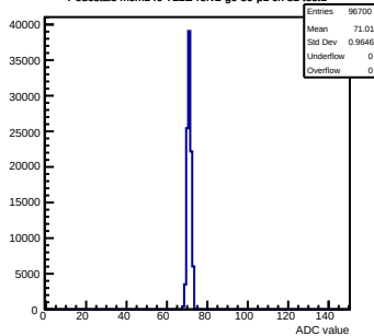
Pedestals mcm140-722E-refv2-g0-s0-p1 ch 82 test1
