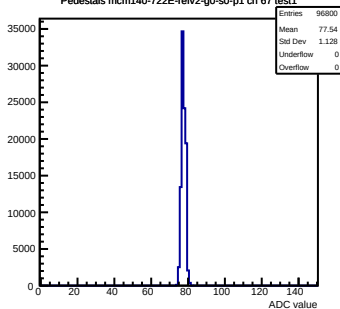
Pedestals mcm140-722E-refV2-g0-s0-p1 ch 67 test1
