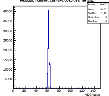
Pedestals mcm140-722E-refv2-g0-s0-p1 ch 99 test1
