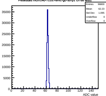
Pedestals mcm140-722E-refV2-g0-s0-p1 ch 68 test1
