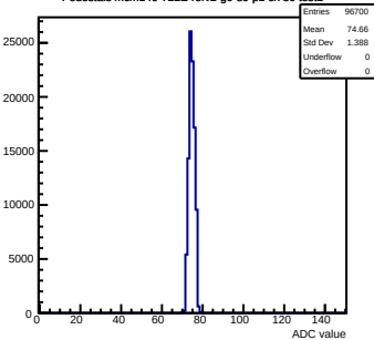
Pedestals mcm140-722E-g0-s0-p1 ch 80 test1
