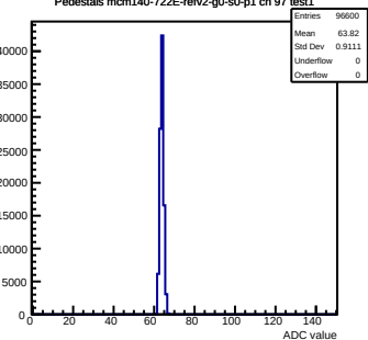
Pedestals mcm140-722E-refv2-g0-s0-p1 ch 97 test1
