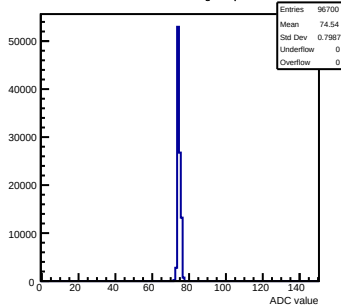
Pedestals mcm140-722E-refv2-g0-s0-p1 ch 94 test1
