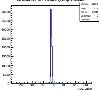
Pedestals mcm140-722E-refV2-g0-s0-p1 ch 66 test1
