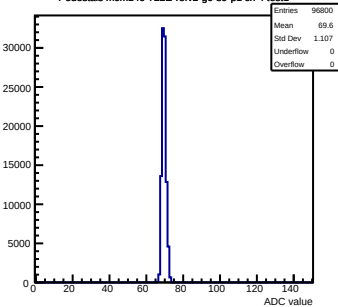
Pedestals mcm140-722E-refV2-g0-s0-p1 ch 4 test1
