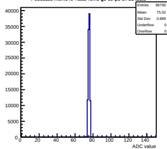
Pedestals mcm140-722E-ref2-g0-s0-p1 ch 23 test1
