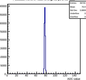
Pedestals mcm140-722E-ref2-g0-s0-p1 ch 29 test1
