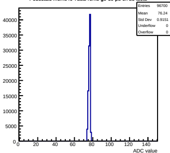
Pedestals mcm140-722E-ref2-g0-s0-p1 ch 28 test1
