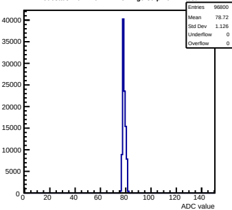
Pedestals mcm140-722E-refV2-g0-s0-p1 ch 12 test1
