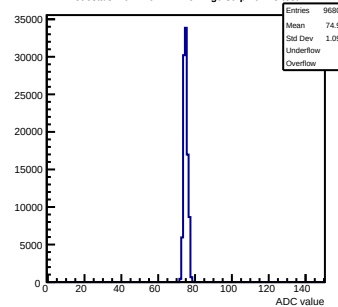
Pedestals mcm140-722E-refV2-g0-s0-p1 ch 15 test1
