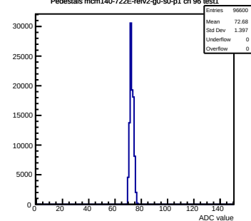
Pedestals mcm140-722E-refv2-g0-s0-p1 ch 96 test1
