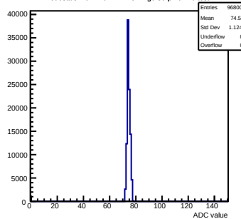
Pedestals mcm140-722E-refV2-g0-s0-p1 ch 10 test1
