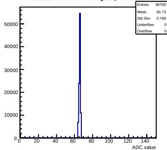
Pedestals mcm140-722E-refv2-g0-s0-p1 ch 86 test1
