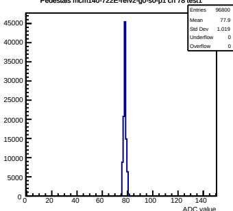
Pedestals mcm140-722E-refV2-g0-s0-p1 ch 78 test1
