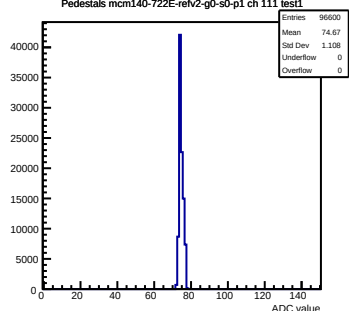
Pedestals mcm140-722E-refv2-g0-s0-p1 ch 111 test1
