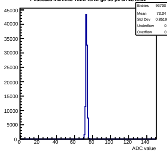
Pedestals mcm140-722E-ref2-g0-s0-p1 ch 18 test1
