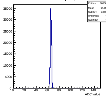
Pedestals mcm140-722E-refV2-g0-s0-p1 ch 14 test1
