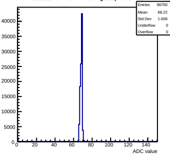
Pedestals mcm140-722E-refv2-g0-s0-p1 ch 84 test1
