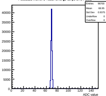
Pedestals mcm140-722E-ref2-g0-s0-p1 ch 24 test1
