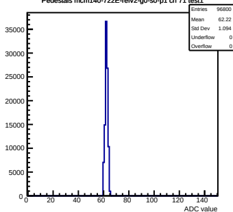
Pedestals mcm140-722E-refV2-g0-s0-p1 ch 71 test1
