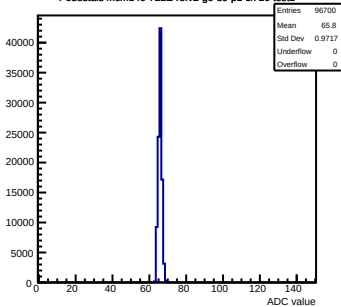
Pedestals mcm140-722E-ref2-g0-s0-p1 ch 20 test1
