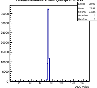
Pedestals mcm140-722E-refV2-g0-s0-p1 ch 65 test1
