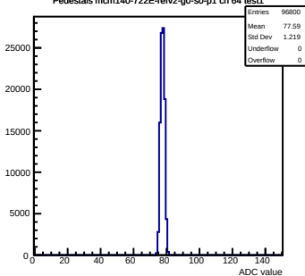
Pedestals mcm140-722E-refV2-g0-s0-p1 ch 64 test1
