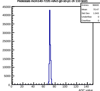
Pedestals mcm140-722E-refv2-g0-s0-p1 ch 110 test1
