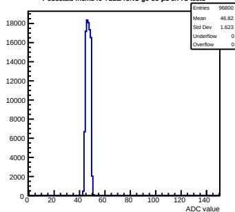
Pedestals mcm140-722E-refv3-g0-s0-p1 ch 73 test1
