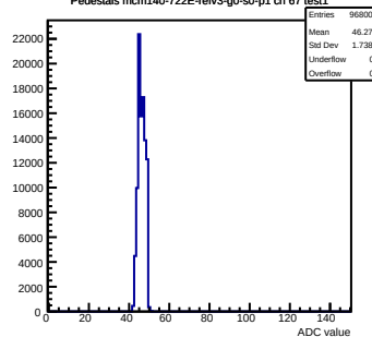
Pedestals mcm140-722E-refv3-g0-s0-p1 ch 67 test1
