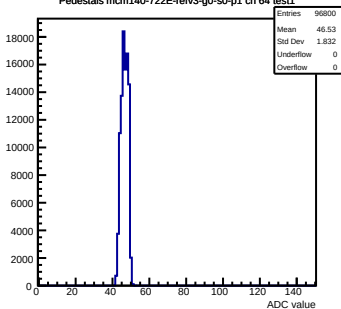
Pedestals mcm140-722E-refv3-g0-s0-p1 ch 64 test1
