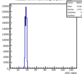
Pedestals mcm140-722E-refv3-g0-s0-p1 ch 77 test1
