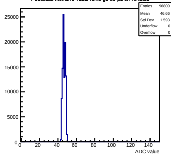
Pedestals mcm140-722E-refv3-g0-s0-p1 ch 78 test1
