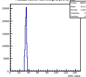
Pedestals mcm140-722E-refv3-g0-s0-p1 ch 69 test1
