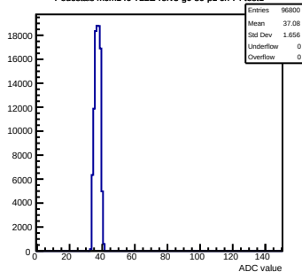
Pedestals mcm140-722E-refv3-g0-s0-p1 ch 74 test1
