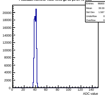
Pedestals mcm140-722E-refv3-g0-s0-p1 ch 70 test1
