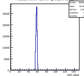
Pedestals mcm140-722E-refv4-g0-s0-p1 ch 55 test1
