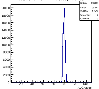
Pedestals mcm140-722E-refV5-g0-s0-p1 ch 32 test1
