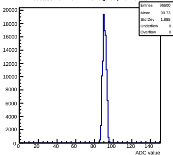
Pedestals mcm140-722E-refV5-g0-s0-p1 ch 40 test1
