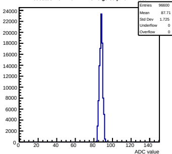
Pedestals mcm140-722E-refV5-g0-s0-p1 ch 44 test1
