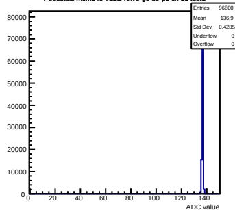
Pedestals mcm140-722E-refV0-g0-s0-p1 ch 11 test1
