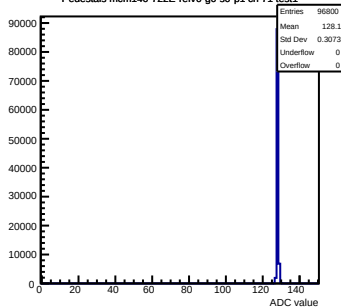
Pedestals mcm140-722E-refV0-g0-s0-p1 ch 71 test1
