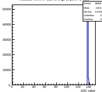
Pedestals mcm140-722E-refV0-g0-s0-p1 ch 78 test1
