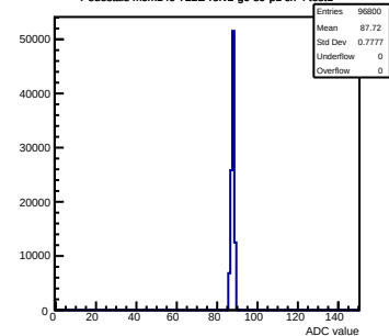
Pedestals mcm140-722E-refv2-g0-s0-p1 ch 4 test1
