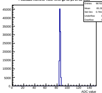
Pedestals mcm140-722E-refV2-g0-s0-p1 ch 82 test1
