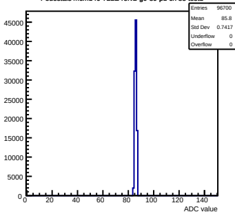
Pedestals mcm140-722E-refV2-g0-s0-p1 ch 88 test1
