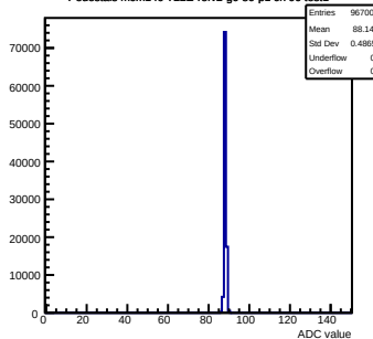
Pedestals mcm140-722E-refV2-g0-s0-p1 ch 90 test1
