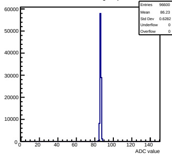
Pedestals mcm140-722E-refv2-g0-s0-p1 ch 45 test1
