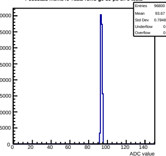
Pedestals mcm140-722E-refv2-g0-s0-p1 ch 9 test1
