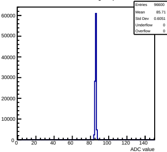
Pedestals mcm140-722E-refv2-g0-s0-p1 ch 40 test1
