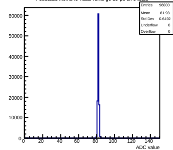
Pedestals mcm140-722E-refv2-g0-s0-p1 ch 0 test1
