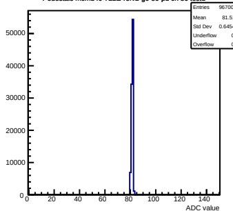
Pedestals mcm140-722E-refV2-g0-s0-p1 ch 86 test1
