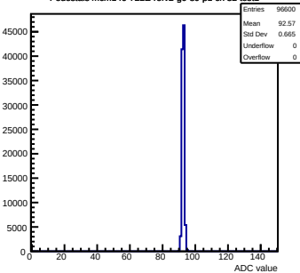
Pedestals mcm140-722E-refv2-g0-s0-p1 ch 32 test1
