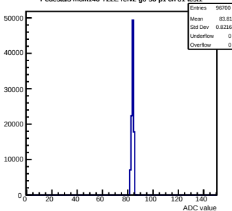
Pedestals mcm140-722E-refV2-g0-s0-p1 ch 81 test1
