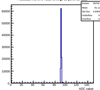
Pedestals mcm140-722E-refV2-g0-s0-p1 ch 89 test1
