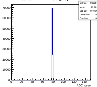
Pedestals mcm140-722E-refV4-g0-s0-p1 ch 5 test1
