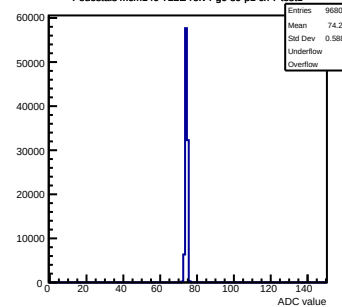
Pedestals mcm140-722E-refV4-g0-s0-p1 ch 7 test1
