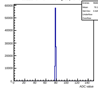
Pedestals mcm140-722E-refV4-g0-s0-p1 ch 15 test1
