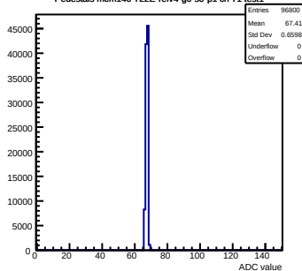
Pedestals mcm140-722E-refv4-g0-s0-p1 ch 71 test1
