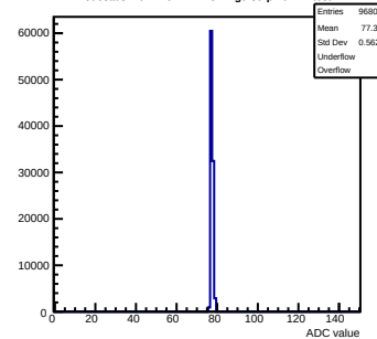
Pedestals mcm140-722E-refV4-g0-s0-p1 ch 11 test1
