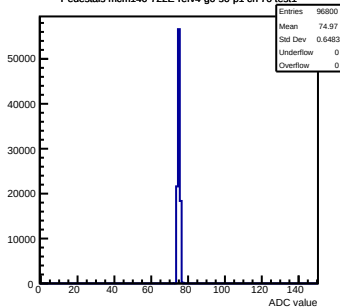
Pedestals mcm140-722E-refv4-g0-s0-p1 ch 70 test1
