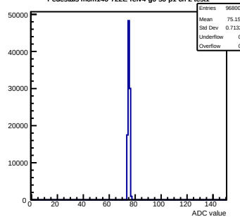
Pedestals mcm140-722E-refV4-g0-s0-p1 ch 2 test1
