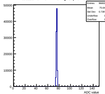
Pedestals mcm140-722E-refV4-g0-s0-p1 ch 10 test1
