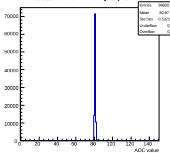
Pedestals mcm140-722E-refV4-g0-s0-p1 ch 9 test1
