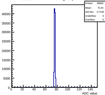
Pedestals mcm140-722E-refV4-g0-s0-p1 ch 8 test1
