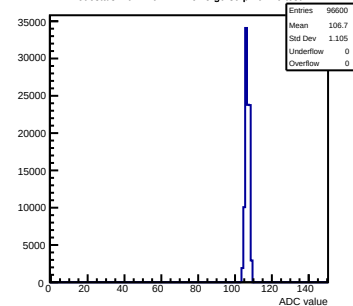
Pedestals mcm140-722E-refV5-g0-s0-p1 ch 40 test1
