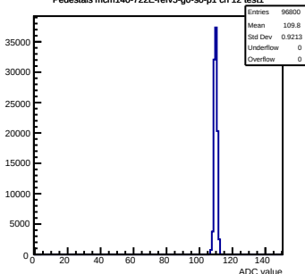
Pedestals mcm140-722E-refV5-g0-s0-p1 ch 12 test1
