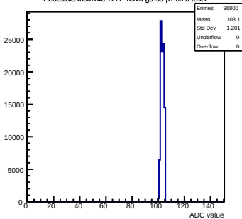
Pedestals mcm140-722E-refV5-g0-s0-p1 ch 0 test1
