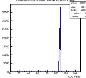
Pedestals mcm140-722E-refV5-g0-s0-p1 ch 1 test1
