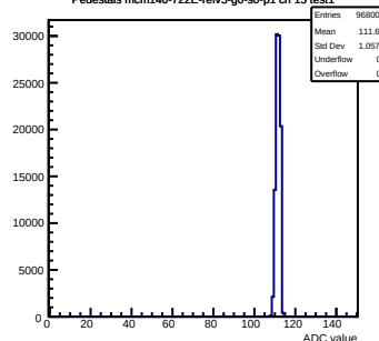
Pedestals mcm140-722E-refV5-g0-s0-p1 ch 15 test1
