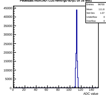
Pedestals mcm140-722E-refV5-g0-s0-p1 ch 16 test1
