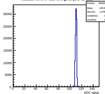
Pedestals mcm140-722E-refV5-g0-s0-p1 ch 35 test1
