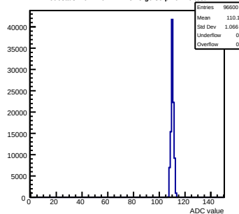
Pedestals mcm140-722E-refV5-g0-s0-p1 ch 46 test1
