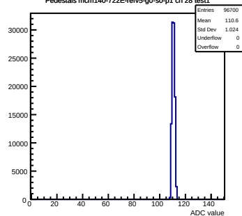
Pedestals mcm140-722E-refV5-g0-s0-p1 ch 28 test1
