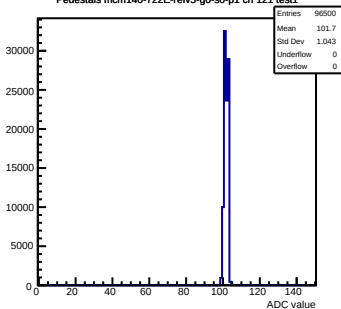
Pedestals mcm140-722E-reV5-g0-s0-p1 ch 121 test1
