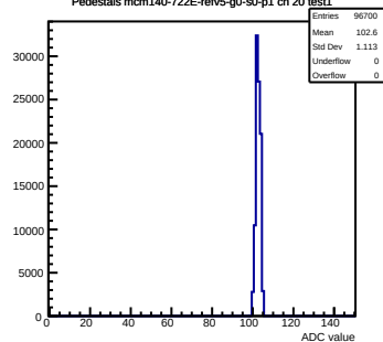
Pedestals mcm140-722E-refV5-g0-s0-p1 ch 20 test1
