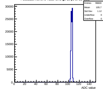
Pedestals mcm140-722E-refV5-g0-s0-p1 ch 36 test1
