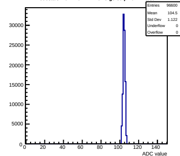
Pedestals mcm140-722E-refV5-g0-s0-p1 ch 44 test1
