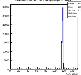
Pedestals mcm140-722E-refV5-g0-s0-p1 ch 30 test1
