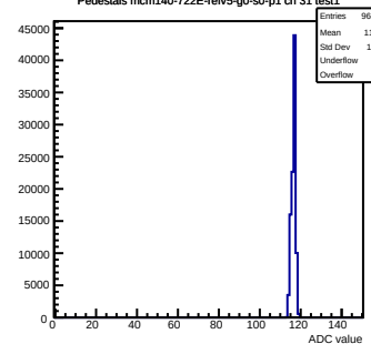
Pedestals mcm140-722E-refV5-g0-s0-p1 ch 31 test1
