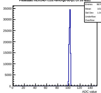
Pedestals mcm140-722E-refV5-g0-s0-p1 ch 26 test1
