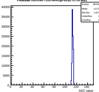
Pedestals mcm140-722E-refV5-g0-s0-p1 ch 29 test1
