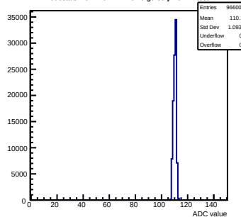
Pedestals mcm140-722E-refV5-g0-s0-p1 ch 47 test1
