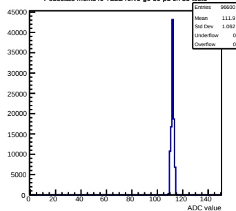
Pedestals mcm140-722E-refV5-g0-s0-p1 ch 33 test1
