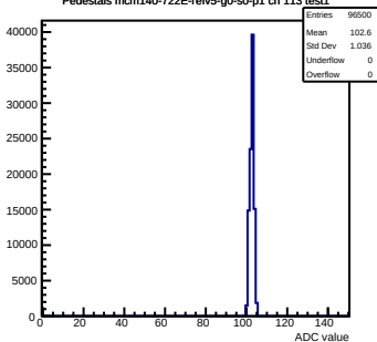
Pedestals mcm140-722E-reV5-g0-s0-p1 ch 113 test1
