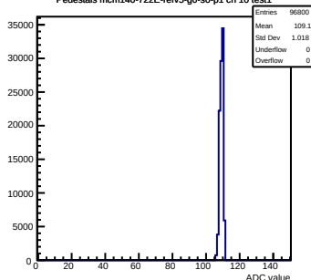
Pedestals mcm140-722E-refV5-g0-s0-p1 ch 10 test1
