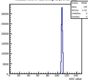
Pedestals mcm140-722E-reV5-g0-s0-p1 ch 127 test1
