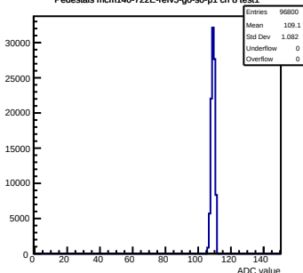
Pedestals mcm140-722E-refV5-g0-s0-p1 ch 8 test1
