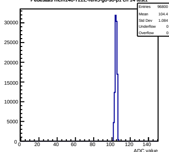
Pedestals mcm140-722E-refV5-g0-s0-p1 ch 14 test1
