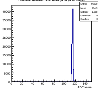
Pedestals mcm140-722E-refV5-g0-s0-p1 ch 9 test1
