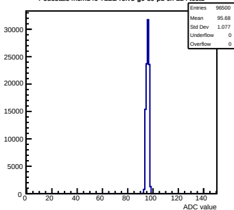
Pedestals mcm140-722E-reV5-g0-s0-p1 ch 124 test1
