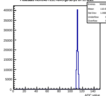
Pedestals mcm140-722E-refV5-g0-s0-p1 ch 11 test1
