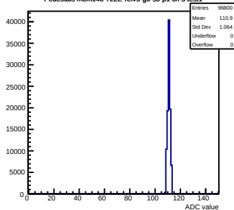
Pedestals mcm140-722E-refV5-g0-s0-p1 ch 5 test1
