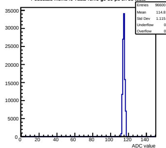
Pedestals mcm140-722E-refV5-g0-s0-p1 ch 38 test1
