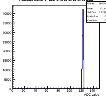
Pedestals mcm140-722E- \nu f6-g0-s0-p1 ch 83 test1
