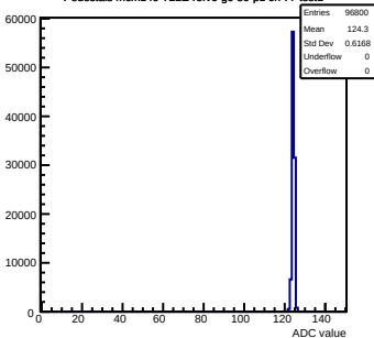
Pedestals mcm140-722E-refv6-g0-s0-p1 ch 77 test1
