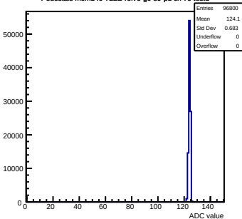
Pedestals mcm140-722E-refv6-g0-s0-p1 ch 79 test1
