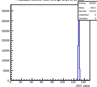
Pedestals mcm140-722E- \nu f6-g0-s0-p1 ch 80 test1
