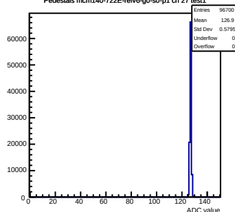
Pedestals mcm140-722E- refv6 -g0-s0-p1 ch 27 test1
