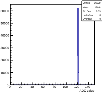
Pedestals mcm140-722E-refv6-g0-s0-p1 ch 121 test1
