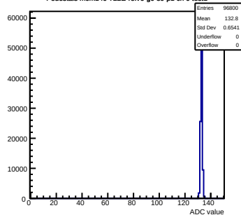
Pedestals mcm140-722E-rlv6-g0-s0-p1 ch 9 test1
