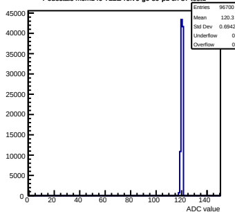
Pedestals mcm140-722E- \nu f6-g0-s0-p1 ch 87 test1
