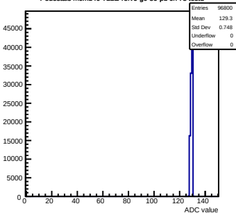
Pedestals mcm140-722E-refv6-g0-s0-p1 ch 78 test1
