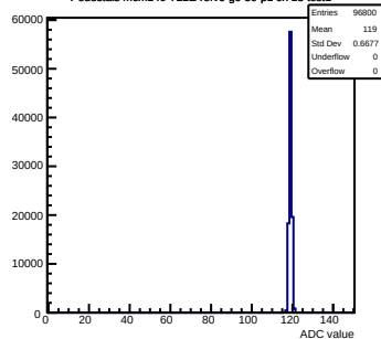
Pedestals mcm140-722E-rlv6-g0-s0-p1 ch 13 test1
