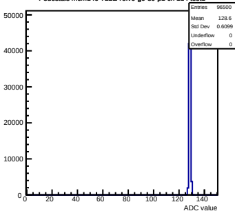
Pedestals mcm140-722E-refv6-g0-s0-p1 ch 114 test1
