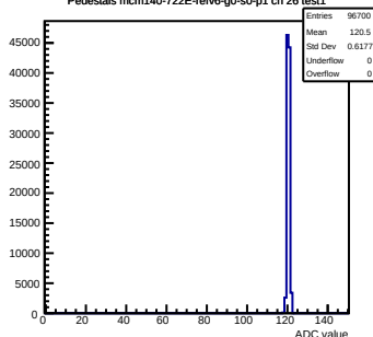
Pedestals mcm140-722E- refv6 -g0-s0-p1 ch 26 test1
