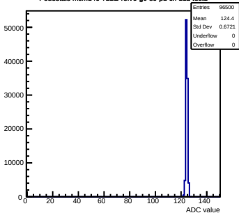
Pedestals mcm140-722E-refv6-g0-s0-p1 ch 112 test1
