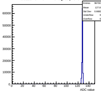
Pedestals mcm140-722E- \nu f6-g0-s0-p1 ch 94 test1
