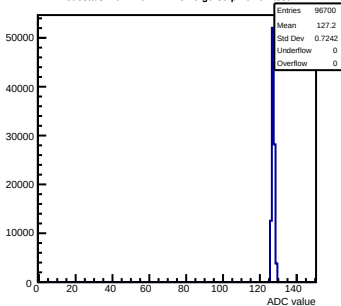
Pedestals mcm140-722E- \nu f6-g0-s0-p1 ch 92 test1
