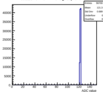
Pedestals mcm140-722E- \nu f6-g0-s0-p1 ch 91 test1
