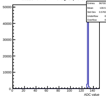
Pedestals mcm140-722E- \nu f6-g0-s0-p1 ch 89 test1
