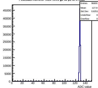
Pedestals mcm140-722E-rlv6-g0-s0-p1 ch 2 test1
