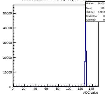
Pedestals mcm140-722E-rlv6-g0-s0-p1 ch 10 test1
