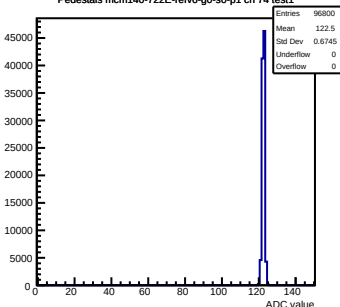
Pedestals mcm140-722E-refv6-g0-s0-p1 ch 74 test1
