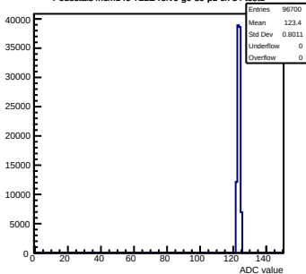
Pedestals mcm140-722E- \nu f6-g0-s0-p1 ch 84 test1
