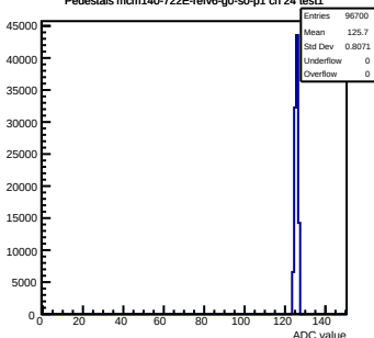
Pedestals mcm140-722E- refv6 -g0-s0-p1 ch 24 test1
