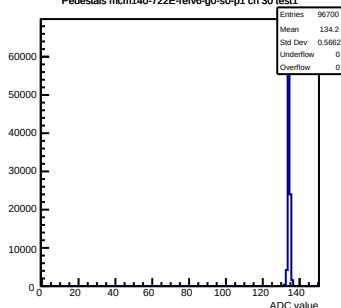
Pedestals mcm140-722E- refv6 -g0-s0-p1 ch 30 test1
