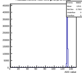
Pedestals mcm140-722E-rlv6-g0-s0-p1 ch 5 test1
