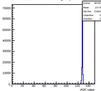
Pedestals mcm140-722E- \nu f6-g0-s0-p1 ch 90 test1
