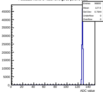
Pedestals mcm140-722E-rlv6-g0-s0-p1 ch 8 test1
