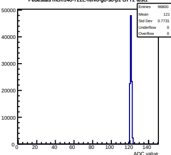
Pedestals mcm140-722E-refv6-g0-s0-p1 ch 72 test1
