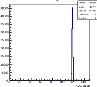
Pedestals mcm140-722E-refv6-g0-s0-p1 ch 117 test1
