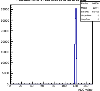
Pedestals mcm140-722E-refv6-g0-s0-p1 ch 68 test1
