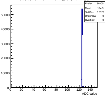
Pedestals mcm140-722E-refv6-g0-s0-p1 ch 76 test1
