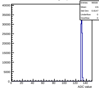
Pedestals mcm140-722E-refv6-g0-s0-p1 ch 123 test1
