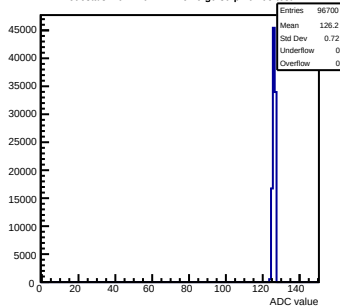
Pedestals mcm140-722E- \nu f6-g0-s0-p1 ch 95 test1
