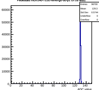
Pedestals mcm140-722E- refv6 -g0-s0-p1 ch 28 test1
