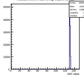
Pedestals mcm140-722E-rlv6-g0-s0-p1 ch 11 test1
