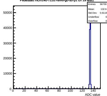
Pedestals mcm140-722E- refv6 -g0-s0-p1 ch 19 test1
