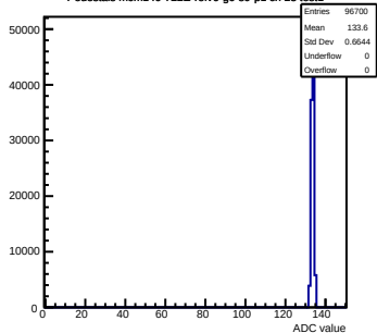
Pedestals mcm140-722E-refV0-g0-s0-p1 ch 23 test1
