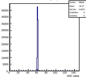
Pedestals mcm140-722E-refv2-g0-s0-p1 ch 120 test1
