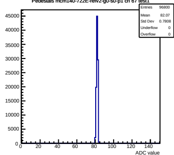
Pedestals mcm140-722E-refv2-g0-s0-p1 ch 67 test1
