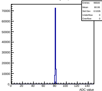
Pedestals mcm140-722E-refv2-g0-s0-p1 ch 116 test1
