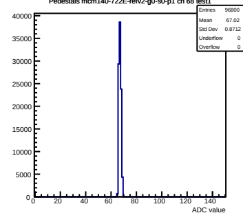
Pedestals mcm140-722E-refv2-g0-s0-p1 ch 68 test1
