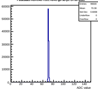
Pedestals mcm140-722E-refv2-g0-s0-p1 ch 60 test1
