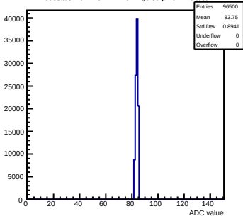
Pedestals mcm140-722E-refv2-g0-s0-p1 ch 112 test1
