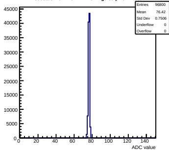
Pedestals mcm140-722E-refV2-g0-s0-p1 ch 0 test1
