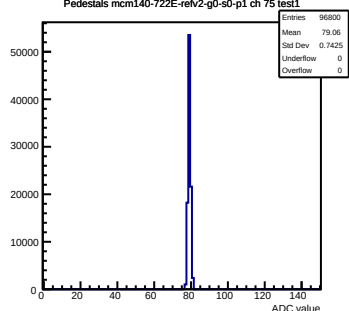
Pedestals mcm140-722E-refv2-g0-s0-p1 ch 75 test1
