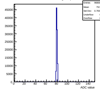
Pedestals mcm140-722E-refV2-g0-s0-p1 ch 11 test1
