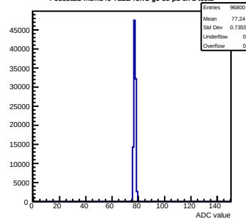
Pedestals mcm140-722E-g0-s0-p1 ch 2 test1
