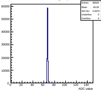
Pedestals mcm140-722E-refv2-g0-s0-p1 ch 126 test1
