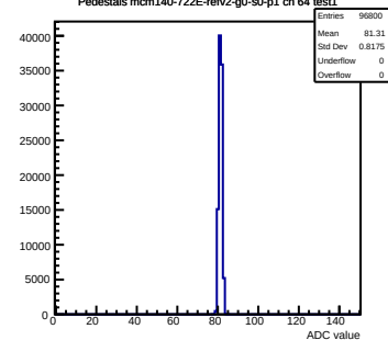
Pedestals mcm140-722E-refv2-g0-s0-p1 ch 64 test1
