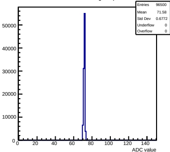
Pedestals mcm140-722E-refv2-g0-s0-p1 ch 122 test1
