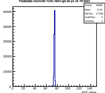
Pedestals mcm140-722E-refv2-g0-s0-p1 ch 79 test1
