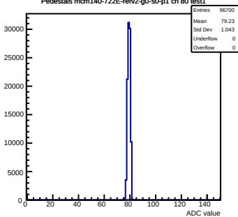
Pedestals mcm140-722E-refv2-g0-s0-p1 ch 80 test1
