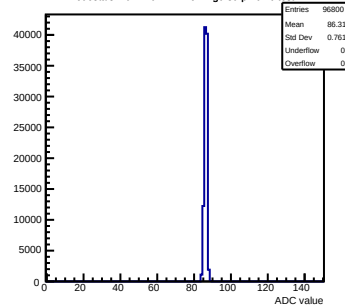
Pedestals mcm140-722E-refV2-g0-s0-p1 ch 6 test1
