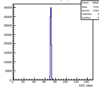
Pedestals mcm140-722E-refV2-g0-s0-p1 ch 14 test1
