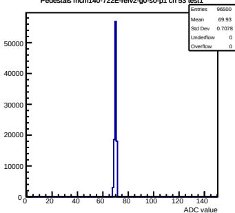
Pedestals mcm140-722E-refv2-g0-s0-p1 ch 53 test1
