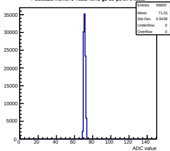
Pedestals mcm140-722E-g0-s0-p1 ch 0 test1
