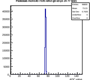
Pedestals mcm140-722E-refv2-g0-s0-p1 ch 77 test1
