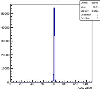
Pedestals mcm140-722E-refv2-g0-s0-p1 ch 123 test1
