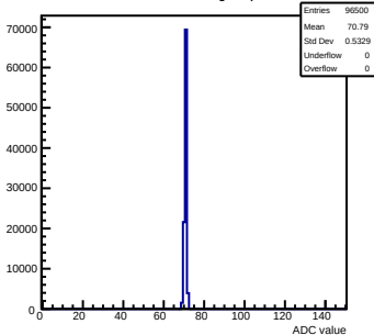
Pedestals mcm140-722E-refv2-g0-s0-p1 ch 121 test1
