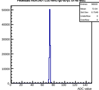
Pedestals mcm140-722E-refv2-g0-s0-p1 ch 48 test1
