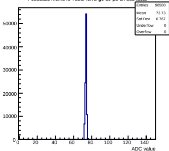
Pedestals mcm140-722E-g0-s0-p1 ch 112 test1
