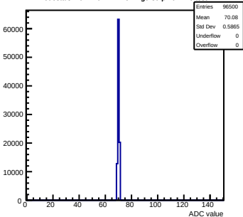
Pedestals mcm140-722E-refv2-g0-s0-p1 ch 114 test1
