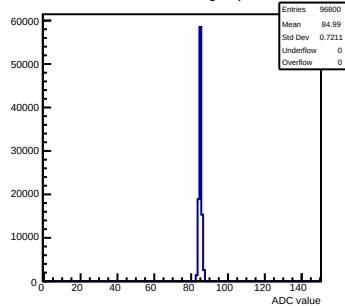
Pedestals mcm140-722E-refV2-g0-s0-p1 ch 9 test1
