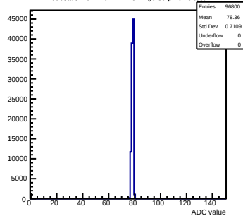
Pedestals mcm140-722E-refV2-g0-s0-p1 ch 5 test1
