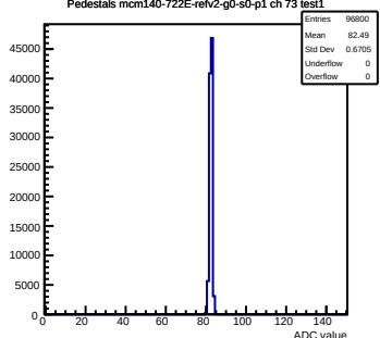
Pedestals mcm140-722E-refv2-g0-s0-p1 ch 73 test1
