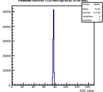
Pedestals mcm140-722E-refv2-g0-s0-p1 ch 65 test1
