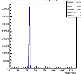
Pedestals mcm140-722E-refV3-g0-s0-p1 ch 93 test1
