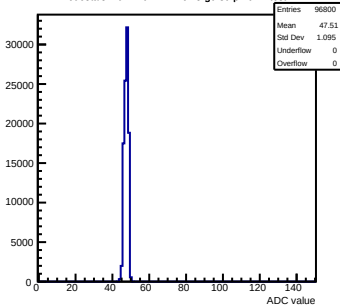
Pedestals mcm140-722E-refV3-g0-s0-p1 ch 2 test1
