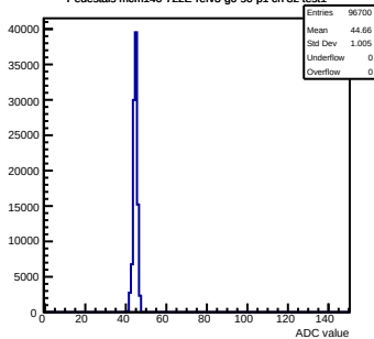
Pedestals mcm140-722E-refV3-g0-s0-p1 ch 82 test1
