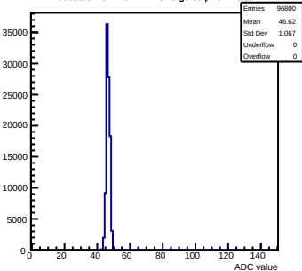
Pedestals mcm140-722E-refV3-g0-s0-p1 ch 4 test1
