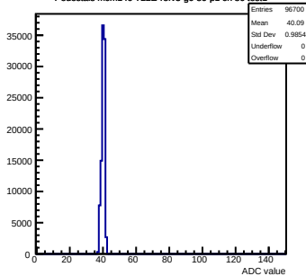
Pedestals mcm140-722E-refV3-g0-s0-p1 ch 86 test1
