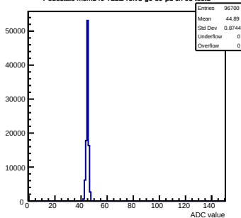
Pedestals mcm140-722E-refV3-g0-s0-p1 ch 95 test1
