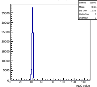
Pedestals mcm140-722E-refV3-g0-s0-p1 ch 14 test1
