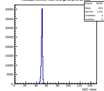
Pedestals mcm140-722E-refV3-g0-s0-p1 ch 80 test1
