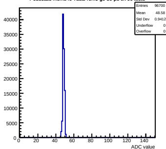
Pedestals mcm140-722E-refV3-g0-s0-p1 ch 90 test1
