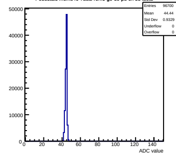
Pedestals mcm140-722E-refV3-g0-s0-p1 ch 88 test1
