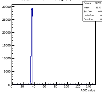
Pedestals mcm140-722E-refV3-g0-s0-p1 ch 87 test1
