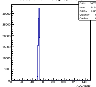
Pedestals mcm140-722E-refV3-g0-s0-p1 ch 89 test1
