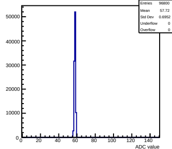
Pedestals mcm140-722E-refv4-g0-s0-p1 ch 68 test1
