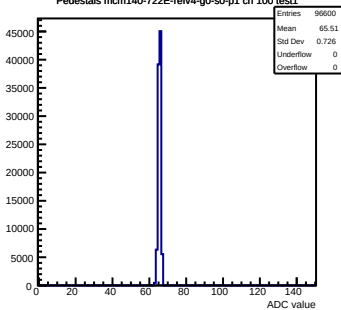
Pedestals mcm140-722E-refv4-g0-s0-p1 ch 100 test1
