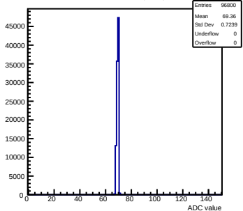
Pedestals mcm140-722E-refv4-g0-s0-p1 ch 66 test1
