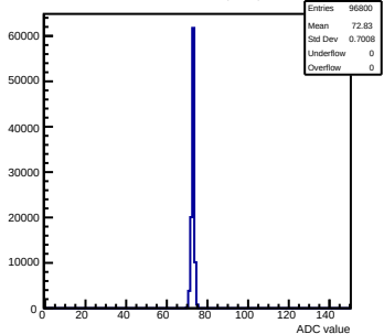
Pedestals mcm140-722E-refv4-g0-s0-p1 ch 67 test1
