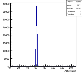
Pedestals mcm140-722E-refv4-g0-s0-p1 ch 72 test1
