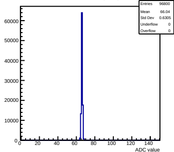
Pedestals mcm140-722E-refv4-g0-s0-p1 ch 65 test1
