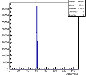
Pedestals mcm140-722E-refv4-g0-s0-p1 ch 71 test1
