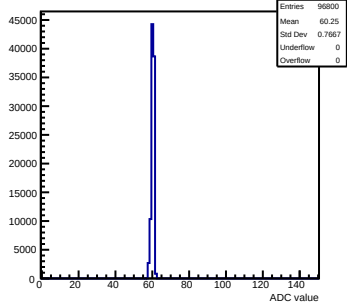
Pedestals mcm140-722E-refv4-g0-s0-p1 ch 69 test1
