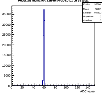
Pedestals mcm140-722E-refv4-g0-s0-p1 ch 99 test1
