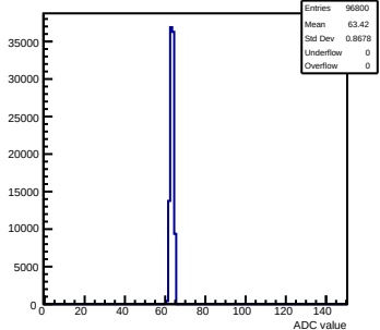
Pedestals mcm140-722E-refv4-g0-s0-p1 ch 74 test1
