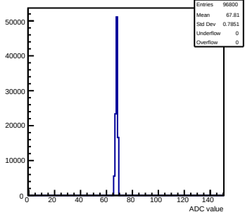
Pedestals mcm140-722E-refv4-g0-s0-p1 ch 70 test1
