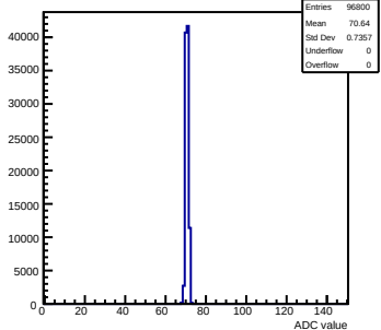
Pedestals mcm140-722E-refv4-g0-s0-p1 ch 78 test1
