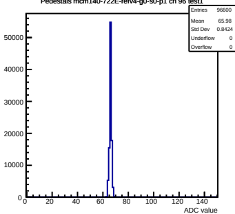
Pedestals mcm140-722E-refv4-g0-s0-p1 ch 96 test1
