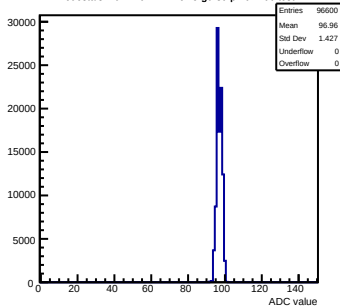
Pedestals mcm140-722E-refV5-g0-s0-p1 ch 106 test1
