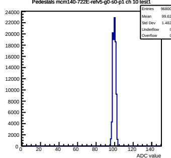
Pedestals mcm140-722E-refV5-g0-s0-p1 ch 10 test1
