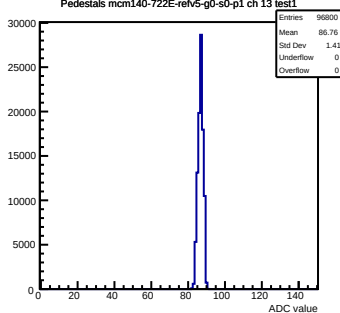
Pedestals mcm140-722E-refV5-g0-s0-p1 ch 13 test1
