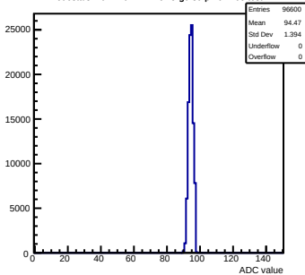
Pedestals mcm140-722E-refV5-g0-s0-p1 ch 105 test1
