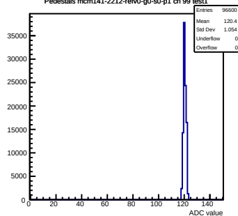
Pedestals mcm141-2212-refV0-g0-s0-p1 ch 99 test1
