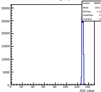
Pedestals mcm141-2212-refV0-g0-s0-p1 ch 13 test1
