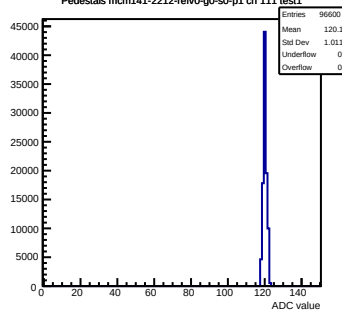
Pedestals mcm141-2212-refV0-g0-s0-p1 ch 111 test1
