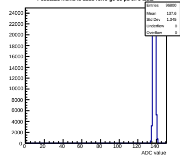
Pedestals mcm141-2212-refV0-g0-s0-p1 ch 0 test1
