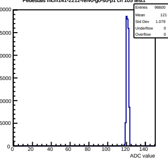
Pedestals mcm141-2212-refV0-g0-s0-p1 ch 105 test1
