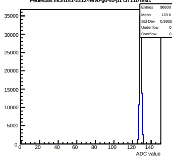
Pedestals mcm141-2212-refV0-g0-s0-p1 ch 110 test1
