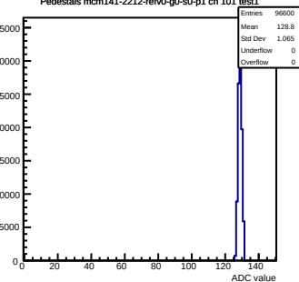
Pedestals mcm141-2212-refV0-g0-s0-p1 ch 101 test1
