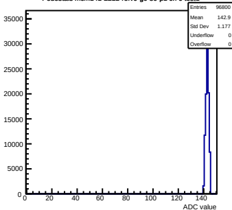
Pedestals mcm141-2212-refV0-g0-s0-p1 ch 6 test1
