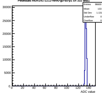
Pedestals mcm141-2212-refV0-g0-s0-p1 ch 102 test1
