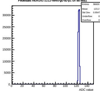
Pedestals mcm141-2212-refV0-g0-s0-p1 ch 98 test1
