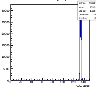
Pedestals mcm141-2212-refV0-g0-s0-p1 ch 10 test1
