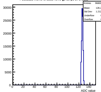
Pedestals mcm141-2212-refV0-g0-s0-p1 ch 3 test1
