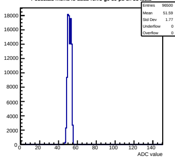
Pedestals mcm141-2212-refv3-g0-s0-p1 ch 53 test1
