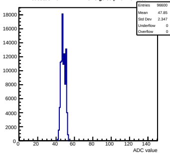
Pedestals mcm141-2212-refv3-g0-s0-p1 ch 104 test1
