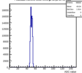
Pedestals mcm141-2212-refv3-g0-s0-p1 ch 49 test1
