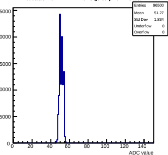
Pedestals mcm141-2212-refv3-g0-s0-p1 ch 123 test1
