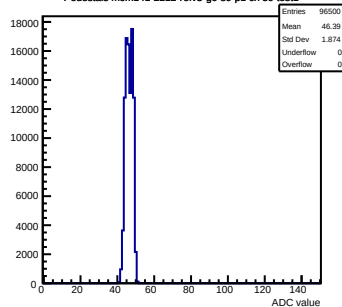
Pedestals mcm141-2212-refv3-g0-s0-p1 ch 59 test1
