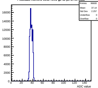
Pedestals mcm141-2212-refv3-g0-s0-p1 ch 99 test1
