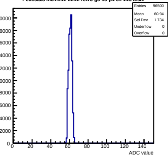
Pedestals mcm141-2212-refv3-g0-s0-p1 ch 115 test1
