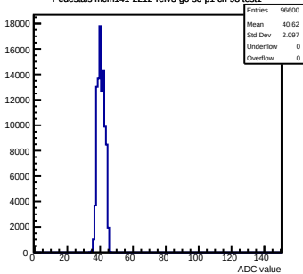
Pedestals mcm141-2212-refv3-g0-s0-p1 ch 98 test1
