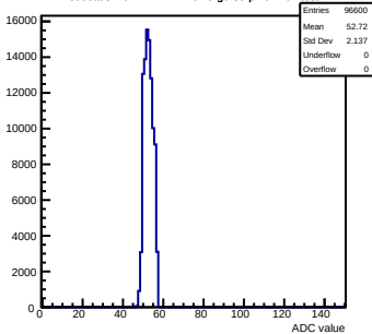
Pedestals mcm141-2212-refv3-g0-s0-p1 ch 102 test1
