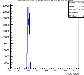
Pedestals mcm141-2212-refv3-g0-s0-p1 ch 51 test1
