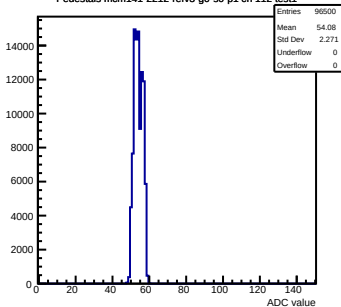
Pedestals mcm141-2212-refv3-g0-s0-p1 ch 112 test1
