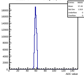
Pedestals mcm141-2212-refv3-g0-s0-p1 ch 120 test1
