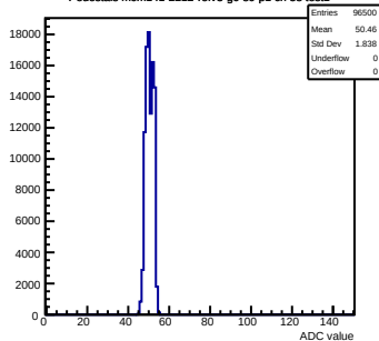
Pedestals mcm141-2212-refv3-g0-s0-p1 ch 58 test1
