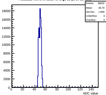
Pedestals mcm141-2212-refv3-g0-s0-p1 ch 52 test1
