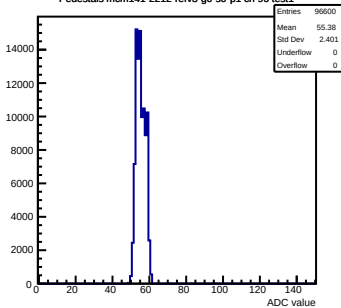
Pedestals mcm141-2212-refv3-g0-s0-p1 ch 96 test1
