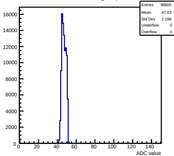
Pedestals mcm141-2212-refv3-g0-s0-p1 ch 108 test1
