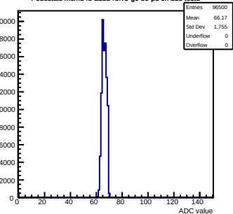
Pedestals mcm141-2212-refv3-g0-s0-p1 ch 118 test1
