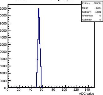
Pedestals mcm141-2212-refv3-g0-s0-p1 ch 126 test1
