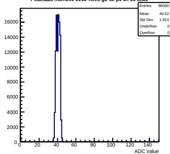
Pedestals mcm141-2212-refv3-g0-s0-p1 ch 50 test1
