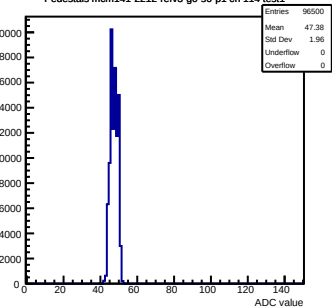
Pedestals mcm141-2212-refv3-g0-s0-p1 ch 114 test1
