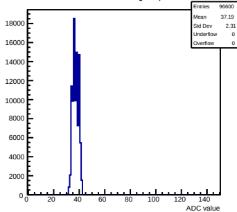
Pedestals mcm141-2212-refv3-g0-s0-p1 ch 111 test1
