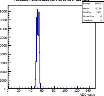
Pedestals mcm141-2212-refv3-g0-s0-p1 ch 113 test1
