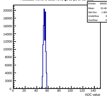
Pedestals mcm141-2212-refv3-g0-s0-p1 ch 63 test1
