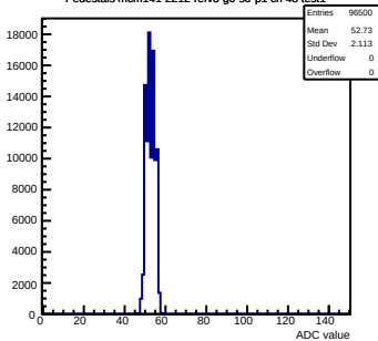
Pedestals mcm141-2212-refv3-g0-s0-p1 ch 48 test1
