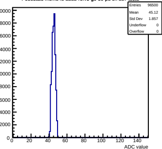
Pedestals mcm141-2212-refv3-g0-s0-p1 ch 117 test1
