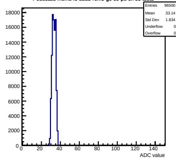
Pedestals mcm141-2212-refv3-g0-s0-p1 ch 55 test1
