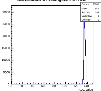
Pedestals mcm141-2212-rlv6-g0-s0-p1 ch 12 test1
