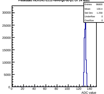
Pedestals mcm141-2212-rlv6-g0-s0-p1 ch 14 test1
