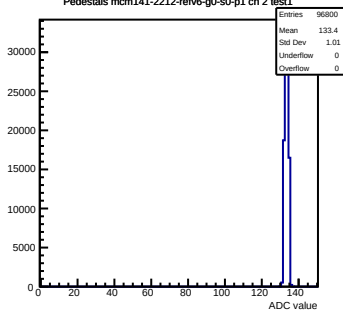
Pedestals mcm141-2212-rlv6-g0-s0-p1 ch 2 test1
