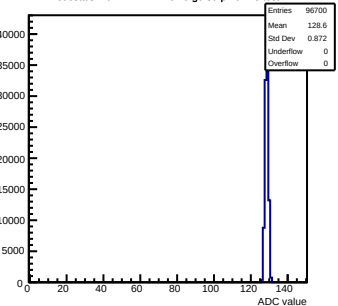
Pedestals mcm141-2212-rlv6-g0-s0-p1 ch 25 test1
