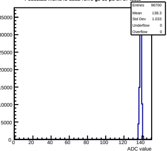
Pedestals mcm141-2212-rlv6-g0-s0-p1 ch 17 test1
