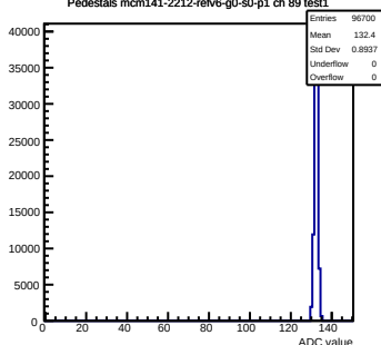
Pedestals mcm141-2212-rlv6-g0-s0-p1 ch 89 test1
