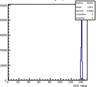
Pedestals mcm141-2212-rlv6-g0-s0-p1 ch 29 test1
