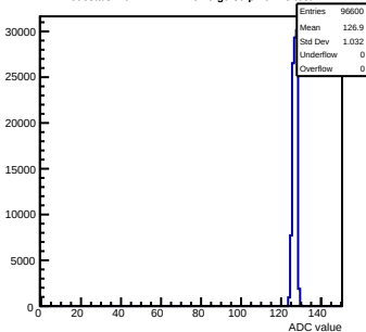
Pedestals mcm141-2212-rlv6-g0-s0-p1 ch 45 test1
