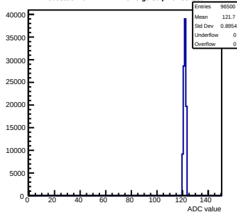
Pedestals mcm141-2212-rev0-g0-s0-p1 ch 55 test1
