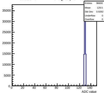
Pedestals mcm141-2212-refv0-g0-s0-p1 ch 106 test1
