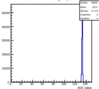
Pedestals mcm141-2212-rev0-g0-s0-p1 ch 52 test1
