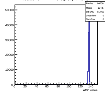
Pedestals mcm141-2212-rfv0-g0-s0-p1 ch 88 test1
