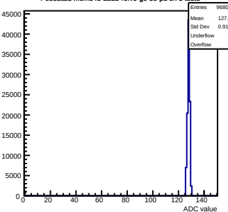
Pedestals mcm141-2212-refV0-g0-s0-p1 ch 3 test1
