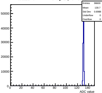
Pedestals mcm141-2212-refv0-g0-s0-p1 ch 108 test1
