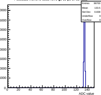
Pedestals mcm141-2212-rfv0-g0-s0-p1 ch 85 test1
