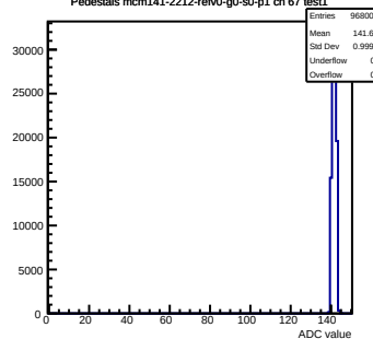
Pedestals mcm141-2212-rev0-g0-s0-p1 ch 67 test1
