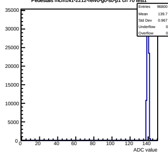
Pedestals mcm141-2212-rev0-g0-s0-p1 ch 70 test1
