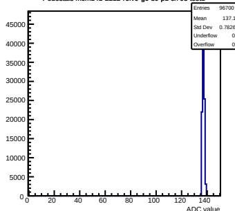
Pedestals mcm141-2212-rfv0-g0-s0-p1 ch 95 test1
