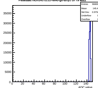
Pedestals mcm141-2212-rev0-g0-s0-p1 ch 79 test1
