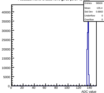
Pedestals mcm141-2212-rev0-g0-s0-p1 ch 48 test1
