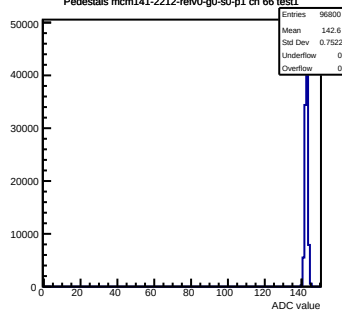
Pedestals mcm141-2212-rev0-g0-s0-p1 ch 66 test1
