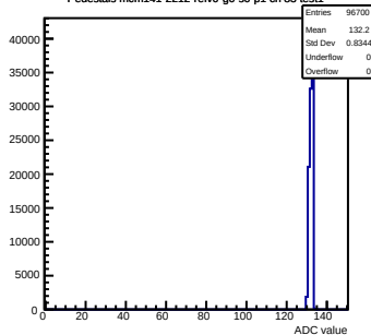
Pedestals mcm141-2212-rfv0-g0-s0-p1 ch 83 test1
