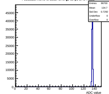
Pedestals mcm141-2212-rfv0-g0-s0-p1 ch 84 test1
