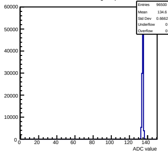
Pedestals mcm141-2212-rev0-g0-s0-p1 ch 63 test1
