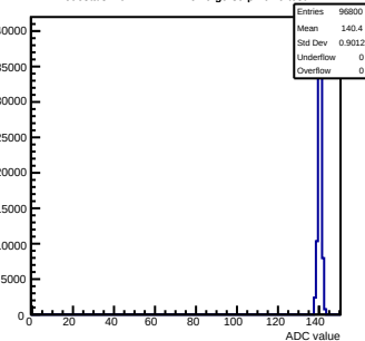
Pedestals mcm141-2212-refV0-g0-s0-p1 ch 9 test1
