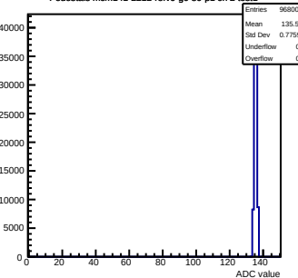
Pedestals mcm141-2212-refV0-g0-s0-p1 ch 2 test1
