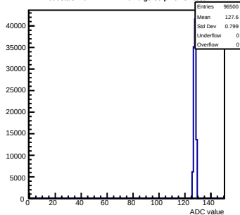
Pedestals mcm141-2212-rev0-g0-s0-p1 ch 54 test1
