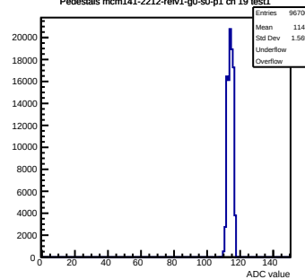
Pedestals mcm141-2212-rfv1-g0-s0-p1 ch 19 test1
