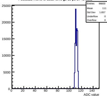
Pedestals mcm141-2212-rlv1-g0-s0-p1 ch 41 test1
