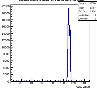
Pedestals mcm141-2212-rlv1-g0-s0-p1 ch 33 test1
