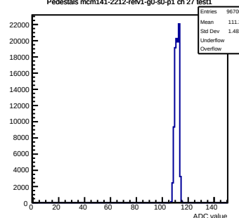
Pedestals mcm141-2212-rfv1-g0-s0-p1 ch 27 test1
