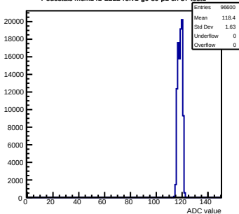
Pedestals mcm141-2212-rlv1-g0-s0-p1 ch 37 test1
