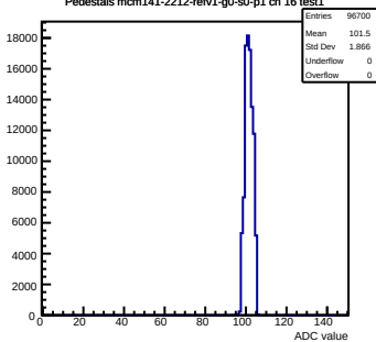
Pedestals mcm141-2212-rfv1-g0-s0-p1 ch 16 test1
