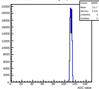
Pedestals mcm141-2212-rlv1-g0-s0-p1 ch 47 test1
