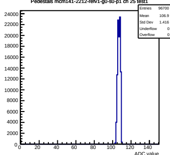
Pedestals mcm141-2212-rfv1-g0-s0-p1 ch 25 test1
