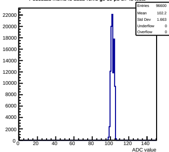
Pedestals mcm141-2212-rlv1-g0-s0-p1 ch 42 test1
