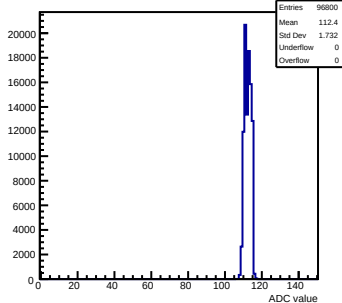
Pedestals mcm141-2212-refv1-g0-s0-p1 ch 77 test1
