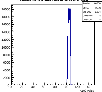
Pedestals mcm141-2212-rlv1-g0-s0-p1 ch 34 test1
