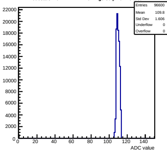
Pedestals mcm141-2212-rlv1-g0-s0-p1 ch 46 test1
