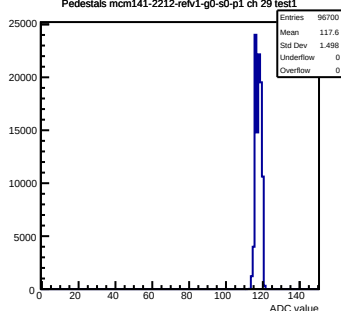
Pedestals mcm141-2212-rfv1-g0-s0-p1 ch 29 test1
