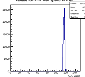
Pedestals mcm141-2212-rfv1-g0-s0-p1 ch 22 test1
