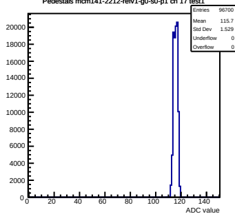
Pedestals mcm141-2212-rfv1-g0-s0-p1 ch 17 test1
