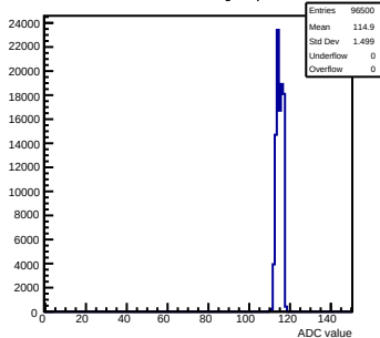
Pedestals mcm141-2212-rcv1-g0-s0-p1 ch 57 test1
