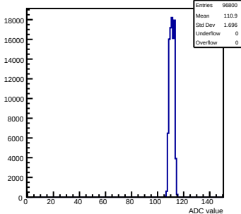
Pedestals mcm141-2212-refv1-g0-s0-p1 ch 76 test1
