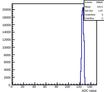
Pedestals mcm141-2212-refv1-g0-s0-p1 ch 73 test1
