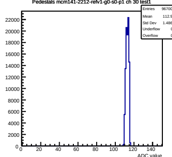
Pedestals mcm141-2212-rfv1-g0-s0-p1 ch 30 test1
