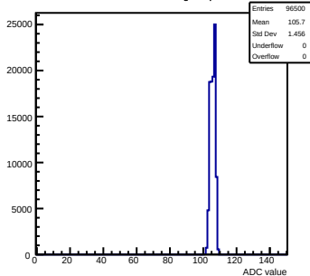
Pedestals mcm141-2212-rcv1-g0-s0-p1 ch 59 test1
