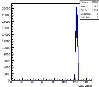
Pedestals mcm141-2212-refv1-g0-s0-p1 ch 74 test1
