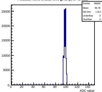
Pedestals mcm141-2212-rlv1-g0-s0-p1 ch 43 test1
