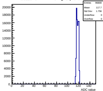
Pedestals mcm141-2212-refv1-g0-s0-p1 ch 67 test1
