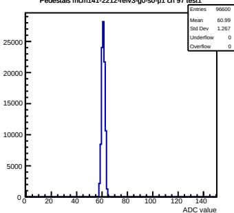
Pedestals mcm141-2212-refv3-g0-s0-p1 ch 97 test1
