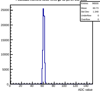
Pedestals mcm141-2212-refv3-g0-s0-p1 ch 112 test1
