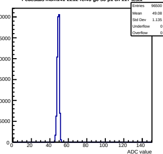
Pedestals mcm141-2212-refv3-g0-s0-p1 ch 117 test1
