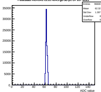
Pedestals mcm141-2212-refv3-g0-s0-p1 ch 107 test1
