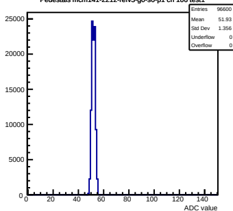
Pedestals mcm141-2212-refv3-g0-s0-p1 ch 106 test1
