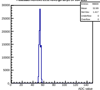
Pedestals mcm141-2212-refv3-g0-s0-p1 ch 104 test1
