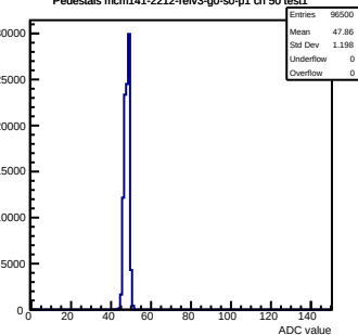
Pedestals mcm141-2212-refv3-g0-s0-p1 ch 50 test1
