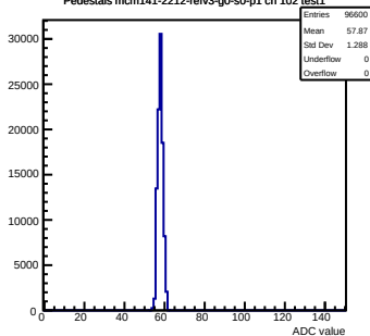
Pedestals mcm141-2212-refv3-g0-s0-p1 ch 102 test1
