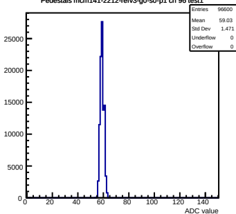
Pedestals mcm141-2212-refv3-g0-s0-p1 ch 96 test1
