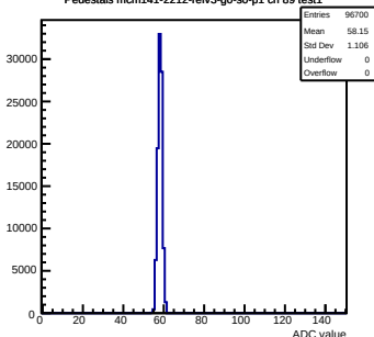
Pedestals mcm141-2212-refv3-g0-s0-p1 ch 89 test1
