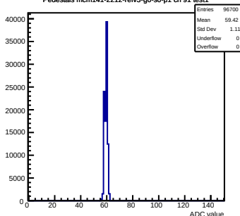
Pedestals mcm141-2212-refv3-g0-s0-p1 ch 91 test1
