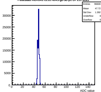
Pedestals mcm141-2212-refv3-g0-s0-p1 ch 111 test1
