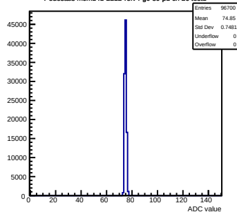
Pedestals mcm141-2212-refv4-g0-s0-p1 ch 26 test1
