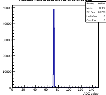
Pedestals mcm141-2212-refv4-g0-s0-p1 ch 21 test1
