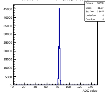
Pedestals mcm141-2212-refv4-g0-s0-p1 ch 80 test1
