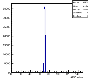
Pedestals mcm141-2212-refv4-g0-s0-p1 ch 14 test1
