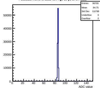
Pedestals mcm141-2212-refv4-g0-s0-p1 ch 24 test1
