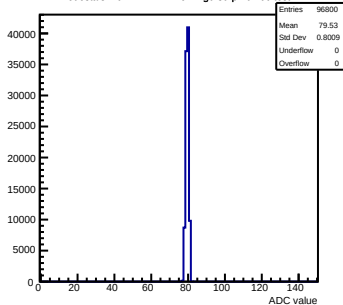
Pedestals mcm141-2212-rtv4-g0-s0-p1 ch 66 test1
