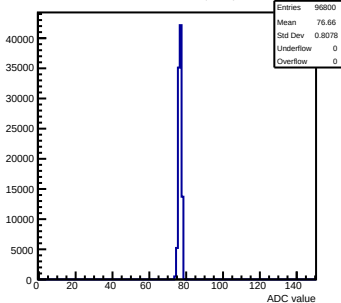
Pedestals mcm141-2212-refv4-g0-s0-p1 ch 4 test1
