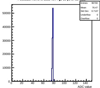
Pedestals mcm141-2212-refv4-g0-s0-p1 ch 82 test1
