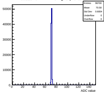
Pedestals mcm141-2212-refv4-g0-s0-p1 ch 85 test1
