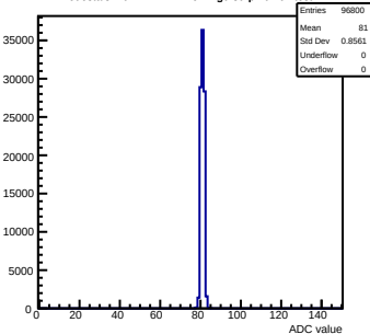
Pedestals mcm141-2212-rtv4-g0-s0-p1 ch 64 test1
