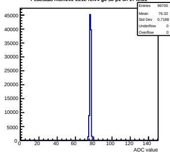
Pedestals mcm141-2212-refv4-g0-s0-p1 ch 17 test1
