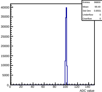
Pedestals mcm141-2212-rtv4-g0-s0-p1 ch 68 test1
