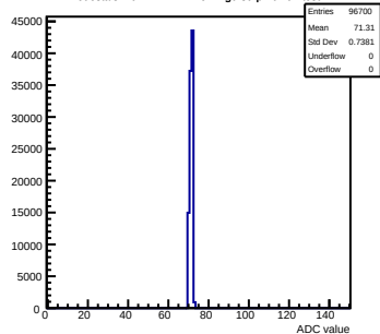
Pedestals mcm141-2212-refv4-g0-s0-p1 ch 87 test1
