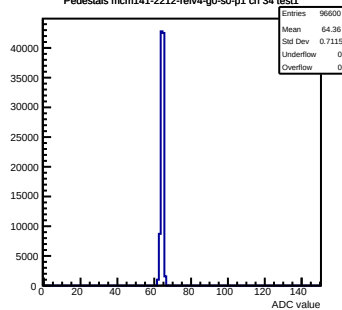
Pedestals mcm141-2212-refv4-g0-s0-p1 ch 34 test1
