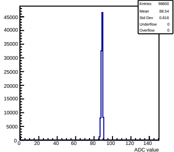
Pedestals mcm141-2212-rtv4-g0-s0-p1 ch 73 test1
