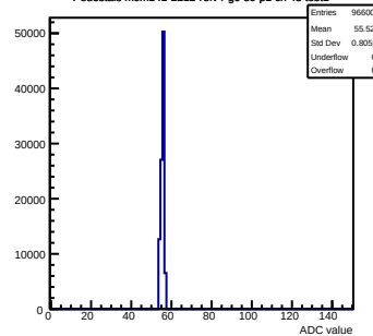
Pedestals mcm141-2212-refv4-g0-s0-p1 ch 43 test1
