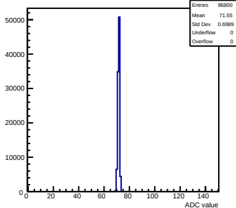
Pedestals mcm141-2212-rtv4-g0-s0-p1 ch 78 test1
