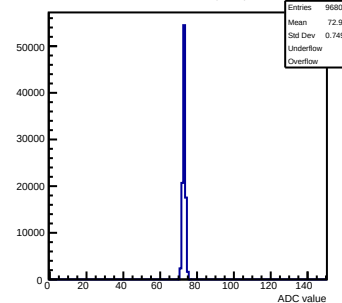
Pedestals mcm141-2212-refv4-g0-s0-p1 ch 7 test1
