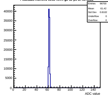
Pedestals mcm141-2212-refv4-g0-s0-p1 ch 16 test1
