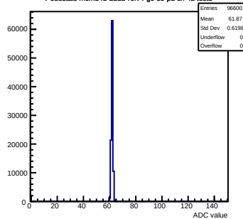
Pedestals mcm141-2212-refv4-g0-s0-p1 ch 42 test1
