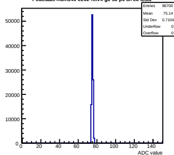
Pedestals mcm141-2212-refv4-g0-s0-p1 ch 22 test1
