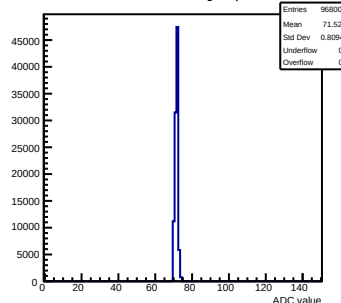
Pedestals mcm141-2212-refv4-g0-s0-p1 ch 10 test1
