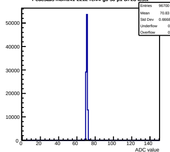
Pedestals mcm141-2212-refv4-g0-s0-p1 ch 23 test1
