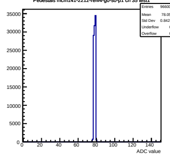
Pedestals mcm141-2212-refv4-g0-s0-p1 ch 35 test1
