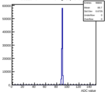
Pedestals mcm141-2212-rtv4-g0-s0-p1 ch 65 test1
