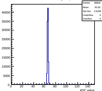
Pedestals mcm141-2212-refv4-g0-s0-p1 ch 8 test1
