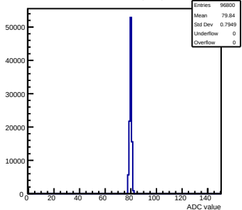
Pedestals mcm141-2212-rtv4-g0-s0-p1 ch 69 test1
