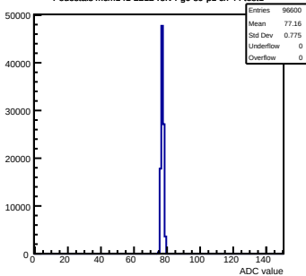
Pedestals mcm141-2212-refv4-g0-s0-p1 ch 44 test1
