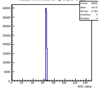
Pedestals mcm141-2212-refv4-g0-s0-p1 ch 45 test1
