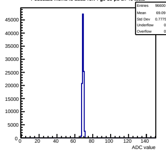
Pedestals mcm141-2212-refv4-g0-s0-p1 ch 46 test1
