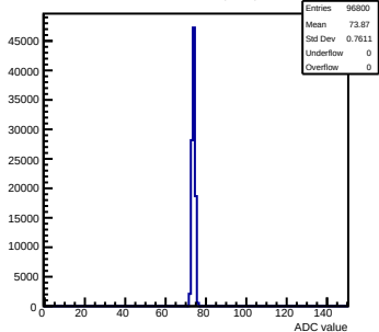
Pedestals mcm141-2212-rtv4-g0-s0-p1 ch 71 test1
