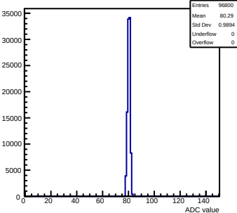
Pedestals mcm141-2212-rtv4-g0-s0-p1 ch 72 test1
