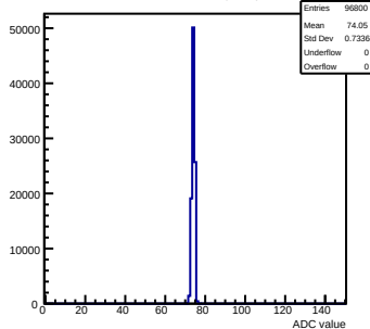
Pedestals mcm141-2212-refv4-g0-s0-p1 ch 1 test1
