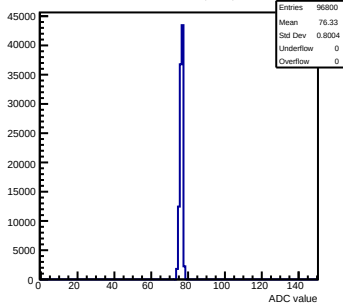
Pedestals mcm141-2212-rtv4-g0-s0-p1 ch 70 test1
