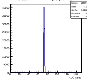
Pedestals mcm141-2212-refv4-g0-s0-p1 ch 41 test1
