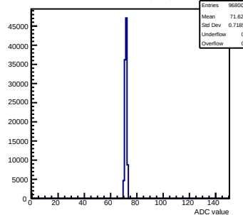
Pedestals mcm141-2212-refv4-g0-s0-p1 ch 2 test1
