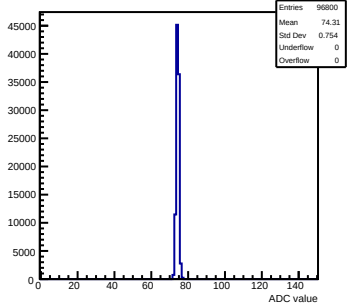
Pedestals mcm141-2212-rtv4-g0-s0-p1 ch 77 test1
