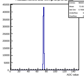
Pedestals mcm141-2212-refv4-g0-s0-p1 ch 38 test1
