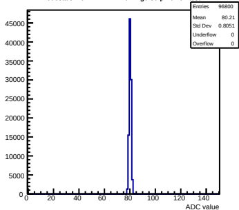
Pedestals mcm141-2212-rtv4-g0-s0-p1 ch 67 test1
