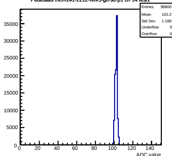
Pedestals mcm141-2212-refv5-g0-s0-p1 ch 14 test1
