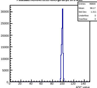
Pedestals mcm141-2212-refv5-g0-s0-p1 ch 8 test1
