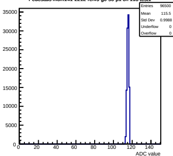
Pedestals mcm141-2212-refv5-g0-s0-p1 ch 118 test1
