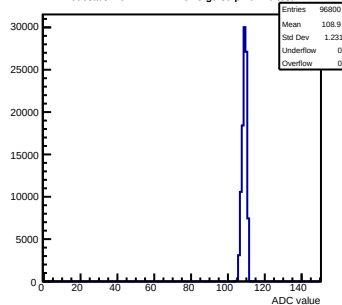
Pedestals mcm141-2212-refv5-g0-s0-p1 ch 70 test1
