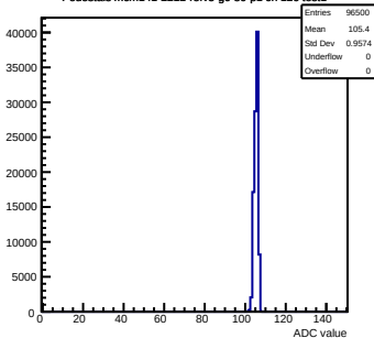
Pedestals mcm141-2212-refv5-g0-s0-p1 ch 126 test1
