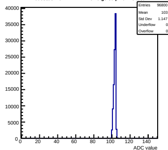
Pedestals mcm141-2212-refv5-g0-s0-p1 ch 78 test1
