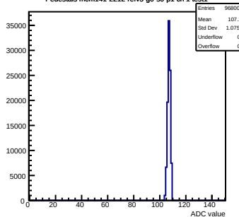
Pedestals mcm141-2212-refv5-g0-s0-p1 ch 1 test1
