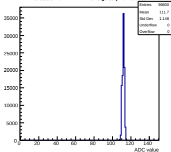
Pedestals mcm141-2212-refv5-g0-s0-p1 ch 69 test1
