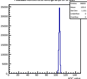
Pedestals mcm141-2212-refv5-g0-s0-p1 ch 12 test1
