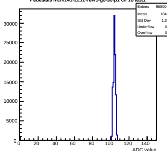
Pedestals mcm141-2212-refv5-g0-s0-p1 ch 10 test1
