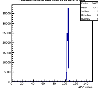
Pedestals mcm141-2212-refv5-g0-s0-p1 ch 5 test1
