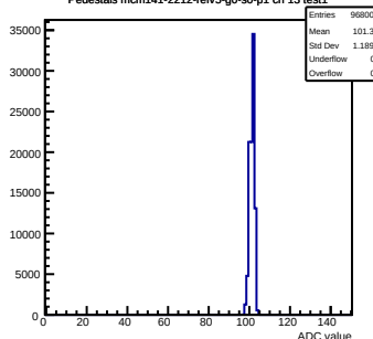
Pedestals mcm141-2212-refv5-g0-s0-p1 ch 13 test1
