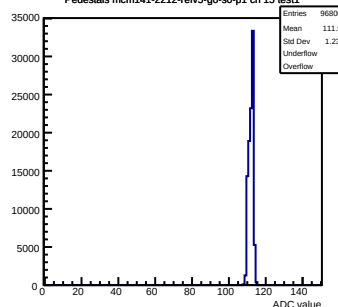
Pedestals mcm141-2212-refv5-g0-s0-p1 ch 15 test1
