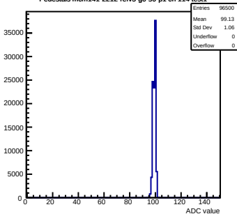
Pedestals mcm141-2212-refv5-g0-s0-p1 ch 114 test1
