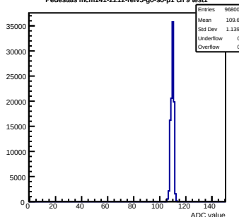
Pedestals mcm141-2212-refv5-g0-s0-p1 ch 9 test1
