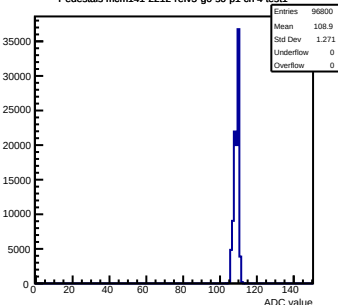
Pedestals mcm141-2212-refv5-g0-s0-p1 ch 4 test1
