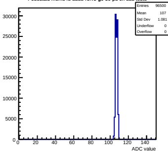
Pedestals mcm141-2212-refv5-g0-s0-p1 ch 122 test1
