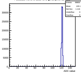
Pedestals mcm141-2212-refv5-g0-s0-p1 ch 65 test1
