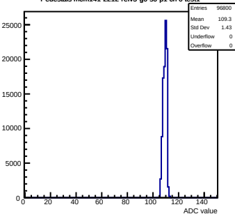
Pedestals mcm141-2212-refv5-g0-s0-p1 ch 0 test1
