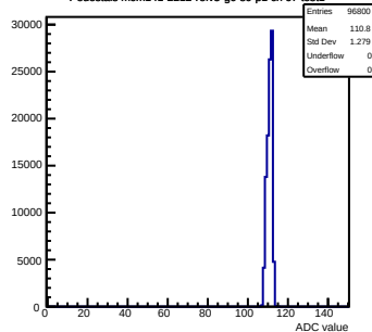
Pedestals mcm141-2212-refv5-g0-s0-p1 ch 67 test1
