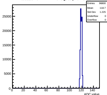
Pedestals mcm141-2212-refv5-g0-s0-p1 ch 73 test1
