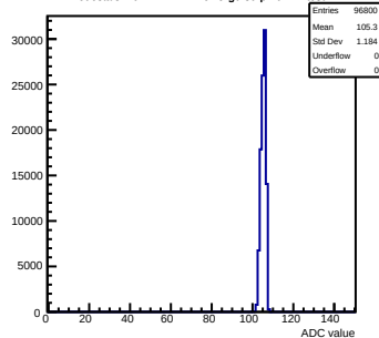
Pedestals mcm141-2212-refv5-g0-s0-p1 ch 71 test1
