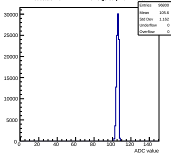
Pedestals mcm141-2212-refv5-g0-s0-p1 ch 77 test1
