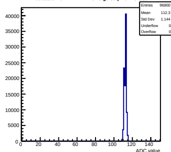
Pedestals mcm141-2212-refv5-g0-s0-p1 ch 75 test1
