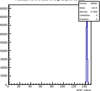
Pedestals mcm141-2212-rlv6-g0-s0-p1 ch 61 test1
