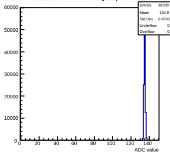
Pedestals mcm141-2212-rlv6-g0-s0-p1 ch 27 test1
