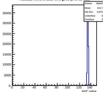
Pedestals mcm141-2212-refv6-g0-s0-p1 ch 10 test1
