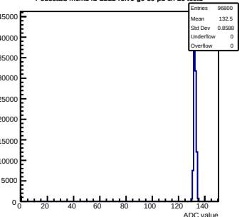
Pedestals mcm141-2212-refv6-g0-s0-p1 ch 13 test1
