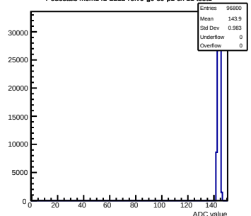
Pedestals mcm141-2212-refv6-g0-s0-p1 ch 11 test1
