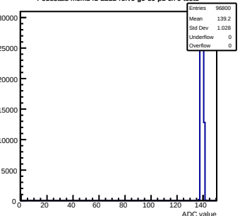
Pedestals mcm141-2212-refv6-g0-s0-p1 ch 9 test1
