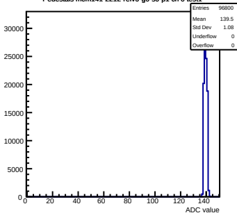
Pedestals mcm141-2212-refv6-g0-s0-p1 ch 0 test1
