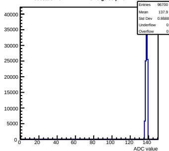
Pedestals mcm141-2212-rlv6-g0-s0-p1 ch 22 test1
