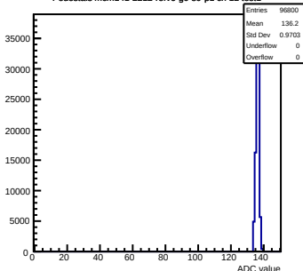
Pedestals mcm141-2212-refv6-g0-s0-p1 ch 12 test1
