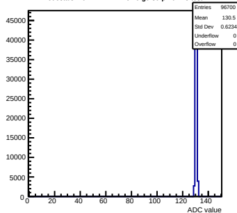
Pedestals mcm141-2212-rlv6-g0-s0-p1 ch 25 test1
