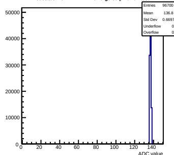
Pedestals mcm141-2212- rev0 -g0-s0-p1 ch 91 test1
