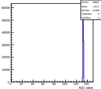
Pedestals mcm141-2212-refv0-g0-s0-p1 ch 108 test1
