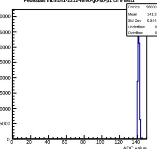
Pedestals mcm141-2212-refv0-g0-s0-p1 ch 9 test1
