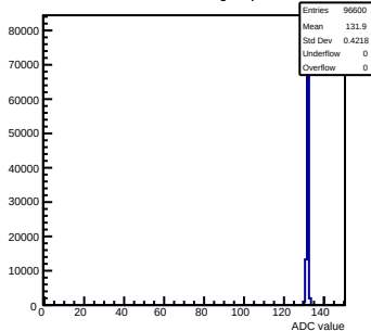
Pedestals mcm141-2212-rev0-g0-s0-p1 ch 45 test1
