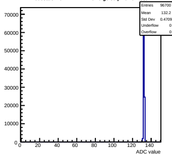
Pedestals mcm141-2212- rev0 -g0-s0-p1 ch 94 test1
