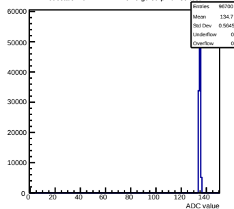
Pedestals mcm141-2212- rev0 -g0-s0-p1 ch 85 test1
