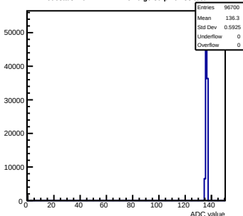
Pedestals mcm141-2212- rev0 -g0-s0-p1 ch 88 test1
