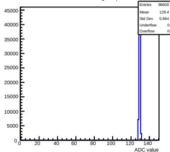
Pedestals mcm141-2212-rev0-g0-s0-p1 ch 42 test1
