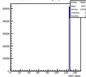
Pedestals mcm141-2212-rev0-g0-s0-p1 ch 39 test1
