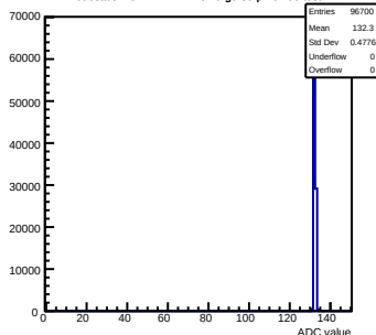
Pedestals mcm141-2212- rev0 -g0-s0-p1 ch 90 test1
