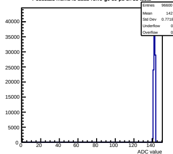
Pedestals mcm141-2212-rev0-g0-s0-p1 ch 35 test1
