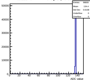
Pedestals mcm141-2212-rev0-g0-s0-p1 ch 36 test1
