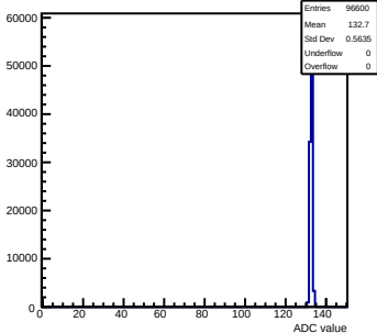
Pedestals mcm141-2212-refv0-g0-s0-p1 ch 104 test1
