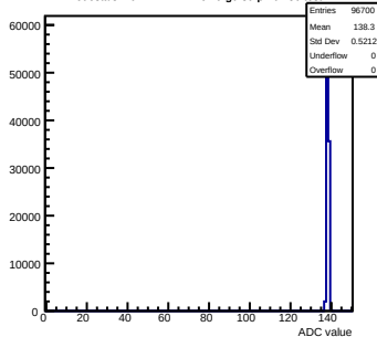
Pedestals mcm141-2212- rev0 -g0-s0-p1 ch 86 test1
