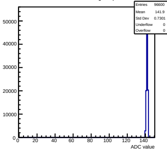
Pedestals mcm141-2212-rev0-g0-s0-p1 ch 40 test1
