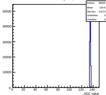
Pedestals mcm141-2212-rev0-g0-s0-p1 ch 46 test1
