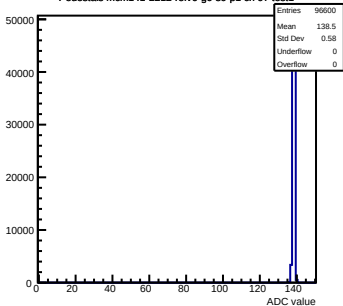
Pedestals mcm141-2212-refv0-g0-s0-p1 ch 97 test1
