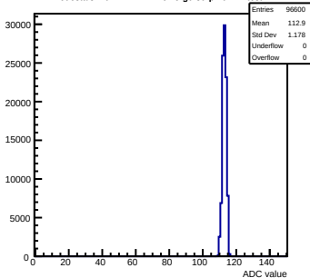
Pedestals mcm141-2212-refv5-g0-s0-p1 ch 44 test1
