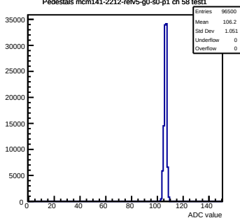
Pedestals mcm141-2212-refv5-g0-s0-p1 ch 58 test1
