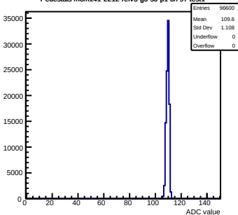
Pedestals mcm141-2212-refv5-g0-s0-p1 ch 97 test1
