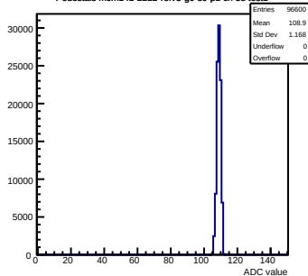
Pedestals mcm141-2212-refv5-g0-s0-p1 ch 38 test1
