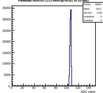
Pedestals mcm141-2212-refv5-g0-s0-p1 ch 53 test1
