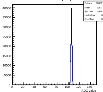
Pedestals mcm141-2212-refv5-g0-s0-p1 ch 46 test1
