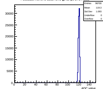
Pedestals mcm141-2212- \text{rfv5-g0-s0-p1} ch 24 \text{test1}
