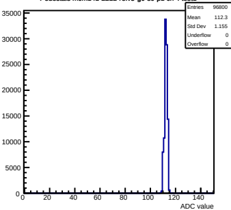
Pedestals mcm141-2212-refv5-g0-s0-p1 ch 4 test1
