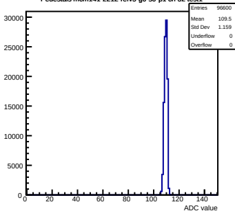
Pedestals mcm141-2212-refv5-g0-s0-p1 ch 32 test1
