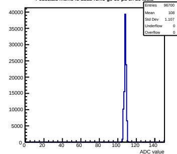
Pedestals mcm141-2212- \text{rfv5-g0-s0-p1} ch 20 \text{test1}
