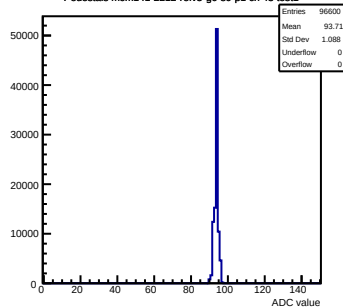
Pedestals mcm141-2212-refv5-g0-s0-p1 ch 43 test1
