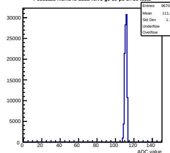
Pedestals mcm141-2212- \text{rfv5-g0-s0-p1} ch 26 \text{test1}
