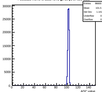
Pedestals mcm141-2212-refv5-g0-s0-p1 ch 106 test1
