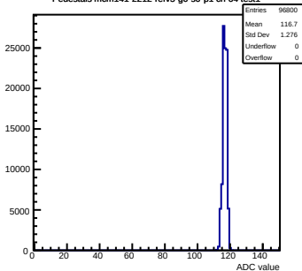
Pedestals mcm141-2212-refv5-g0-s0-p1 ch 64 test1
