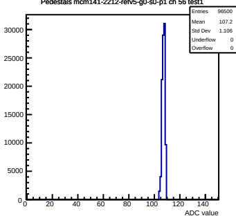
Pedestals mcm141-2212-refv5-g0-s0-p1 ch 56 test1
