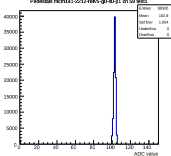
Pedestals mcm141-2212-refv5-g0-s0-p1 ch 59 test1
