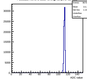
Pedestals mcm141-2212- \text{rfv5-g0-s0-p1} ch 18 \text{test1}
