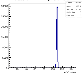
Pedestals mcm141-2212-refv5-g0-s0-p1 ch 109 test1
