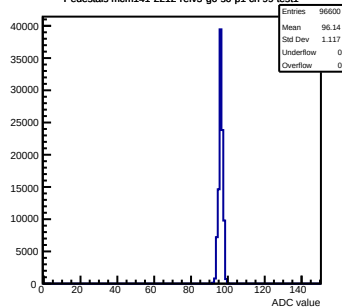
Pedestals mcm141-2212-refv5-g0-s0-p1 ch 99 test1
