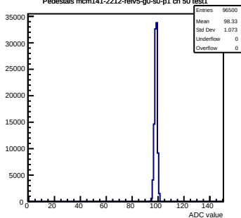
Pedestals mcm141-2212-refv5-g0-s0-p1 ch 50 test1
