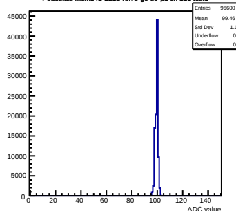
Pedestals mcm141-2212-refv5-g0-s0-p1 ch 111 test1
