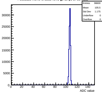
Pedestals mcm141-2212-refv5-g0-s0-p1 ch 36 test1
