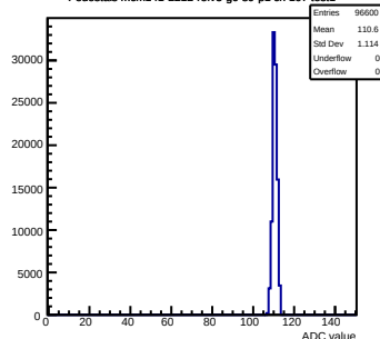
Pedestals mcm141-2212-refv5-g0-s0-p1 ch 107 test1
