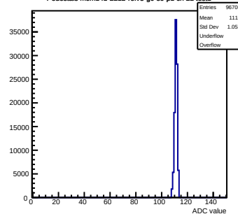
Pedestals mcm141-2212- \text{rfv5-g0-s0-p1} ch 22 \text{test1}
