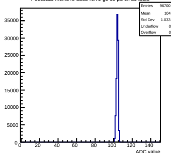
Pedestals mcm141-2212- \text{rfv5-g0-s0-p1} ch 25 \text{test1}
