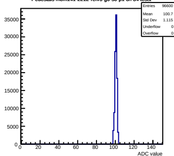
Pedestals mcm141-2212-refv5-g0-s0-p1 ch 34 test1
