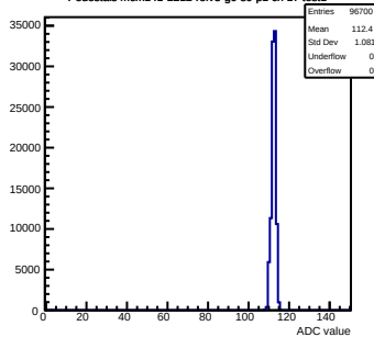
Pedestals mcm141-2212- \text{rfv5-g0-s0-p1} ch 17 \text{test1}
