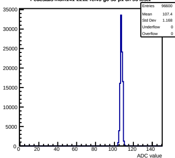
Pedestals mcm141-2212-refv5-g0-s0-p1 ch 96 test1
