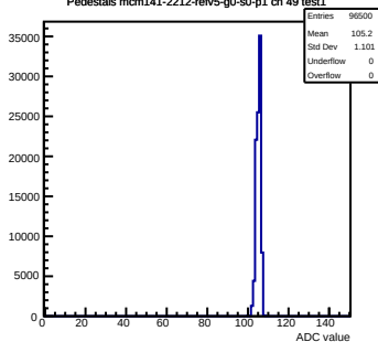
Pedestals mcm141-2212-refv5-g0-s0-p1 ch 49 test1
