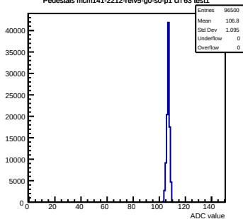
Pedestals mcm141-2212-refv5-g0-s0-p1 ch 63 test1
