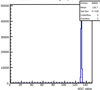
Pedestals mcm141-2212-rtv6-g0-s0-p1 ch 8 test1
