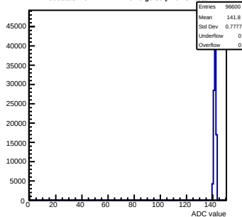
Pedestals mcm141-2212-rlv6-g0-s0-p1 ch 37 test1
