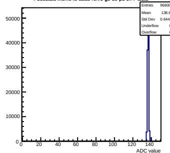
Pedestals mcm141-2212-rtv6-g0-s0-p1 ch 7 test1
