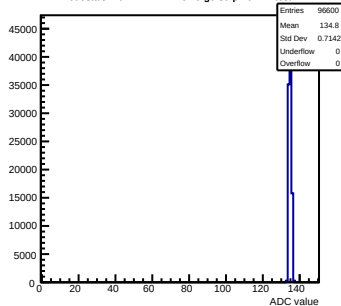
Pedestals mcm141-2212-rlv6-g0-s0-p1 ch 41 test1
