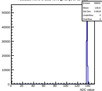
Pedestals mcm141-2212-rlv6-g0-s0-p1 ch 32 test1
