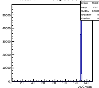
Pedestals mcm141-2212-rlv6-g0-s0-p1 ch 34 test1
