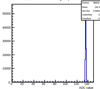
Pedestals mcm141-2212-rlv6-g0-s0-p1 ch 38 test1
