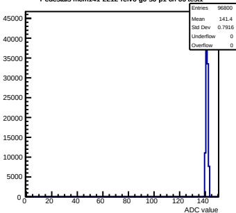
Pedestals mcm141-2212-rlv6-g0-s0-p1 ch 66 test1
