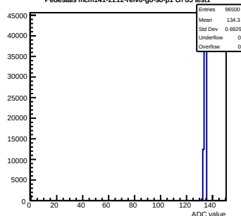
Pedestals mcm141-2212-rlv6-g0-s0-p1 ch 63 test1
