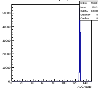
Pedestals mcm141-2212-rlv6-g0-s0-p1 ch 42 test1
