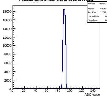
Pedestals mcm142-4215-rv1-g0-s0-p1 ch 66 test1
