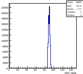
Pedestals mcm142-4215-rfv1-g0-s0-p1 ch 13 test1
