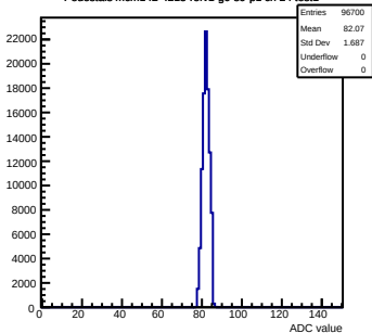
Pedestals mcm142-4215-rv1-g0-s0-p1 ch 24 test1
