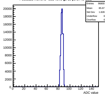
Pedestals mcm142-4215-rv1-g0-s0-p1 ch 75 test1
