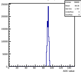
Pedestals mcm142-4215-rfv1-g0-s0-p1 ch 11 test1
