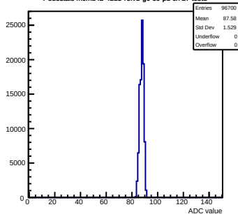
Pedestals mcm142-4215-rv1-g0-s0-p1 ch 27 test1
