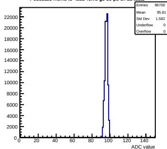
Pedestals mcm142-4215-rv1-g0-s0-p1 ch 22 test1
