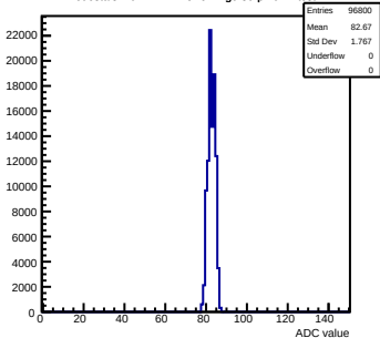
Pedestals mcm142-4215-rfv1-g0-s0-p1 ch 7 test1
