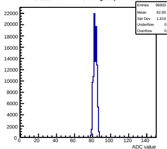
Pedestals mcm142-4215-rv1-g0-s0-p1 ch 78 test1
