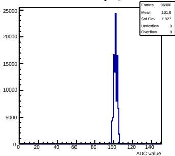
Pedestals mcm142-4215-rfv1-g0-s0-p1 ch 8 test1
