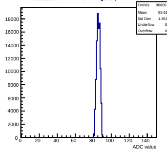
Pedestals mcm142-4215-rv1-g0-s0-p1 ch 79 test1
