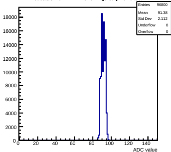
Pedestals mcm142-4215-rfv1-g0-s0-p1 ch 0 test1
