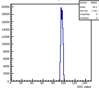
Pedestals mcm142-4215-rfv1-g0-s0-p1 ch 14 test1
