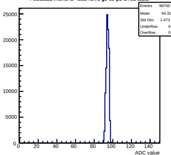
Pedestals mcm142-4215-rv1-g0-s0-p1 ch 25 test1
