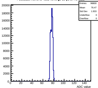
Pedestals mcm142-4215-rv1-g0-s0-p1 ch 72 test1
