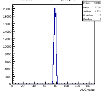
Pedestals mcm142-4215-rv1-g0-s0-p1 ch 71 test1
