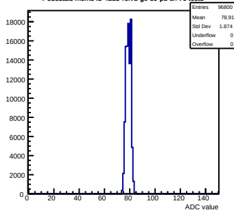
Pedestals mcm142-4215-rv1-g0-s0-p1 ch 70 test1
