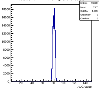
Pedestals mcm142-4215-rv1-g0-s0-p1 ch 68 test1
