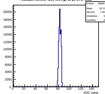
Pedestals mcm142-4215-rv1-g0-s0-p1 ch 67 test1
