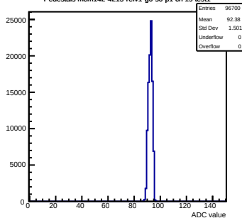
Pedestals mcm142-4215-rv1-g0-s0-p1 ch 19 test1
