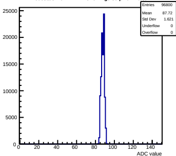
Pedestals mcm142-4215-rfv1-g0-s0-p1 ch 2 test1
