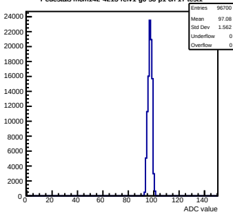
Pedestals mcm142-4215-rv1-g0-s0-p1 ch 17 test1
