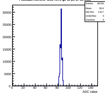
Pedestals mcm142-4215-rv1-g0-s0-p1 ch 18 test1
