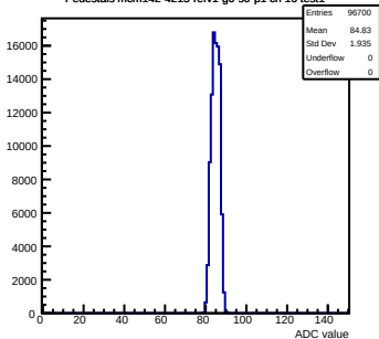
Pedestals mcm142-4215-rv1-g0-s0-p1 ch 16 test1
