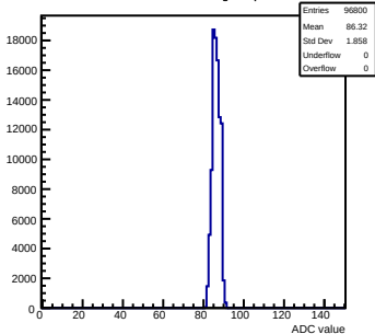
Pedestals mcm142-4215-rfv1-g0-s0-p1 ch 9 test1
