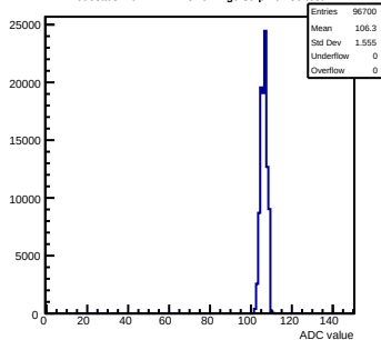
Pedestals mcm142-4215-rv1-g0-s0-p1 ch 30 test1
