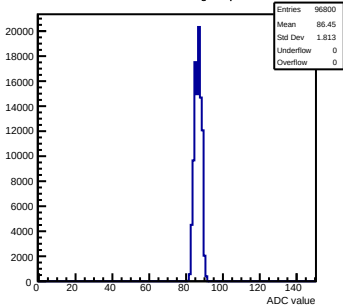
Pedestals mcm142-4215-rfv1-g0-s0-p1 ch 10 test1
