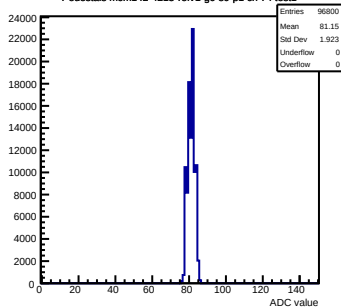
Pedestals mcm142-4215-rv1-g0-s0-p1 ch 74 test1
