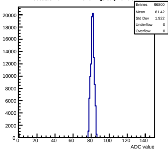
Pedestals mcm142-4215-rfv1-g0-s0-p1 ch 6 test1
