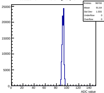
Pedestals mcm142-4215-rv1-g0-s0-p1 ch 28 test1
