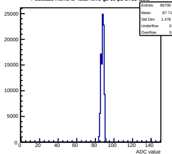
Pedestals mcm142-4215-rv1-g0-s0-p1 ch 23 test1
