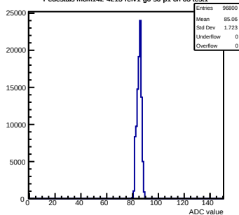
Pedestals mcm142-4215-rv1-g0-s0-p1 ch 65 test1
