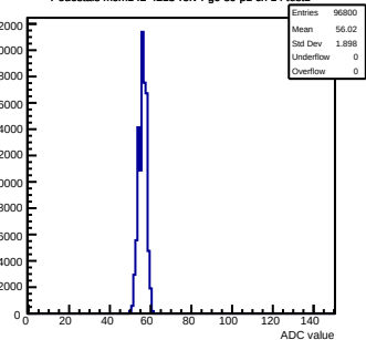
Pedestals mcm142-4215-refv4-g0-s0-p1 ch 14 test1
