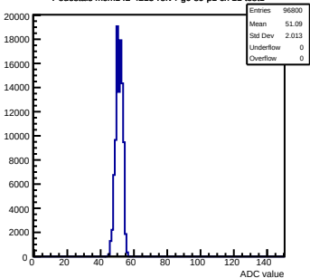
Pedestals mcm142-4215-refv4-g0-s0-p1 ch 11 test1
