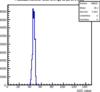
Pedestals mcm142-4215-refv4-g0-s0-p1 ch 5 test1
