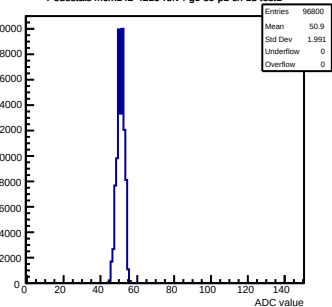
Pedestals mcm142-4215-refv4-g0-s0-p1 ch 13 test1
