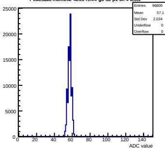
Pedestals mcm142-4215-refv4-g0-s0-p1 ch 4 test1
