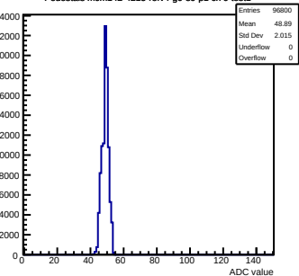
Pedestals mcm142-4215-refv4-g0-s0-p1 ch 9 test1
