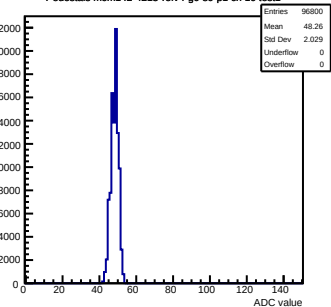
Pedestals mcm142-4215-refv4-g0-s0-p1 ch 10 test1
