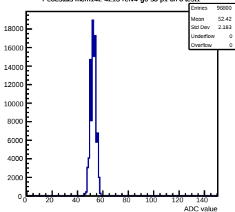
Pedestals mcm142-4215-refv4-g0-s0-p1 ch 0 test1
