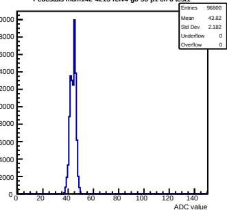
Pedestals mcm142-4215-refv4-g0-s0-p1 ch 6 test1
