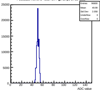
Pedestals mcm142-4215-refv4-g0-s0-p1 ch 15 test1
