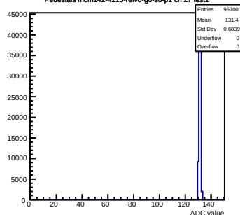
Pedestals mcm142-4215-relv0-g0-s0-p1 ch 27 test1
