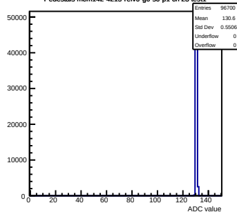
Pedestals mcm142-4215-relv0-g0-s0-p1 ch 23 test1
