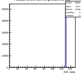
Pedestals mcm142-4215-rev0-g0-s0-p1 ch 65 test1
