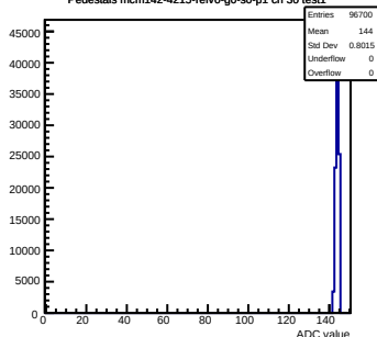
Pedestals mcm142-4215-relv0-g0-s0-p1 ch 30 test1
