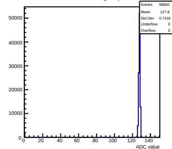
Pedestals mcm142-4215-refV0-g0-s0-p1 ch 12 test1
