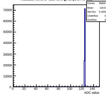
Pedestals mcm142-4215-rev0-g0-s0-p1 ch 71 test1
