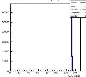
Pedestals mcm142-4215-refv0-g0-s0-p1 ch 109 test1
