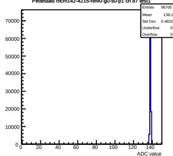
Pedestals mcm142-4215-rev0-g0-s0-p1 ch 87 test1
