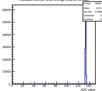
Pedestals mcm142-4215-rev0-g0-s0-p1 ch 66 test1
