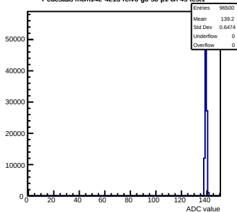
Pedestals mcm142-4215-refv0-g0-s0-p1 ch 49 test1
