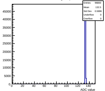
Pedestals mcm142-4215-refV0-g0-s0-p1 ch 13 test1
