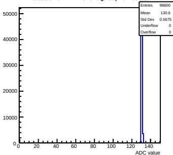
Pedestals mcm142-4215-refv0-g0-s0-p1 ch 108 test1
