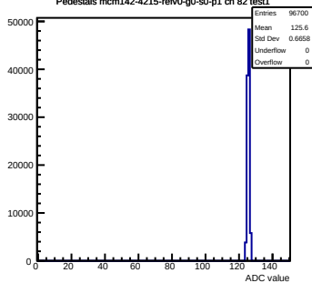
Pedestals mcm142-4215-rev0-g0-s0-p1 ch 82 test1
