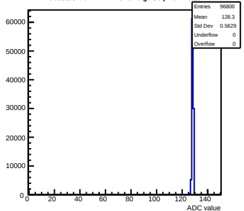
Pedestals mcm142-4215-refV0-g0-s0-p1 ch 7 test1
