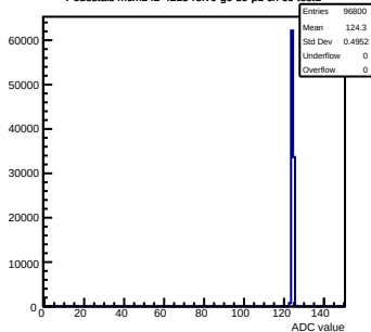
Pedestals mcm142-4215-rev0-g0-s0-p1 ch 69 test1
