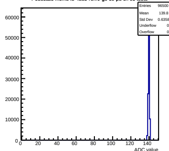
Pedestals mcm142-4215-refv0-g0-s0-p1 ch 63 test1
