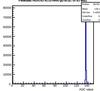
Pedestals mcm142-4215-rev0-g0-s0-p1 ch 83 test1
