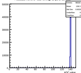
Pedestals mcm142-4215-refv0-g0-s0-p1 ch 58 test1
