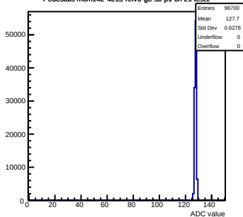
Pedestals mcm142-4215-relv0-g0-s0-p1 ch 21 test1
