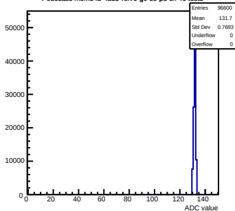
Pedestals mcm142-4215-rev0-g0-s0-p1 ch 46 test1
