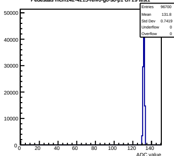
Pedestals mcm142-4215-relv0-g0-s0-p1 ch 29 test1
