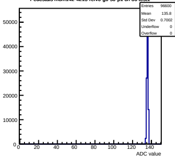
Pedestals mcm142-4215-rev0-g0-s0-p1 ch 36 test1
