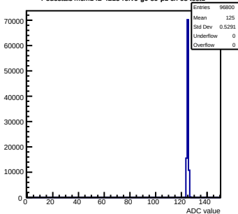
Pedestals mcm142-4215-rev0-g0-s0-p1 ch 68 test1
