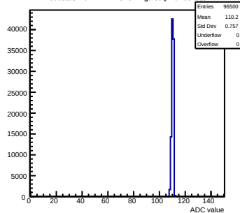
Pedestals mcm142-4215-refv1-g0-s0-p1 ch 55 test1
