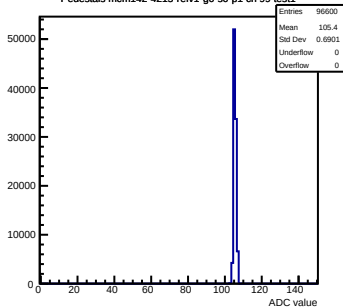
Pedestals mcm142-4215-refv1-g0-s0-p1 ch 99 test1
