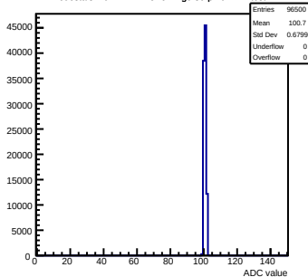
Pedestals mcm142-4215-refv1-g0-s0-p1 ch 122 test1
