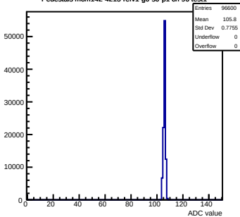
Pedestals mcm142-4215-refv1-g0-s0-p1 ch 96 test1
