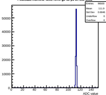
Pedestals mcm142-4215-refv1-g0-s0-p1 ch 112 test1
