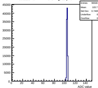
Pedestals mcm142-4215-refv1-g0-s0-p1 ch 127 test1
