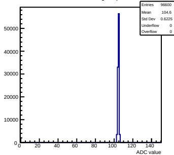
Pedestals mcm142-4215-refv1-g0-s0-p1 ch 105 test1
