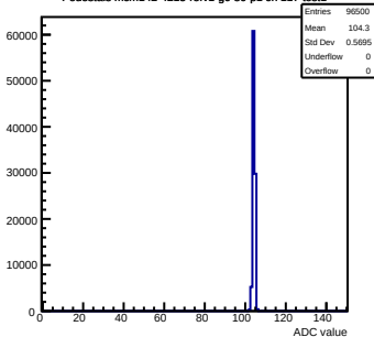
Pedestals mcm142-4215-refv1-g0-s0-p1 ch 117 test1
