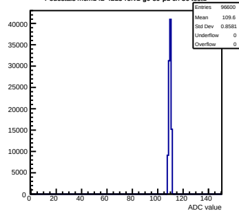
Pedestals mcm142-4215-relv1-g0-s0-p1 ch 36 test1
