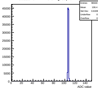
Pedestals mcm142-4215-refv1-g0-s0-p1 ch 126 test1
