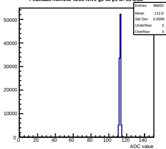
Pedestals mcm142-4215-refv1-g0-s0-p1 ch 98 test1
