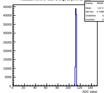
Pedestals mcm142-4215-refv1-g0-s0-p1 ch 51 test1
