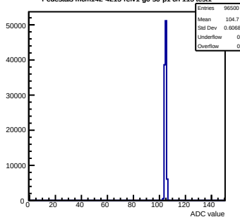
Pedestals mcm142-4215-refv1-g0-s0-p1 ch 115 test1
