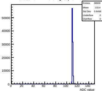
Pedestals mcm142-4215-refv1-g0-s0-p1 ch 120 test1
