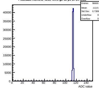
Pedestals mcm142-4215-relv1-g0-s0-p1 ch 34 test1
