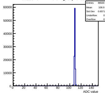
Pedestals mcm142-4215-refv1-g0-s0-p1 ch 53 test1
