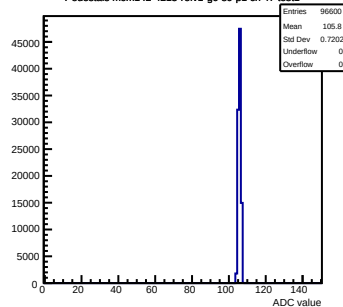
Pedestals mcm142-4215-relv1-g0-s0-p1 ch 47 test1
