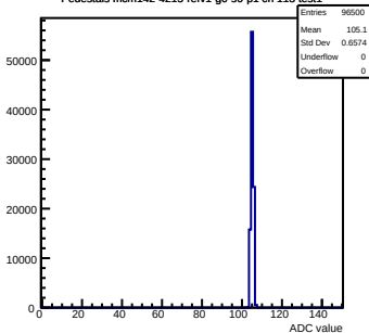
Pedestals mcm142-4215-refv1-g0-s0-p1 ch 113 test1
