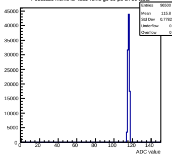
Pedestals mcm142-4215-refv1-g0-s0-p1 ch 50 test1
