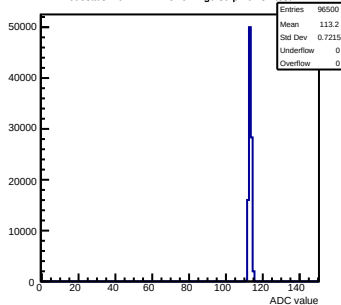
Pedestals mcm142-4215-refv1-g0-s0-p1 ch 54 test1
