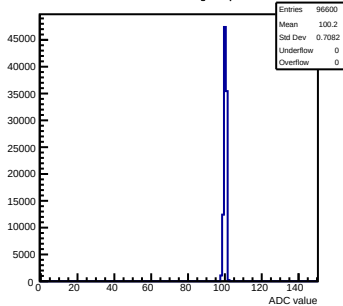
Pedestals mcm142-4215-refv1-g0-s0-p1 ch 107 test1
