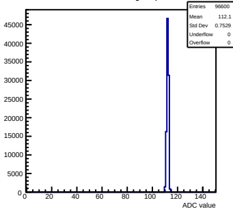
Pedestals mcm142-4215-refv1-g0-s0-p1 ch 104 test1
