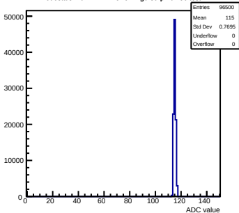
Pedestals mcm142-4215-refv1-g0-s0-p1 ch 56 test1
