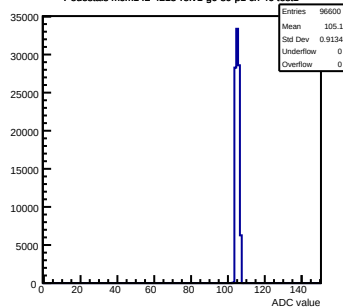
Pedestals mcm142-4215-relv1-g0-s0-p1 ch 46 test1
