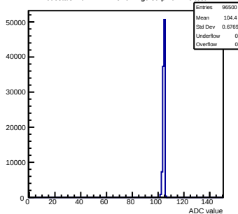
Pedestals mcm142-4215-refv1-g0-s0-p1 ch 123 test1
