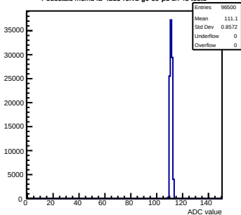
Pedestals mcm142-4215-refv1-g0-s0-p1 ch 48 test1
