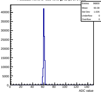
Pedestals mcm142-4215-refv3-g0-s0-p1 ch 8 test1
