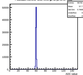
Pedestals mcm142-4215-refv3-g0-s0-p1 ch 87 test1
