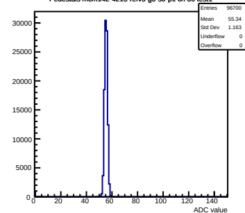
Pedestals mcm142-4215-refv3-g0-s0-p1 ch 80 test1
