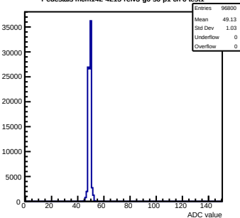
Pedestals mcm142-4215-refv3-g0-s0-p1 ch 0 test1
