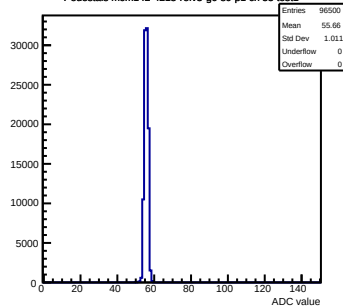
Pedestals mcm142-4215-refv3-g0-s0-p1 ch 55 test1
