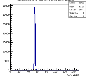
Pedestals mcm142-4215-refv3-g0-s0-p1 ch 81 test1
