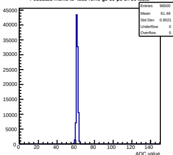
Pedestals mcm142-4215-refv3-g0-s0-p1 ch 56 test1
