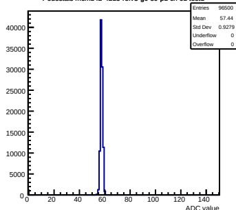
Pedestals mcm142-4215-refv3-g0-s0-p1 ch 61 test1
