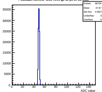
Pedestals mcm142-4215-refv3-g0-s0-p1 ch 86 test1
