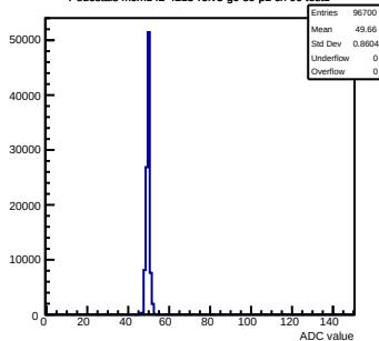
Pedestals mcm142-4215-refv3-g0-s0-p1 ch 90 test1
