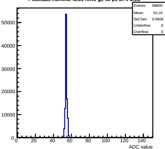
Pedestals mcm142-4215-refv3-g0-s0-p1 ch 4 test1
