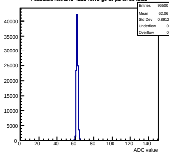
Pedestals mcm142-4215-refv3-g0-s0-p1 ch 50 test1
