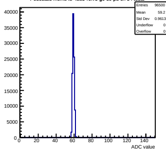
Pedestals mcm142-4215-refv3-g0-s0-p1 ch 54 test1
