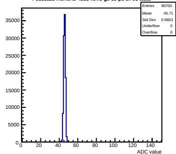
Pedestals mcm142-4215-refv3-g0-s0-p1 ch 93 test1
