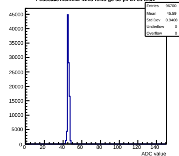
Pedestals mcm142-4215-refv3-g0-s0-p1 ch 84 test1
