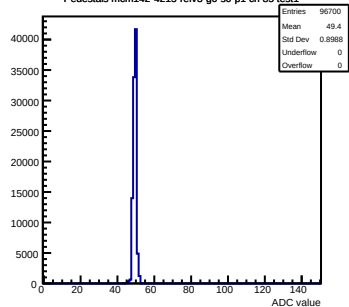
Pedestals mcm142-4215-refv3-g0-s0-p1 ch 85 test1
