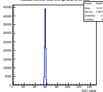
Pedestals mcm142-4215-refv3-g0-s0-p1 ch 51 test1
