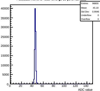
Pedestals mcm142-4215-refv3-g0-s0-p1 ch 12 test1
