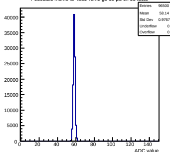
Pedestals mcm142-4215-refv3-g0-s0-p1 ch 58 test1
