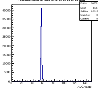
Pedestals mcm142-4215-refv3-g0-s0-p1 ch 83 test1
