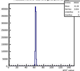
Pedestals mcm142-4215-refv3-g0-s0-p1 ch 60 test1
