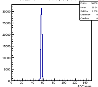
Pedestals mcm142-4215-refv3-g0-s0-p1 ch 62 test1
