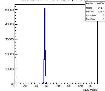
Pedestals mcm142-4215-refv3-g0-s0-p1 ch 92 test1
