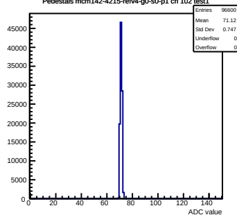
Pedestals mcm142-4215-refv4-g0-s0-p1 ch 102 test1
