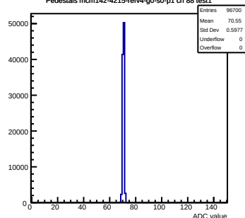
Pedestals mcm142-4215-rlv4-g0-s0-p1 ch 88 test1
