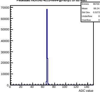
Pedestals mcm142-4215-rlv4-g0-s0-p1 ch 85 test1
