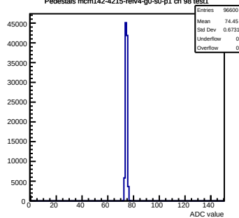
Pedestals mcm142-4215-refv4-g0-s0-p1 ch 98 test1
