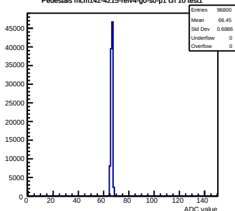
Pedestals mcm142-4215-refv4-g0-s0-p1 ch 10 test1
