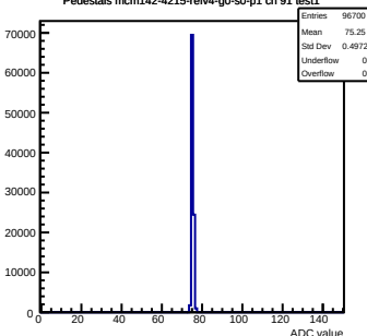
Pedestals mcm142-4215-rlv4-g0-s0-p1 ch 91 test1
