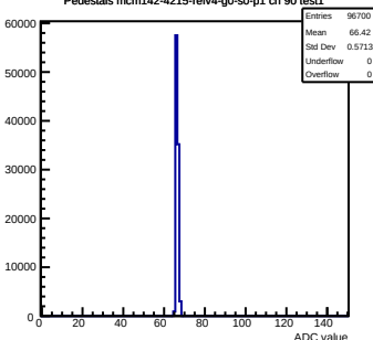
Pedestals mcm142-4215-rlv4-g0-s0-p1 ch 90 test1
