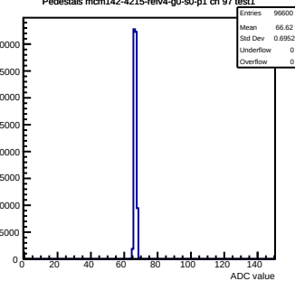
Pedestals mcm142-4215-refv4-g0-s0-p1 ch 97 test1
