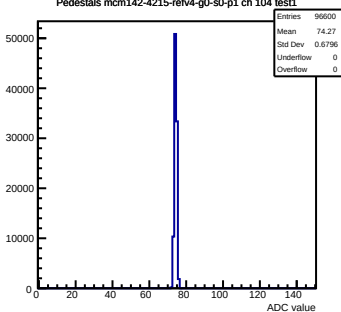
Pedestals mcm142-4215-refv4-g0-s0-p1 ch 104 test1
