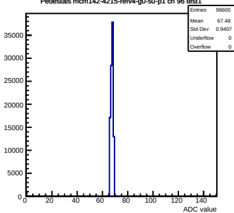
Pedestals mcm142-4215-refv4-g0-s0-p1 ch 96 test1
