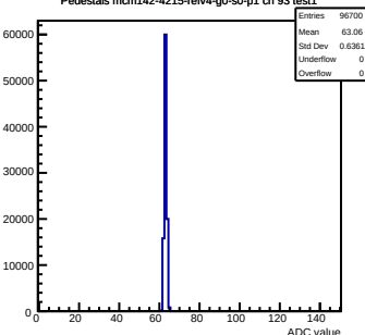
Pedestals mcm142-4215-rlv4-g0-s0-p1 ch 93 test1
