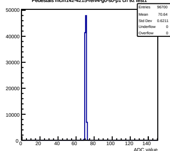
Pedestals mcm142-4215-rlv4-g0-s0-p1 ch 92 test1
