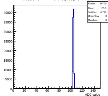
Pedestals mcm142-4215-rfv5-g0-s0-p1 ch 92 test1
