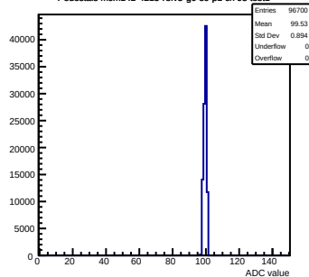
Pedestals mcm142-4215-rfv5-g0-s0-p1 ch 95 test1
