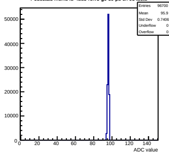
Pedestals mcm142-4215-rfv5-g0-s0-p1 ch 93 test1
