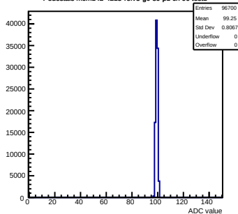
Pedestals mcm142-4215-rfv5-g0-s0-p1 ch 90 test1
