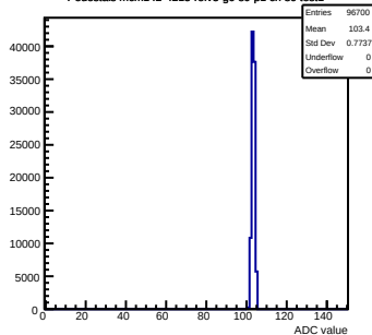
Pedestals mcm142-4215-rfv5-g0-s0-p1 ch 89 test1
