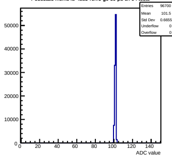
Pedestals mcm142-4215-rfv5-g0-s0-p1 ch 94 test1
