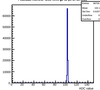
Pedestals mcm142-4215-rfv5-g0-s0-p1 ch 81 test1
