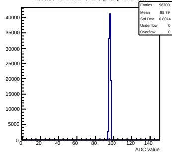
Pedestals mcm142-4215-rfv5-g0-s0-p1 ch 84 test1
