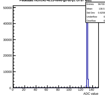
Pedestals mcm142-4215-relv6-g0-s0-p1 ch 87 test1
