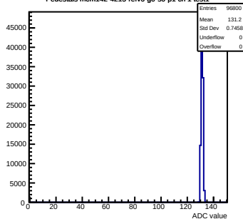
Pedestals mcm142-4215-rlv6-g0-s0-p1 ch 1 test1
