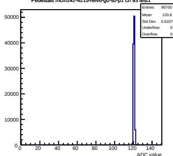
Pedestals mcm142-4215-relv6-g0-s0-p1 ch 93 test1
