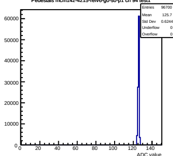
Pedestals mcm142-4215-relv6-g0-s0-p1 ch 94 test1
