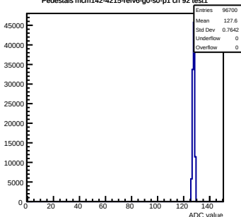
Pedestals mcm142-4215-relv6-g0-s0-p1 ch 92 test1
