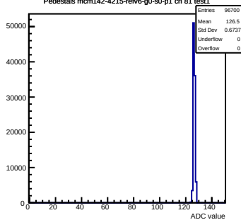
Pedestals mcm142-4215-relv6-g0-s0-p1 ch 81 test1
