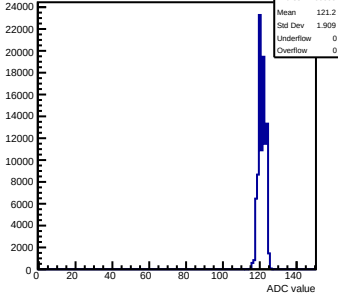
Pedestals mcm143-2C13-refV0-g0-s0-p1 ch 106 test1
