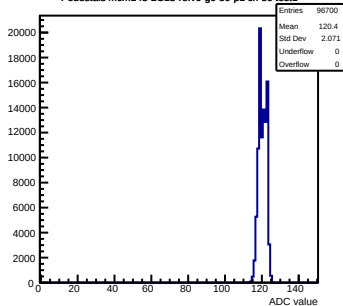
Pedestals mcm143-2C13-refV0-g0-s0-p1 ch 80 test1
