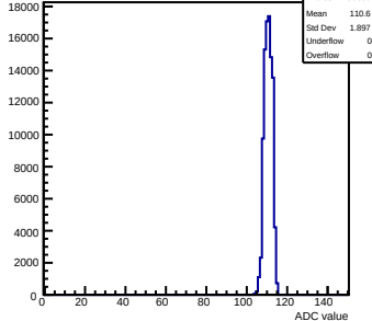
Pedestals mcm143-2C13-refV0-g0-s0-p1 ch 111 test1
