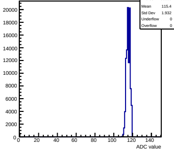
Pedestals mcm143-2C13-refV0-g0-s0-p1 ch 108 test1
