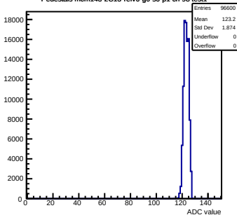
Pedestals mcm143-2C13-refV0-g0-s0-p1 ch 98 test1
