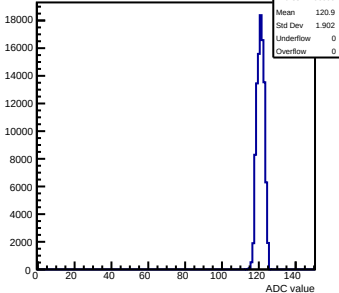
Pedestals mcm143-2C13-refV0-g0-s0-p1 ch 101 test1
