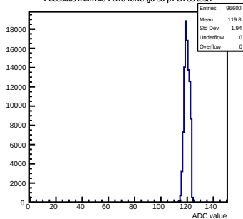
Pedestals mcm143-2C13-refV0-g0-s0-p1 ch 35 test1
