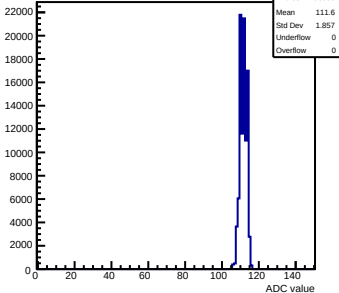
Pedestals mcm143-2C13-refV0-g0-s0-p1 ch 109 test1
