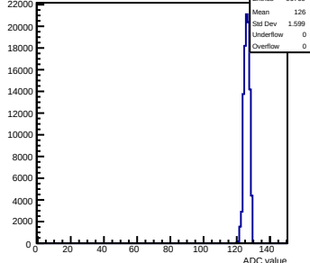
Pedestals mcm143-2C13-refV0-g0-s0-p1 ch 31 test1
