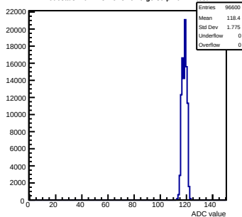
Pedestals mcm143-2C13-refV0-g0-s0-p1 ch 47 test1
