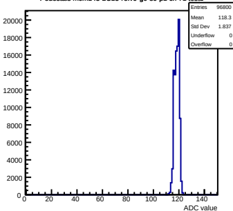
Pedestals mcm143-2C13-refV0-g0-s0-p1 ch 71 test1
