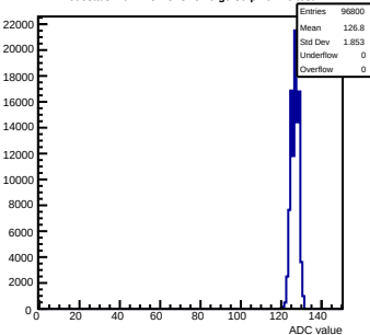
Pedestals mcm143-2C13-refV0-g0-s0-p1 ch 76 test1
