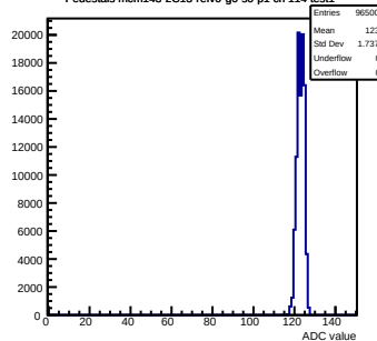
Pedestals mcm143-2C13-rev0-g0-s0-p1 ch 114 test1
