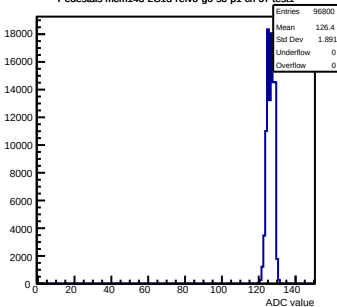
Pedestals mcm143-2C13-refV0-g0-s0-p1 ch 67 test1
