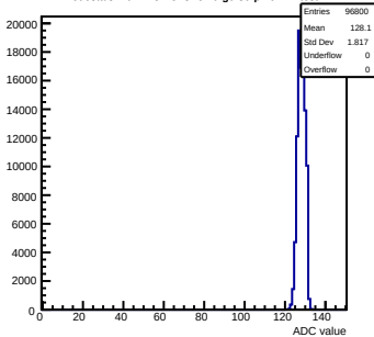
Pedestals mcm143-2C13-refV0-g0-s0-p1 ch 12 test1
