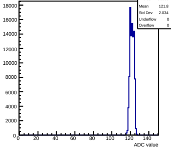
Pedestals mcm143-2C13-refV0-g0-s0-p1 ch 104 test1
