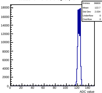
Pedestals mcm143-2C13-refV0-g0-s0-p1 ch 72 test1
