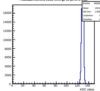
Pedestals mcm143-2C13-refV0-g0-s0-p1 ch 3 test1
