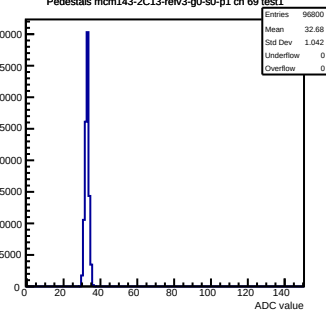
Pedestals mcm143-2C13-refV3-g0-s0-p1 ch 69 test1
