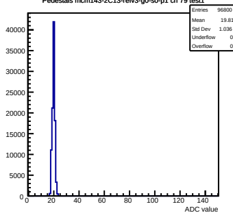
Pedestals mcm143-2C13-refV3-g0-s0-p1 ch 79 test1
