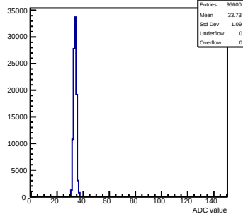
Pedestals mcm143-2C13-refV3-g0-s0-p1 ch 38 test1
