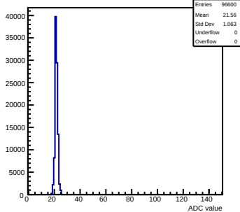
Pedestals mcm143-2C13-refV3-g0-s0-p1 ch 44 test1
