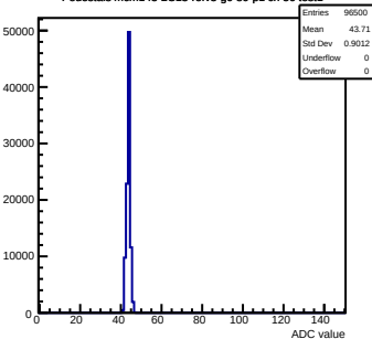
Pedestals mcm143-2C13-refV3-g0-s0-p1 ch 56 test1
