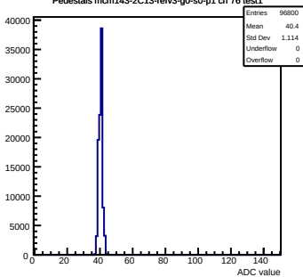
Pedestals mcm143-2C13-refV3-g0-s0-p1 ch 76 test1
