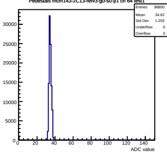
Pedestals mcm143-2C13-refV3-g0-s0-p1 ch 64 test1
