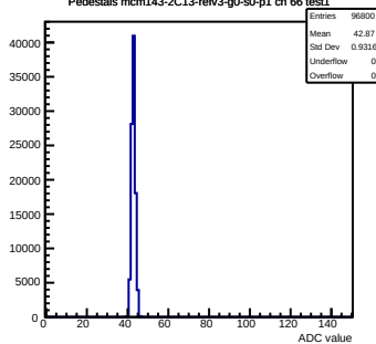
Pedestals mcm143-2C13-refV3-g0-s0-p1 ch 66 test1
