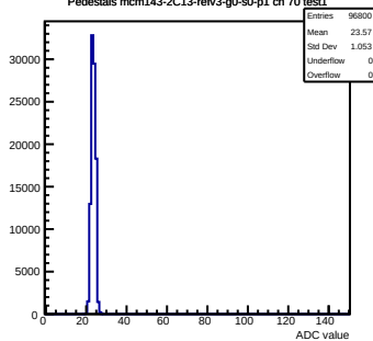
Pedestals mcm143-2C13-refV3-g0-s0-p1 ch 70 test1
