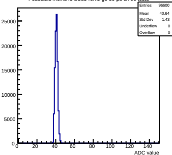
Pedestals mcm143-2C13-refV3-g0-s0-p1 ch 96 test1
