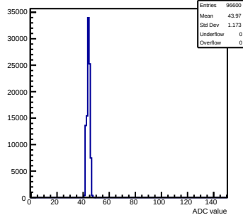
Pedestals mcm143-2C13-refV3-g0-s0-p1 ch 43 test1
