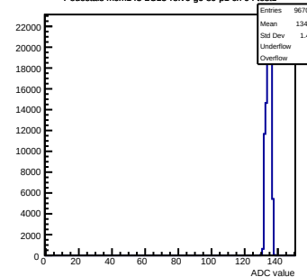
Pedestals mcm143-2C13-refv6-g0-s0-p1 ch 94 test1
