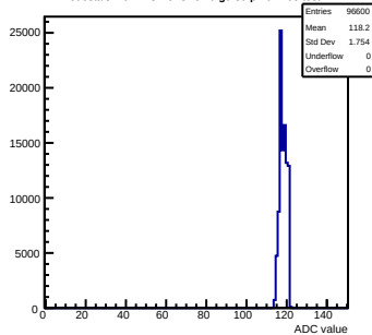
Pedestals mcm143-2C13-refV6-g0-s0-p1 ch 105 test1
