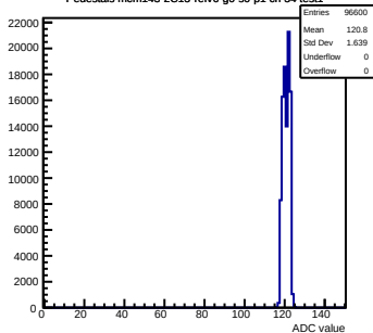
Pedestals mcm143-2C13-refV6-g0-s0-p1 ch 34 test1
