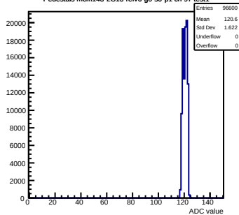
Pedestals mcm143-2C13-refV6-g0-s0-p1 ch 97 test1
