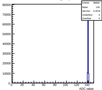
Pedestals mcm143-2C13-refV0-g0-s0-p1 ch 11 test1
