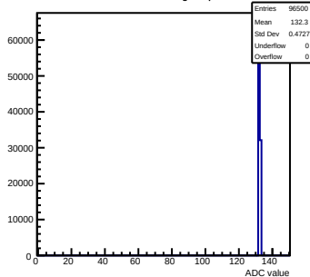
Pedestals mcm143-2C13-rev0-g0-s0-p1 ch 122 test1
