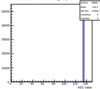
Pedestals mcm143-2C13-refV0-g0-s0-p1 ch 102 test1
