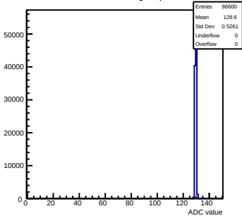
Pedestals mcm143-2C13-refV0-g0-s0-p1 ch 107 test1
