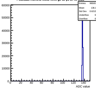
Pedestals mcm143-2C13-refV0-g0-s0-p1 ch 49 test1
