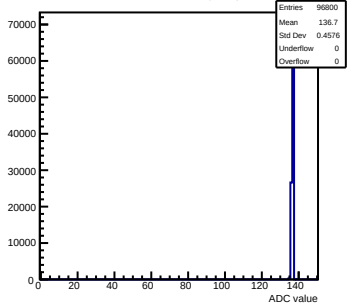
Pedestals mcm143-2C13-refV0-g0-s0-p1 ch 5 test1
