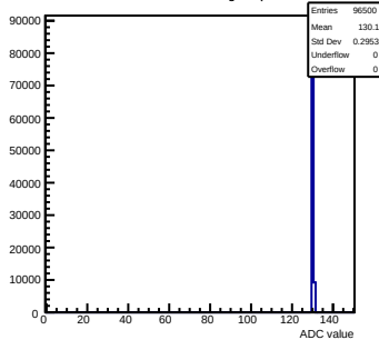
Pedestals mcm143-2C13-refV0-g0-s0-p1 ch 62 test1
