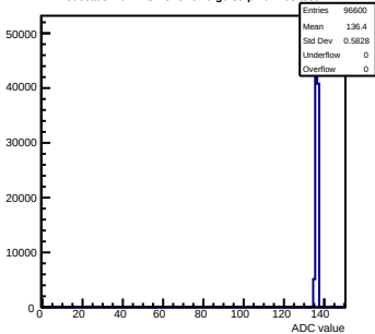
Pedestals mcm143-2C13-refV0-g0-s0-p1 ch 103 test1
