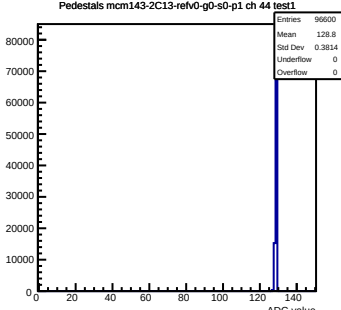
Pedestals mcm143-2C13-refV0-g0-s0-p1 ch 44 test1
