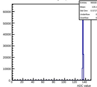
Pedestals mcm143-2C13-rev0-g0-s0-p1 ch 123 test1
