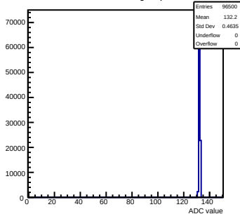
Pedestals mcm143-2C13-rev0-g0-s0-p1 ch 121 test1
