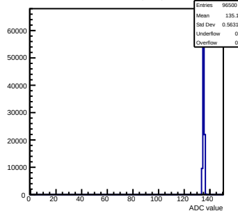
Pedestals mcm143-2C13-rev0-g0-s0-p1 ch 119 test1
