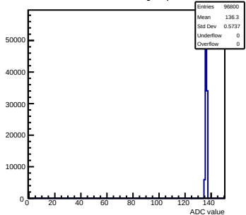
Pedestals mcm143-2C13-refV0-g0-s0-p1 ch 9 test1
