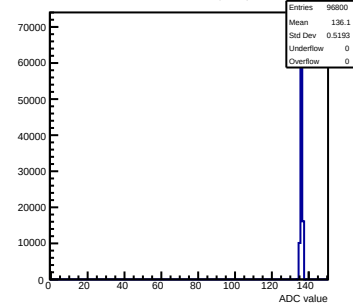
Pedestals mcm143-2C13-refV0-g0-s0-p1 ch 4 test1
