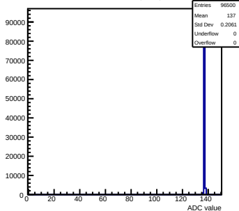
Pedestals mcm143-2C13-rev0-g0-s0-p1 ch 116 test1
