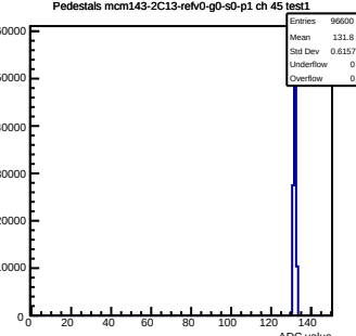
Pedestals mcm143-2C13-refV0-g0-s0-p1 ch 45 test1
