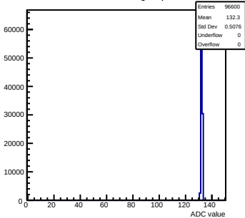
Pedestals mcm143-2C13-refV0-g0-s0-p1 ch 110 test1
