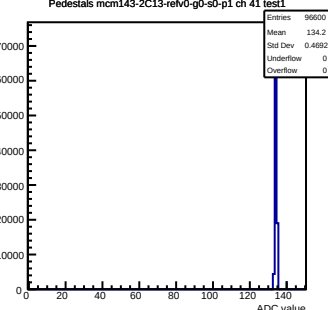
Pedestals mcm143-2C13-refV0-g0-s0-p1 ch 41 test1
