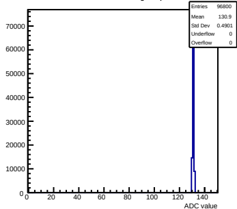
Pedestals mcm143-2C13-refV0-g0-s0-p1 ch 14 test1
