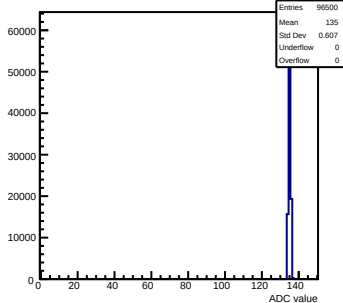
Pedestals mcm143-2C13-rev0-g0-s0-p1 ch 124 test1
