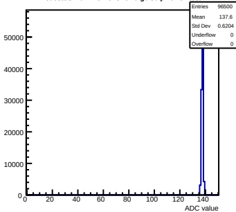
Pedestals mcm143-2C13-refV0-g0-s0-p1 ch 52 test1
