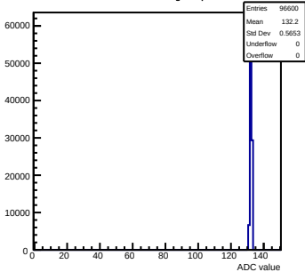
Pedestals mcm143-2C13-refV0-g0-s0-p1 ch 111 test1
