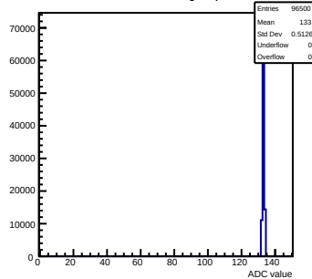
Pedestals mcm143-2C13-refV0-g0-s0-p1 ch 63 test1
