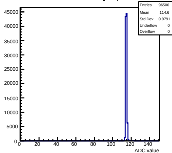
Pedestals mcm143-2C13-refv1-g0-s0-p1 ch 57 test1
