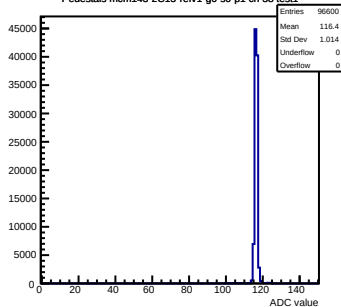
Pedestals mcm143-2C13-refv1-g0-s0-p1 ch 38 test1
