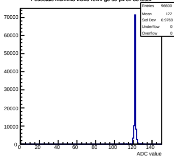
Pedestals mcm143-2C13-refv1-g0-s0-p1 ch 33 test1
