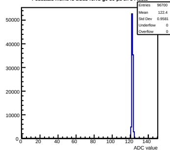
Pedestals mcm143-2C13-refv1-g0-s0-p1 ch 84 test1
