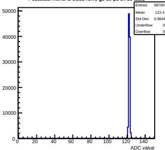
Pedestals mcm143-2C13-refv1-g0-s0-p1 ch 85 test1
