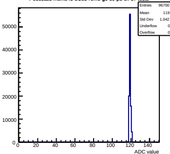
Pedestals mcm143-2C13-refv1-g0-s0-p1 ch 87 test1
