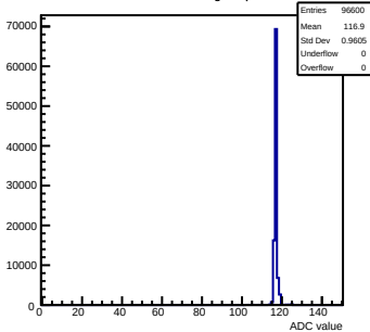
Pedestals mcm143-2C13-refV1-g0-s0-p1 ch 108 test1
