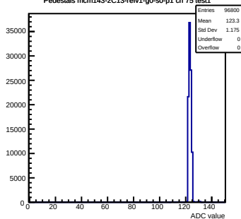
Pedestals mcm143-2C13-refv1-g0-s0-p1 ch 75 test1
