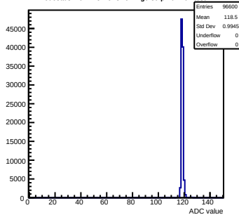
Pedestals mcm143-2C13-refV1-g0-s0-p1 ch 102 test1
