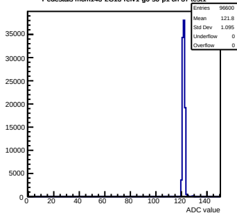
Pedestals mcm143-2C13-refv1-g0-s0-p1 ch 37 test1
