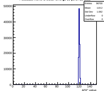
Pedestals mcm143-2C13-refv1-g0-s0-p1 ch 88 test1
