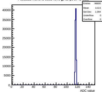
Pedestals mcm143-2C13-refv1-g0-s0-p1 ch 45 test1
