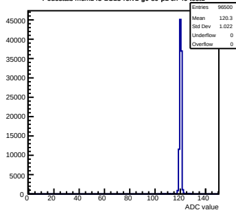
Pedestals mcm143-2C13-refv1-g0-s0-p1 ch 49 test1
