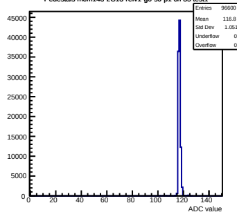
Pedestals mcm143-2C13-refv1-g0-s0-p1 ch 35 test1
