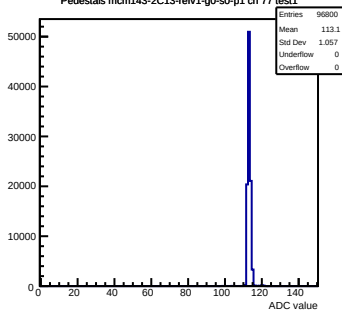
Pedestals mcm143-2C13-refv1-g0-s0-p1 ch 77 test1
