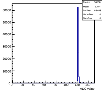
Pedestals mcm143-2C13-refv1-g0-s0-p1 ch 53 test1
