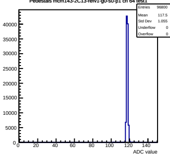
Pedestals mcm143-2C13-refv1-g0-s0-p1 ch 64 test1
