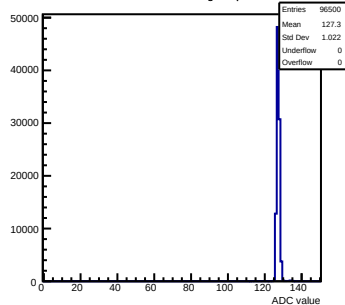
Pedestals mcm143-2C13-refv1-g0-s0-p1 ch 58 test1
