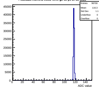
Pedestals mcm143-2C13-refv1-g0-s0-p1 ch 80 test1
