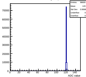
Pedestals mcm143-2C13-refV1-g0-s0-p1 ch 106 test1
