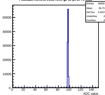
Pedestals mcm143-2C13-ref2-g0-s0-p1 ch 71 test1
