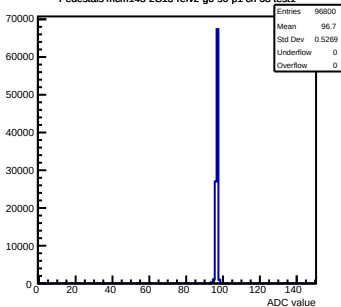
Pedestals mcm143-2C13-ref2-g0-s0-p1 ch 68 test1
