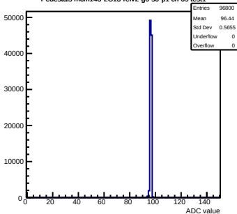
Pedestals mcm143-2C13-ref2-g0-s0-p1 ch 69 test1
