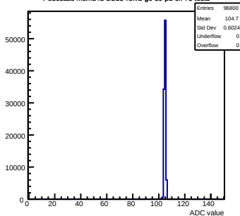
Pedestals mcm143-2C13-ref2-g0-s0-p1 ch 78 test1
