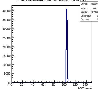
Pedestals mcm143-2C13-ref2-g0-s0-p1 ch 75 test1
