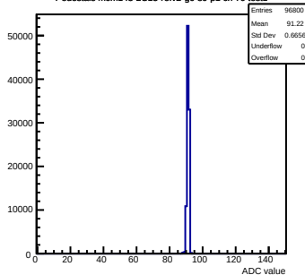
Pedestals mcm143-2C13-ref2-g0-s0-p1 ch 79 test1
