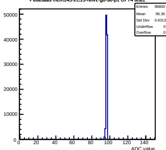
Pedestals mcm143-2C13-ref2-g0-s0-p1 ch 74 test1
