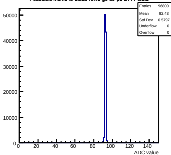
Pedestals mcm143-2C13-ref2-g0-s0-p1 ch 77 test1
