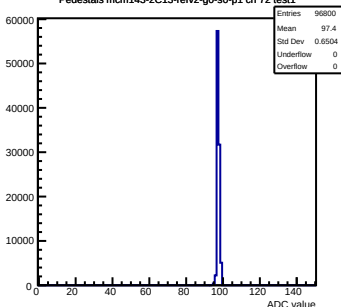
Pedestals mcm143-2C13-ref2-g0-s0-p1 ch 72 test1
