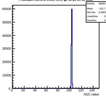
Pedestals mcm143-2C13-ref2-g0-s0-p1 ch 66 test1
