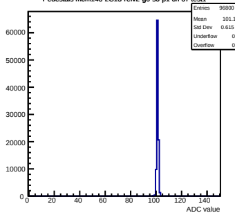
Pedestals mcm143-2C13-ref2-g0-s0-p1 ch 67 test1
