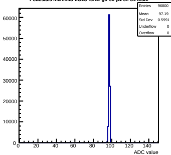
Pedestals mcm143-2C13-ref2-g0-s0-p1 ch 64 test1
