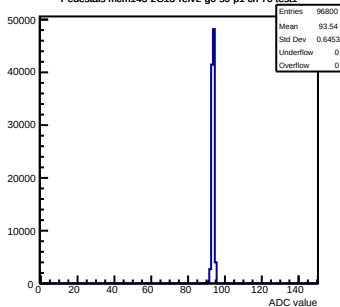
Pedestals mcm143-2C13-ref2-g0-s0-p1 ch 70 test1
