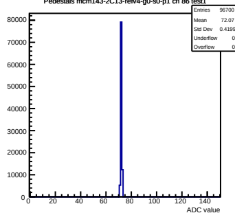
Pedestals mcm143-2C13-refV4-g0-s0-p1 ch 86 test1
