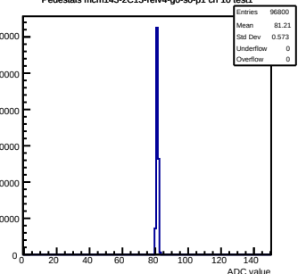
Pedestals mcm143-2C13-refV4-g0-s0-p1 ch 10 test1
