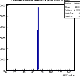
Pedestals mcm143-2C13-refv4-g0-s0-p1 ch 77 test1
