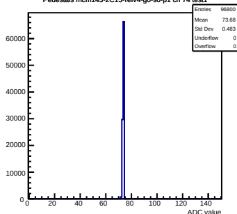
Pedestals mcm143-2C13-refv4-g0-s0-p1 ch 74 test1
