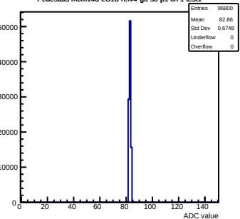
Pedestals mcm143-2C13-refV4-g0-s0-p1 ch 1 test1
