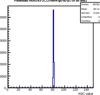
Pedestals mcm143-2C13-refV4-g0-s0-p1 ch 85 test1
