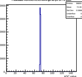
Pedestals mcm143-2C13-refv4-g0-s0-p1 ch 73 test1
