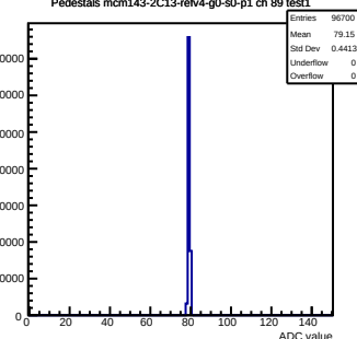
Pedestals mcm143-2C13-refV4-g0-s0-p1 ch 89 test1
