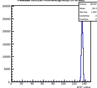
Pedestals mcm150-7A16-refV0-g0-s0-p1 ch 26 test1
