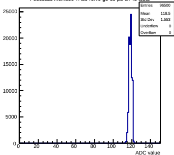
Pedestals mcm150-7A16-refV0-g0-s0-p1 ch 48 test1
