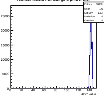
Pedestals mcm150-7A16-refV0-g0-s0-p1 ch 12 test1
