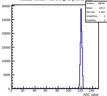
Pedestals mcm150-7A16-refV0-g0-s0-p1 ch 52 test1
