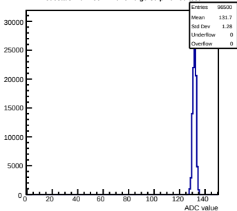
Pedestals mcm150-7A16-refV0-g0-s0-p1 ch 60 test1
