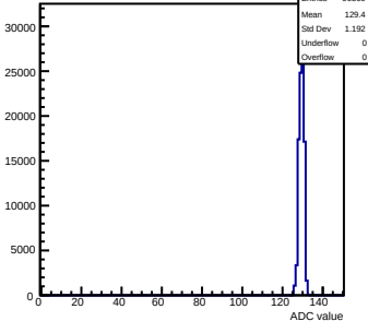
Pedestals mcm150-7A16-refV0-g0-s0-p1 ch 119 test1
