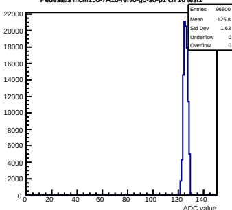
Pedestals mcm150-7A16-refV0-g0-s0-p1 ch 10 test1
