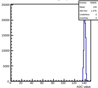
Pedestals mcm150-7A16-refV0-g0-s0-p1 ch 43 test1
