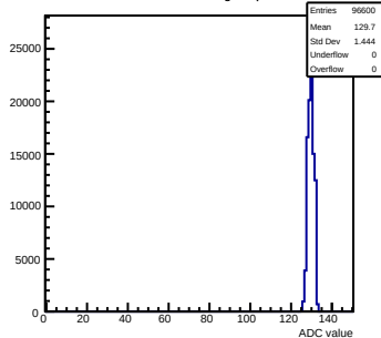
Pedestals mcm150-7A16-refV0-g0-s0-p1 ch 109 test1
