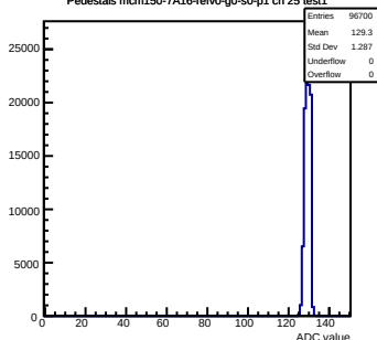
Pedestals mcm150-7A16-refV0-g0-s0-p1 ch 25 test1
