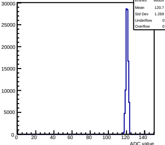
Pedestals mcm150-7A16-refV0-g0-s0-p1 ch 121 test1
