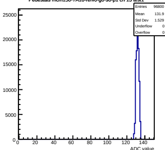
Pedestals mcm150-7A16-refV0-g0-s0-p1 ch 13 test1
